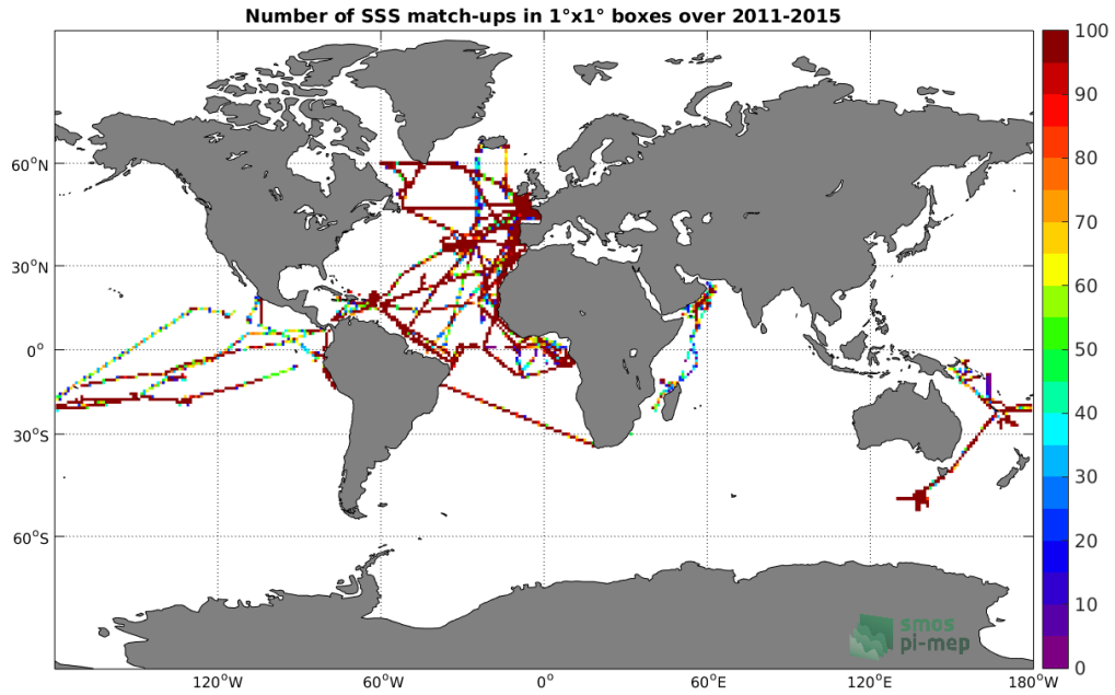
Figure 4: Number of SSS match-ups between TSG-GOSUD-Research-vessel SSS and the Aquarius-L4-IPRC-V5-WEEKLY SSS product for the Global Ocean Pi-MEP region over 1°x1° boxes and for the full satellite product period.
