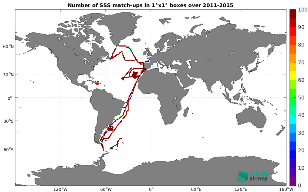
Figure 4: Number of SSS match-ups between TSG (CSIC-UTM) SSS and the Aquarius SSS L4 OI v5 - Weekly (IPRC) SSS product for the Global Ocean Pi-MEP region over 1^\circ \times 1^\circ boxes and for the full satellite product period.
