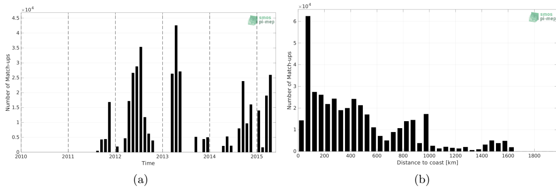
Figure 1: Number of match-ups between TSG (CSIC-UTM) and Aquarius SSS L4 OI v5 - Weekly (IPRC) SSS as a function of time (a) and as function of the distance to coast (b) over the Global Ocean Pi-MEP region and for the full satellite product period.
