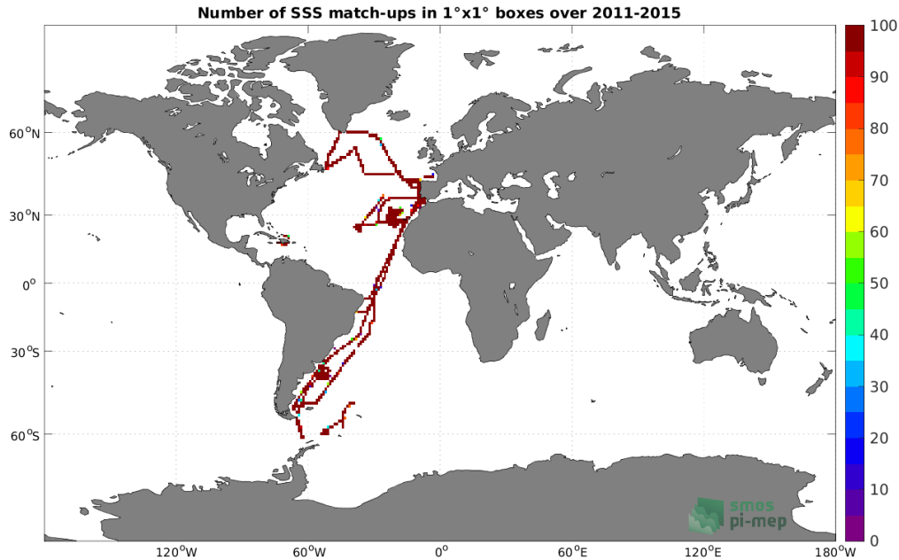
Figure 4: Number of SSS match-ups between TSG (CSIC-UTM) SSS and the Aquarius SSS L4 OI v5 - Weekly (IPRC) SSS product for the Global Ocean Pi-MEP region over 1°x1° boxes and for the full satellite product period.
