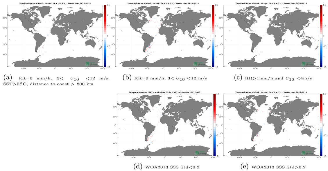
Figure 12: Temporal mean gridded over spatial boxes of size 1^\circ \times 1^\circ of \Delta SSS (Aquarius SSS L4 OI v5 - Weekly (IPRC) - TSG (CSIC-UTM)) for 5 different subdatasets corresponding to:RR=0 mm/h, 3 < U_{10} < 12 m/s, SST > 5^\circ\text{C} , distance to coast > 800 km (a), RR=0 mm/h, 3 < U_{10} < 12 m/s (b), RR > 1 mm/h and U_{10} < 4 m/s (c), WOA2013 SSS Std < 0.2 (d), WOA2013 SSS Std > 0.2 (e).
