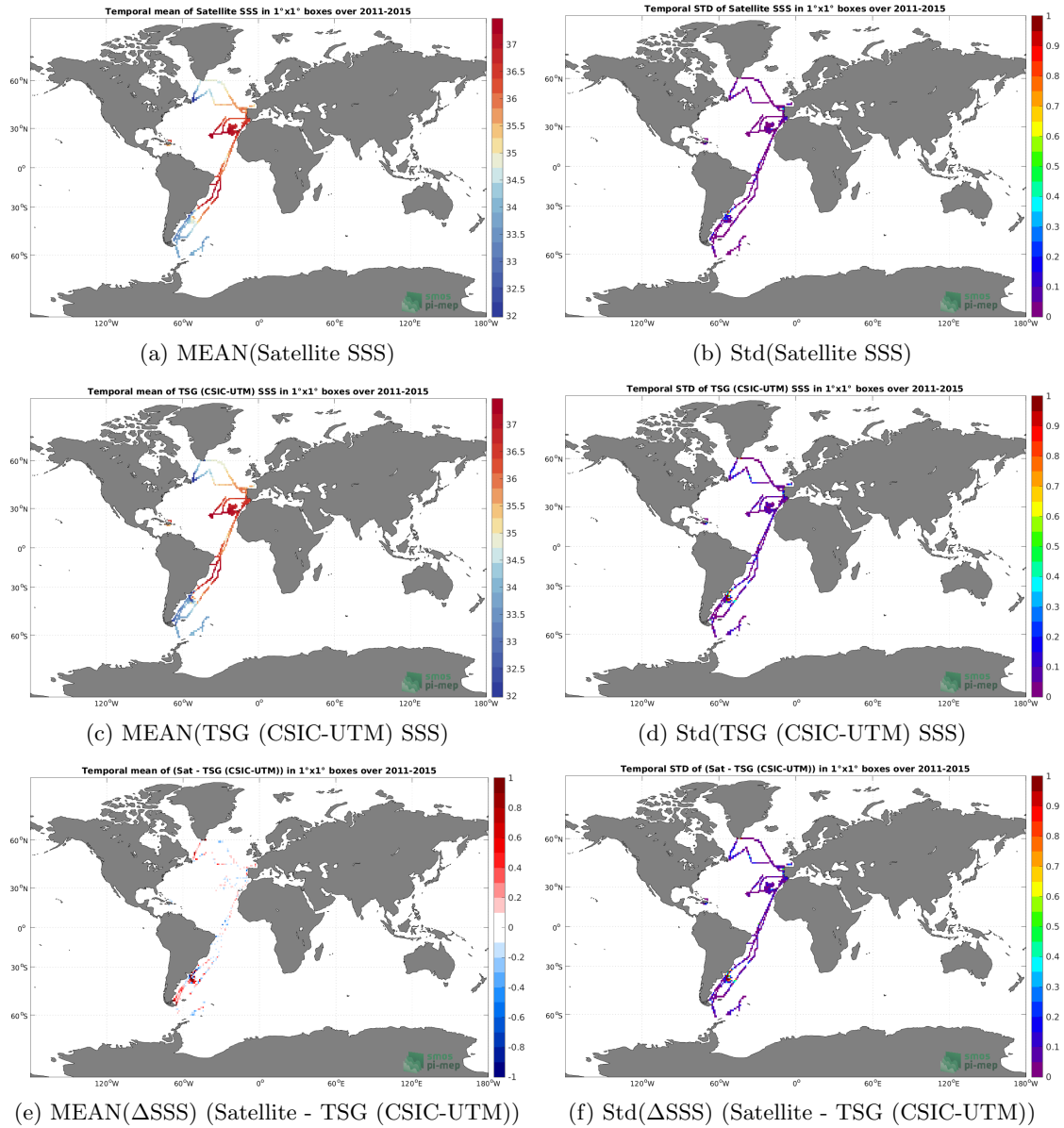
Figure 6: Temporal mean (left) and Std (right) of SSS from Aquarius SSS L4 OI v5 - Weekly (IPRC) (top), TSG (CSIC-UTM) (middle), and of \Delta SSS (Satellite - TSG (CSIC-UTM)). Only match-up pairs are used to generate these maps.
