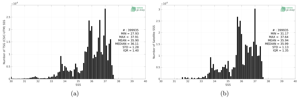
Figure 2: Histograms of SSS from TSG (CSIC-UTM) (a) and Aquarius SSS L4 OI v5 - Weekly (IPRC) (b) considering all match-up pairs per bins of 0.1 over the Global Ocean Pi-MEP region and for the full satellite product period.
