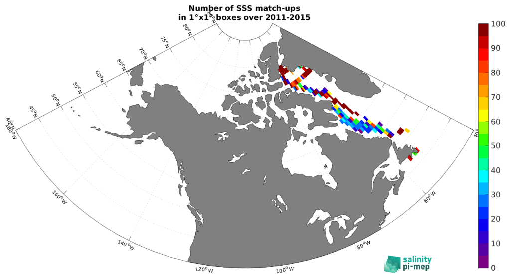
Figure 5: Number of SSS match-ups between TSG (Amundsen) SSS and the Aquarius SSS L4 OI v5 - Weekly (IPRC) SSS product for the Global Ocean Pi-MEP region over 1°×1° boxes and for the full satellite product period.
