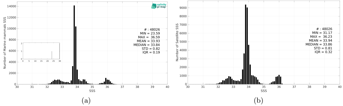
Figure 3: Histograms of SSS from Marine mammals (a) and Aquarius SSS L4 OI v5 - Weekly (IPRC) (b) considering all match-up pairs per bins of 0.1 over the Global Ocean Pi-MEP region and for the full satellite product period.
