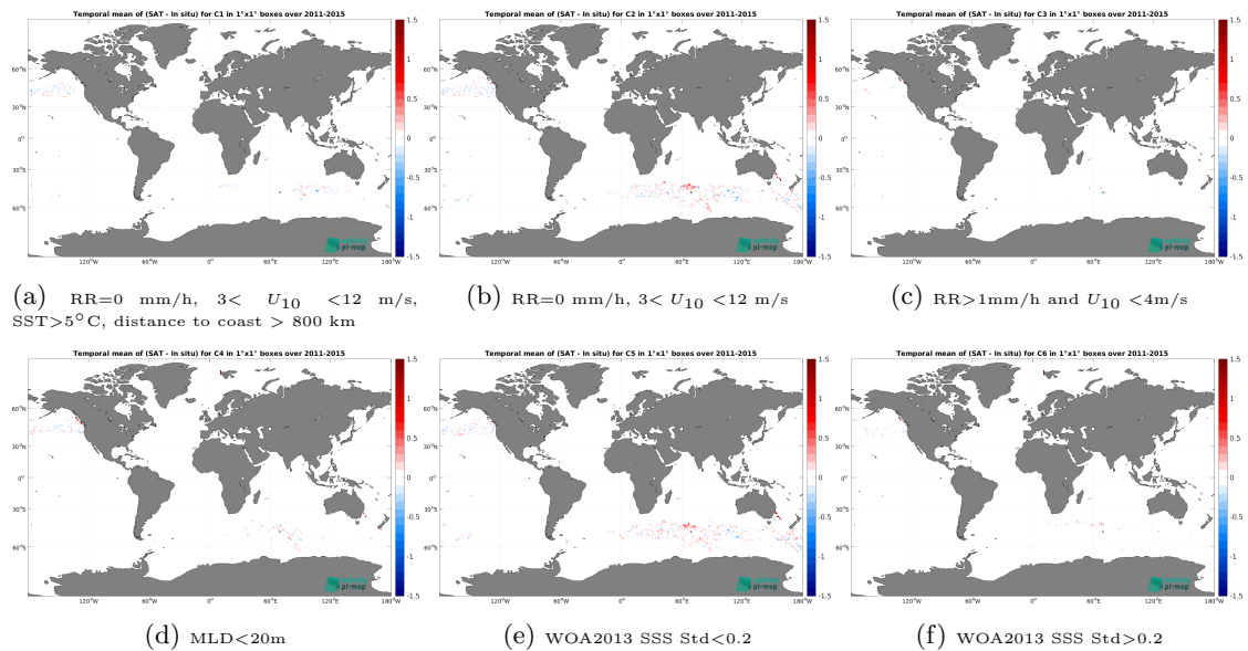
Figure 14: Temporal mean gridded over spatial boxes of size 1^\circ \times 1^\circ of \Delta SSS (Aquarius SSS L4 OI v5 - Weekly (IPRC) - Marine mammals) for 6 different subdatasets corresponding to: RR=0 mm/h, 3 < U_{10} < 12 m/s, SST > 5°C, distance to coast > 800 km (a), RR=0 mm/h, 3 < U_{10} < 12 m/s (b), RR > 1mm/h and U_{10} < 4 m/s (c), MLD < 20m (d), WOA2013 SSS Std < 0.2 (e), WOA2013 SSS Std > 0.2 (f).
