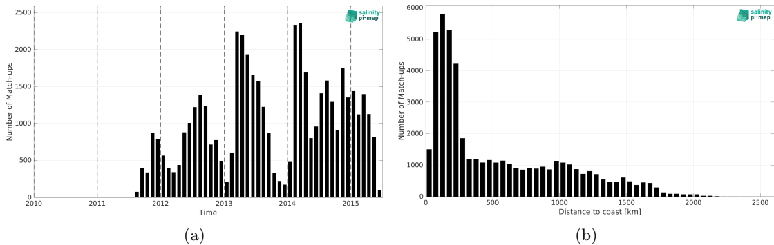
Figure 2: Number of match-ups between Marine mammals and Aquarius SSS L4 OI v5 - Weekly (IPRC) SSS as a function of time (a) and as function of the distance to coast (b) over the Global Ocean Pi-MEP region and for the full satellite product period.
