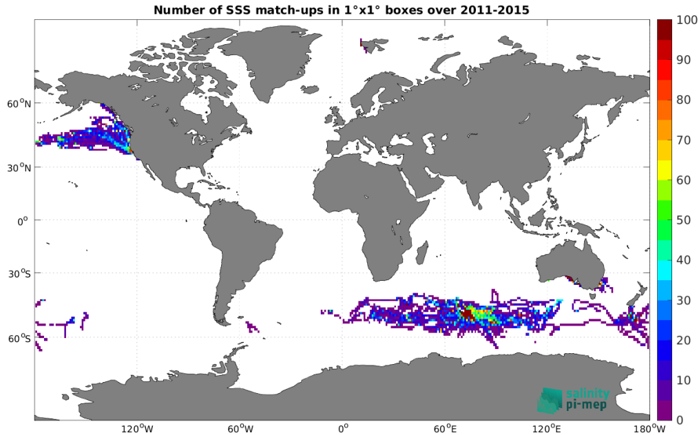
Figure 5: Number of SSS match-ups between Marine mammals SSS and the Aquarius SSS L4 OI v5 - Weekly (IPRC) SSS product for the Global Ocean Pi-MEP region over 1^\circ \times 1^\circ boxes and for the full satellite product period.
