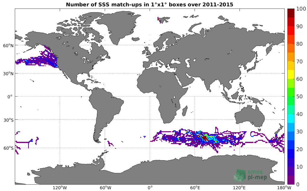
Figure 4: Number of SSS match-ups between Sea mammals SSS and the Aquarius SSS L4 OI v5 - Weekly (IPRC) SSS product for the Global Ocean Pi-MEP region over 1^\circ \times 1^\circ boxes and for the full satellite product period.
