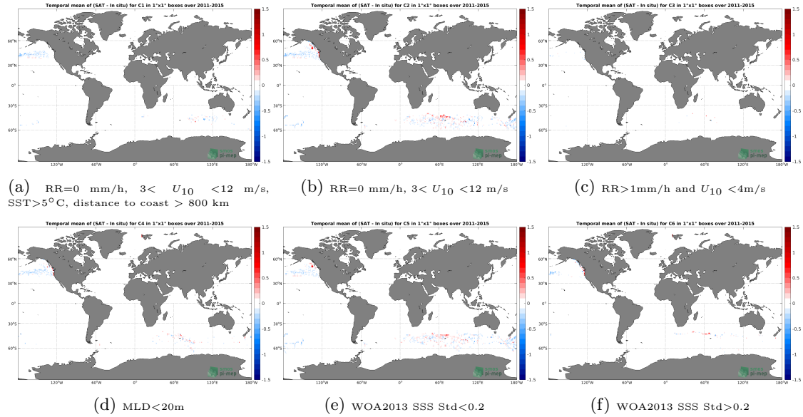
Figure 12: Temporal mean gridded over spatial boxes of size 1^\circ \times 1^\circ of \Delta SSS (Aquarius SSS L4 OI v5 - Weekly (IPRC) - Sea mammals) for 6 different subdatasets corresponding to: RR=0 mm/h, 3 < U_{10} < 12 m/s, SST >5^\circ\text{C} , distance to coast > 800 km (a), RR=0 mm/h, 3 < U_{10} < 12 m/s (b), RR >1 mm/h and U_{10} < 4 m/s (c), MLD <20 m (d), WOA2013 SSS Std <0.2 (e), WOA2013 SSS Std >0.2 (f).
