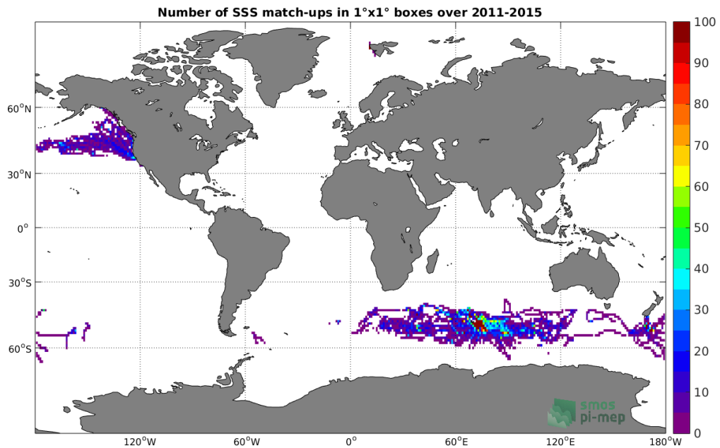
Figure 4: Number of SSS match-ups between Sea mammals SSS and the Aquarius-L4-IPRC-V5-WEEKLY SSS product for the Global Ocean Pi-MEP region over 1°x1° boxes and for the full satellite product period.
