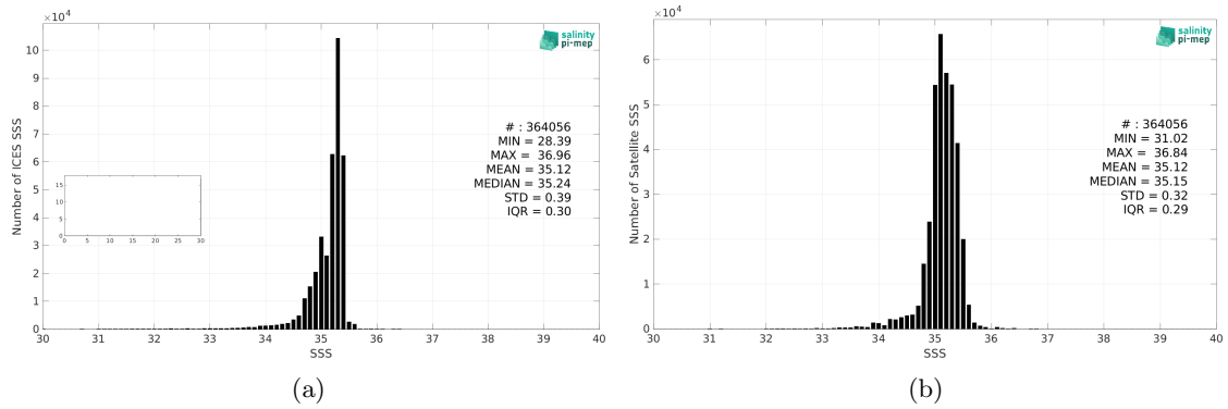
Figure 2: Histograms of SSS from ICES (a) and Aquarius SSS L4 OI v5 - Weekly (IPRC) (b) considering all match-up pairs per bins of 0.1 over the Global Ocean Pi-MEP region and for the full satellite product period.
