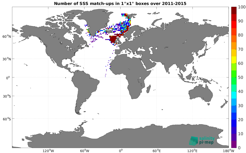
Figure 4: Number of SSS match-ups between ICES SSS and the Aquarius SSS L4 OI v5 - Weekly (IPRC) SSS product for the Global Ocean Pi-MEP region over 1^\circ \times 1^\circ boxes and for the full satellite product period.
