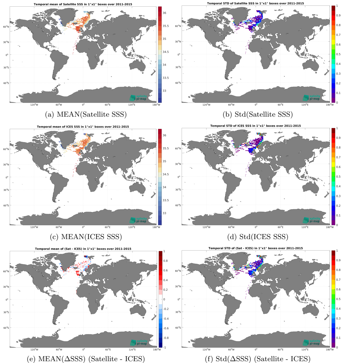
Figure 6: Temporal mean (left) and Std (right) of SSS from Aquarius SSS L4 OI v5 - Weekly (IPRC) (top), ICES (middle), and of \Delta SSS (Satellite - ICES). Only match-up pairs are used to generate these maps.
