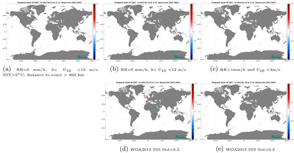
Figure 12: Temporal mean gridded over spatial boxes of size 1^\circ \times 1^\circ of \Delta SSS (Aquarius SSS L4 OI v5 - Weekly (IPRC) - ICES) for 5 different subdatasets corresponding to:RR=0 mm/h, 3 < U_{10} < 12 m/s, SST > 5^\circ\text{C} , distance to coast > 800 km (a), RR=0 mm/h, 3 < U_{10} < 12 m/s (b), RR > 1 mm/h and U_{10} < 4 m/s (c), WOA2013 SSS Std < 0.2 (d), WOA2013 SSS Std > 0.2 (e).
