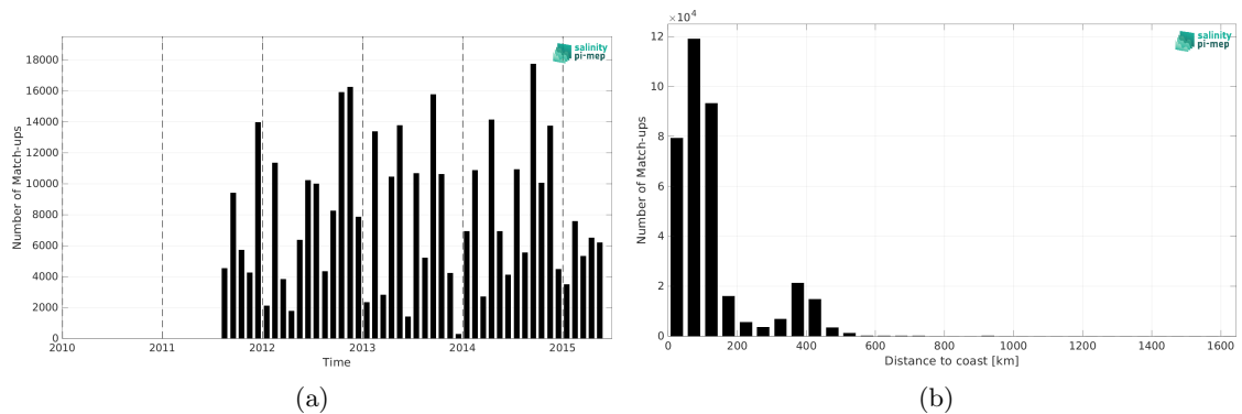
Figure 1: Number of match-ups between ICES and Aquarius SSS L4 OI v5 - Weekly (IPRC) SSS as a function of time (a) and as function of the distance to coast (b) over the Global Ocean Pi-MEP region and for the full satellite product period.
