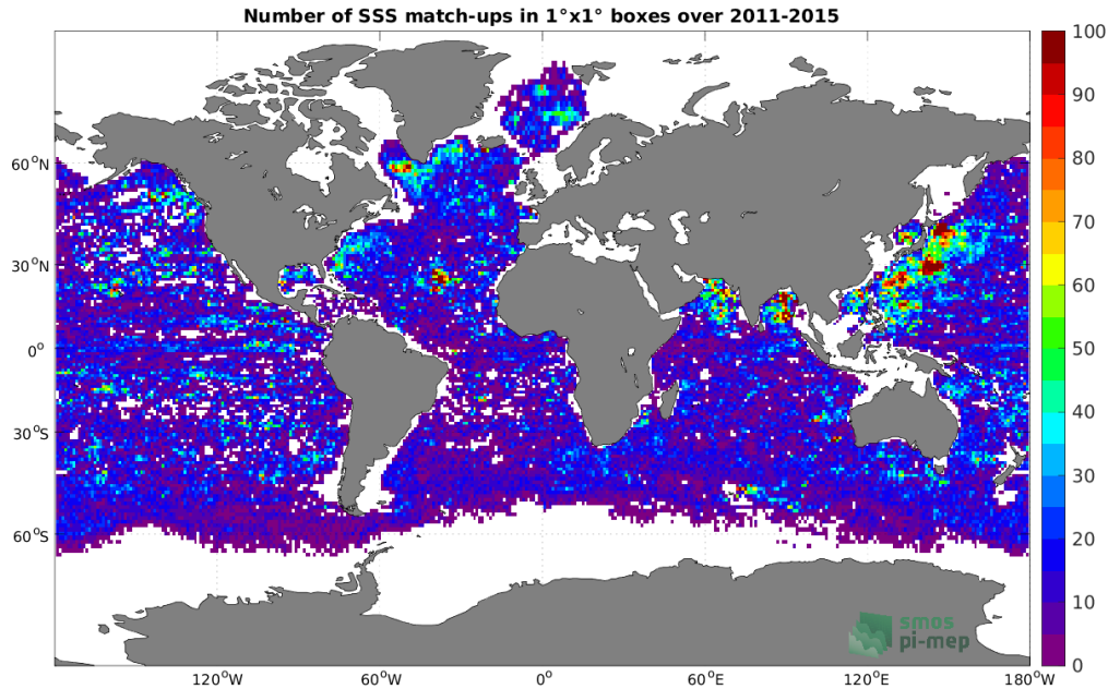
Figure 4: Number of SSS match-ups between Argo SSS and the Aquarius SSS L4 OI v5 - Weekly (IPRC) SSS product for the Global Ocean Pi-MEP region over 1^\circ \times 1^\circ boxes and for the full satellite product period.
