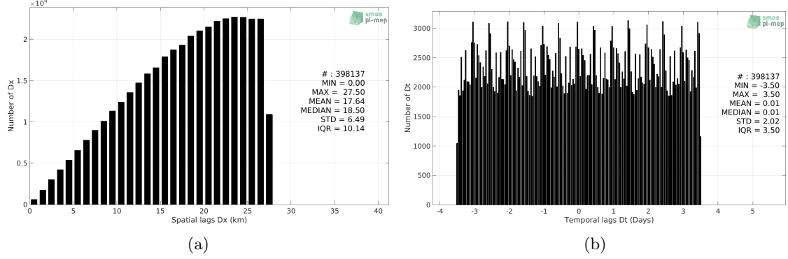
Figure 5: Histograms of the spatial (a) and temporal (b) lags between the time of the Argo measurements and the date of the corresponding Aquarius SSS L4 OI v5 - Weekly (IPRC) SSS product.
