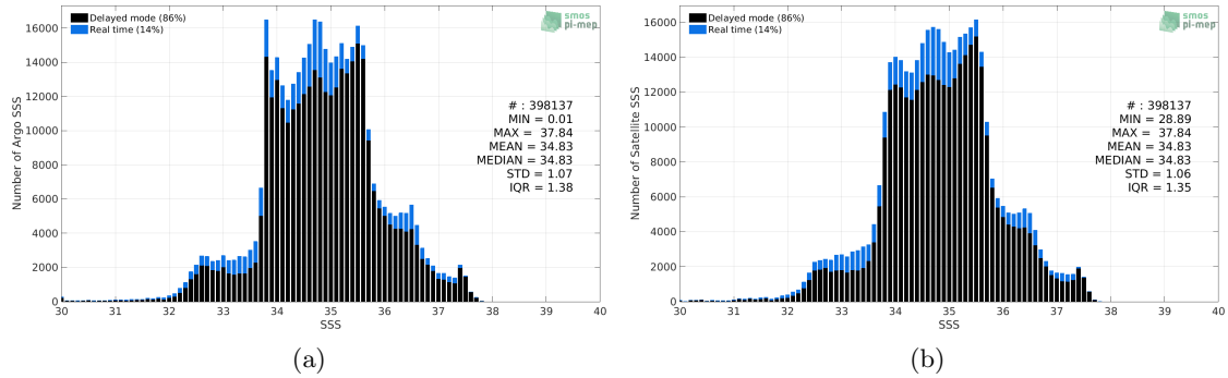
Figure 2: Histograms of SSS from Argo (a) and Aquarius SSS L4 OI v5 - Weekly (IPRC) (b) considering all match-up pairs per bins of 0.1 over the Global Ocean Pi-MEP region and for the full satellite product period.
