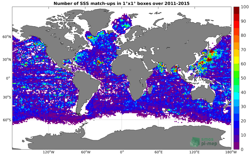
Figure 4: Number of SSS match-ups between Argos SSS and the Aquarius SSS L4 OI v5 - Weekly (IPRC) SSS product for the Global Ocean Pi-MEP region over 1^\circ \times 1^\circ boxes and for the full satellite product period.
