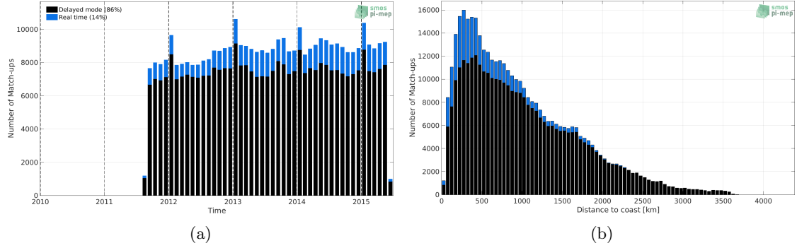
Figure 1: Number of match-ups between Argo and Aquarius SSS L4 OI v5 - Weekly (IPRC) SSS as a function of time (a) and as function of the distance to coast (b) over the Global Ocean Pi-MEP region and for the full satellite product period.
