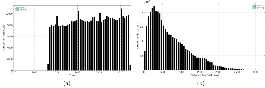
Figure 1: Number of match-ups between Argo and Aquarius-L4-IPRC-V5-WEEKLY SSS as a function of time (a) and as function of the distance to coast (b) over the Global Ocean Pi-MEP region and for the full satellite product period.
