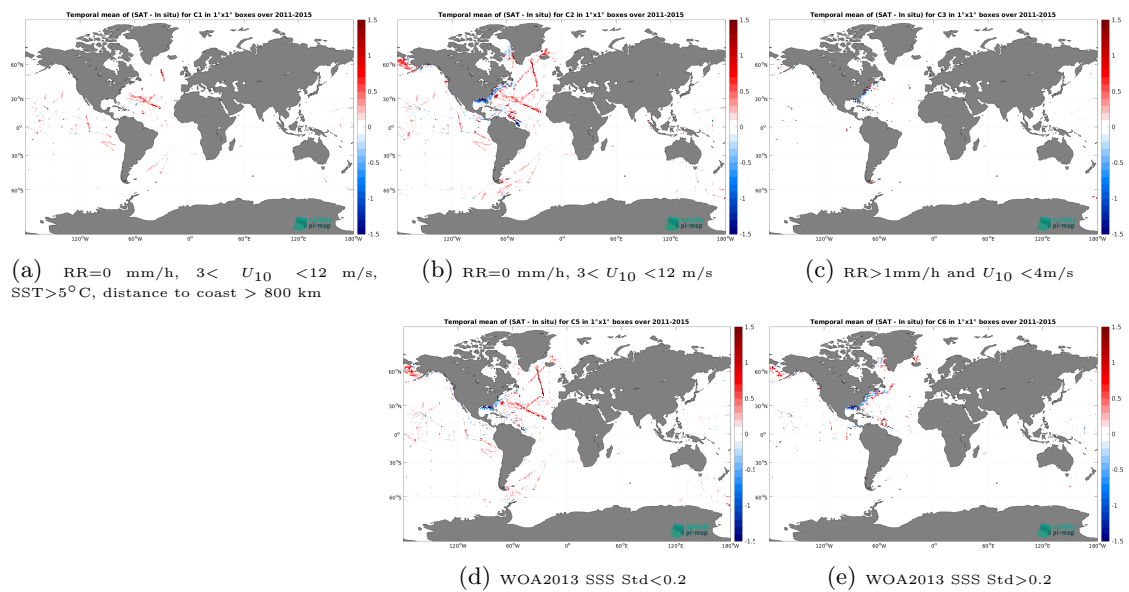
Figure 14: Temporal mean gridded over spatial boxes of size 1^\circ \times 1^\circ of \Delta SSS (Aquarius SSS L4 OI v5 - Monthly (IPRC) - TSG (SAMOS)) for 5 different subdatasets corresponding to: RR=0 mm/h, 3 < U_{10} < 12 m/s, SST > 5°C, distance to coast > 800 km (a), RR=0 mm/h, 3 < U_{10} < 12 m/s (b), RR > 1mm/h and U_{10} < 4 m/s (c), WOA2013 SSS Std < 0.2 (d), WOA2013 SSS Std > 0.2 (e).
