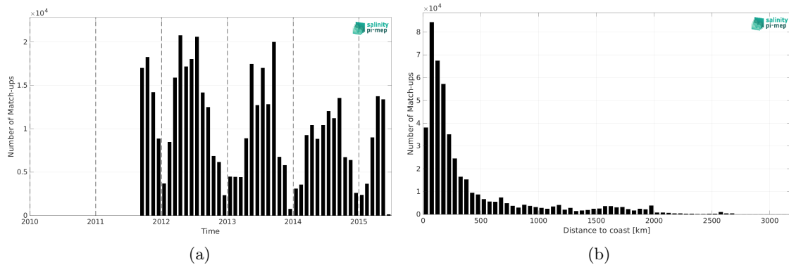
Figure 2: Number of match-ups between TSG (SAMOS) and Aquarius SSS L4 OI v5 - Monthly (IPRC) SSS as a function of time (a) and as function of the distance to coast (b) over the Global Ocean Pi-MEP region and for the full satellite product period.
