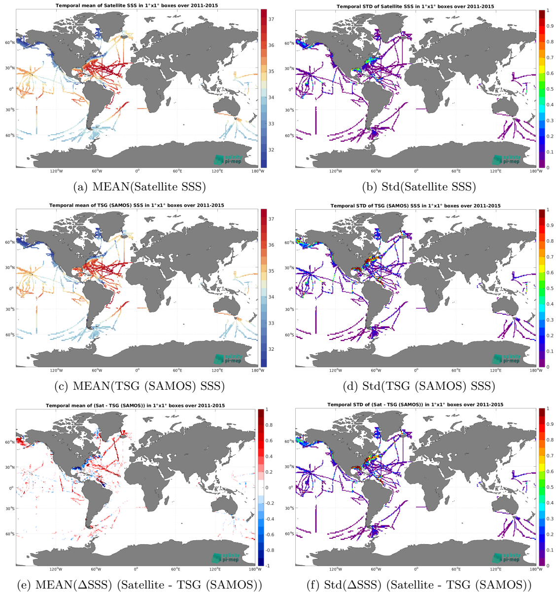
Figure 7: Temporal mean (left) and Std (right) of SSS from Aquarius SSS L4 OI v5 - Monthly (IPRC) (top), TSG (SAMOS) (middle), and of \Delta SSS (Satellite - TSG (SAMOS)). Only match-up pairs are used to generate these maps.
