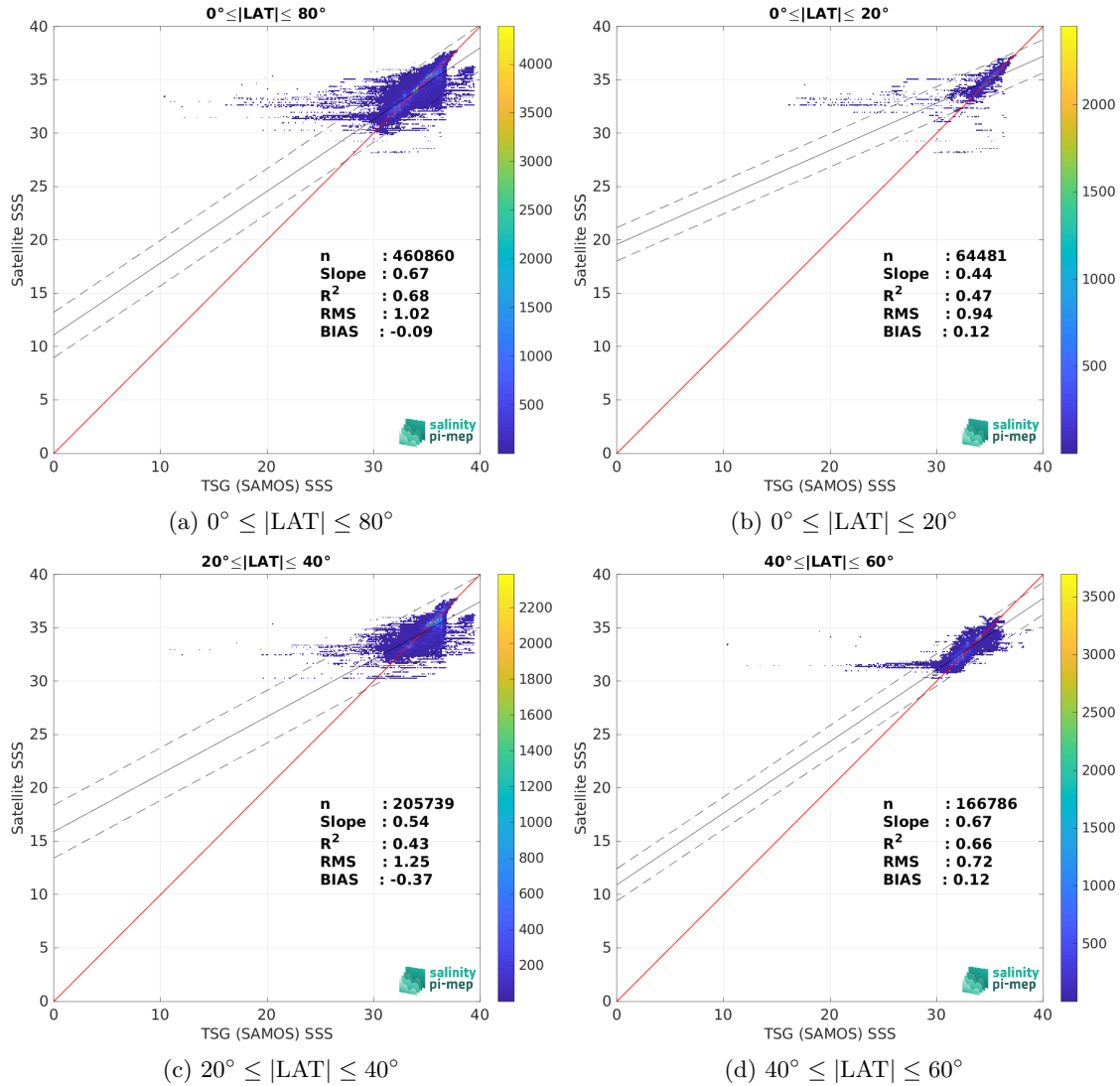
Figure 10: Contour maps of the concentration of Aquarius SSS L4 OI v5 - Monthly (IPRC) SSS (y-axis) versus TSG (SAMOS) SSS (x-axis) at match-up pairs for different latitude bands. For each plot, the red line shows x=y . The black thin and dashed lines indicate a linear fit through the data cloud and the \pm 95\% confidence levels, respectively. The number match-up pairs n , the slope and R^2 coefficient of the linear fit, the root mean square (RMS) and the mean bias between satellite and in situ data are indicated for each latitude band in each plots.
