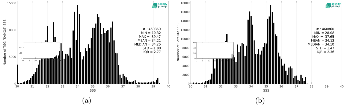
Figure 3: Histograms of SSS from TSG (SAMOS) (a) and Aquarius SSS L4 OI v5 - Monthly (IPRC) (b) considering all match-up pairs per bins of 0.1 over the Global Ocean Pi-MEP region and for the full satellite product period.
