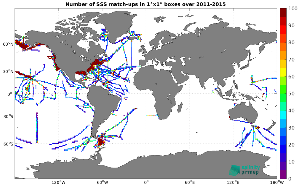
Figure 5: Number of SSS match-ups between TSG (SAMOS) SSS and the Aquarius SSS L4 OI v5 - Monthly (IPRC) SSS product for the Global Ocean Pi-MEP region over 1^\circ \times 1^\circ boxes and for the full satellite product period.
