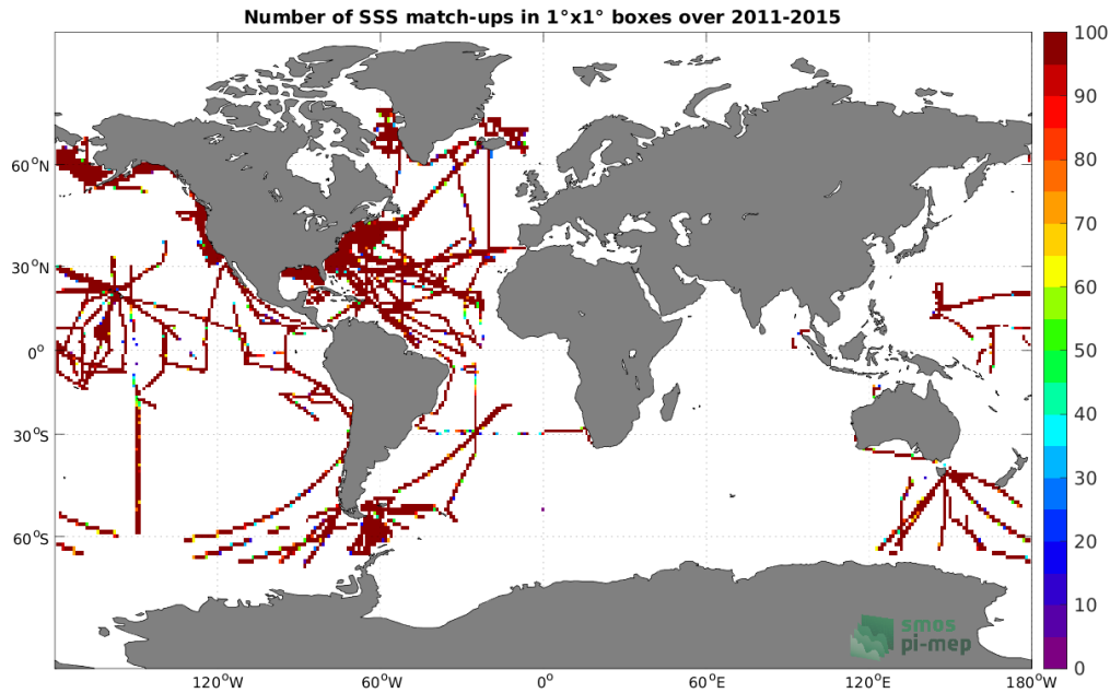
Figure 4: Number of SSS match-ups between TSG (SAMOS) SSS and the Aquarius SSS L4 OI v5 - Monthly (IPRC) SSS product for the Global Ocean Pi-MEP region over 1^\circ \times 1^\circ boxes and for the full satellite product period.
