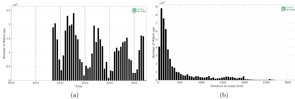
Figure 1: Number of match-ups between TSG (SAMOS) and Aquarius SSS L4 OI v5 - Monthly (IPRC) SSS as a function of time (a) and as function of the distance to coast (b) over the Global Ocean Pi-MEP region and for the full satellite product period.
