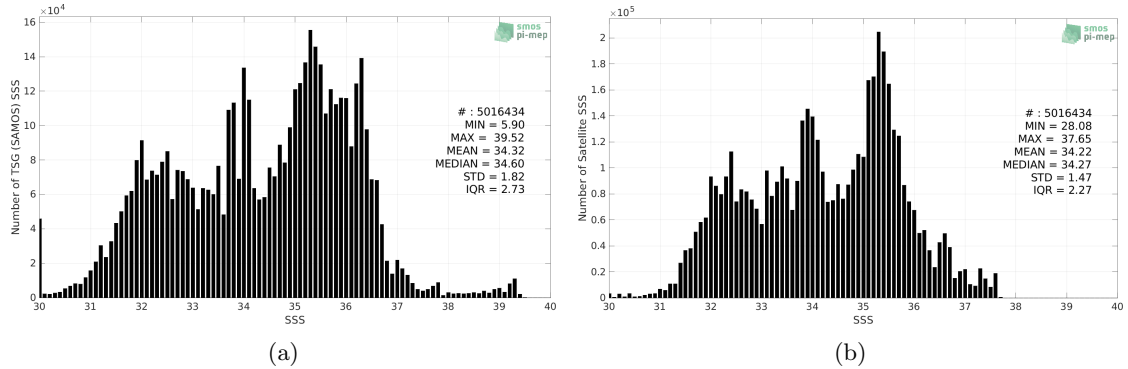
Figure 2: Histograms of SSS from TSG (SAMOS) (a) and Aquarius SSS L4 OI v5 - Monthly (IPRC) (b) considering all match-up pairs per bins of 0.1 over the Global Ocean Pi-MEP region and for the full satellite product period.
