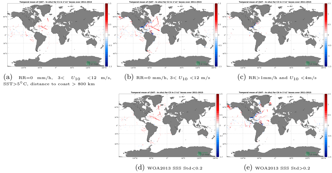
Figure 12: Temporal mean gridded over spatial boxes of size 1^\circ \times 1^\circ of \Delta SSS (Aquarius-L4-IPRC-V5-MONTHLY - TSG-SAMOS) for 5 different subdatasets corresponding to:RR=0 mm/h, 3 < U_{10} < 12 m/s, SST >5^\circ C, distance to coast > 800 km (a), RR=0 mm/h, 3 < U_{10} < 12 m/s (b), RR >1 mm/h and U_{10} < 4 m/s (c), WOA2013 SSS Std <0.2 (d), WOA2013 SSS Std >0.2 (e).
