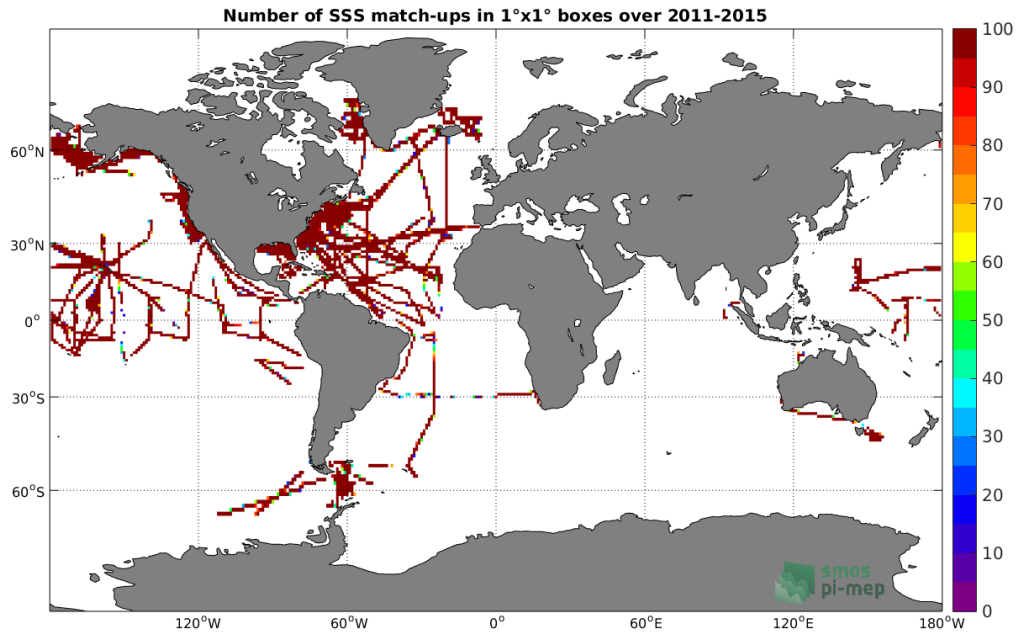
Figure 4: Number of SSS match-ups between TSG-SAMOS SSS and the Aquarius-L4-IPRC-V5-MONTHLY SSS product for the Global Ocean Pi-MEP region over 1°x1° boxes and for the full satellite product period.
