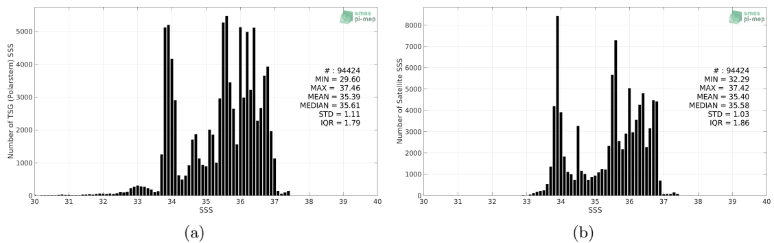
Figure 2: Histograms of SSS from TSG (Polarstern) (a) and Aquarius SSS L4 OI v5 - Monthly (IPRC) (b) considering all match-up pairs per bins of 0.1 over the Global Ocean Pi-MEP region and for the full satellite product period.
