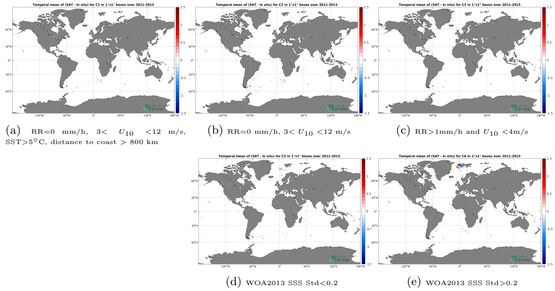
Figure 12: Temporal mean gridded over spatial boxes of size 1^\circ \times 1^\circ of \Delta SSS (Aquarius SSS L4 OI v5 - Monthly (IPRC) - TSG (Polarstern)) for 5 different subdatasets corresponding to: RR=0 mm/h, 3 < U_{10} < 12 m/s, SST > 5^\circ C , distance to coast > 800 km (a), RR=0 mm/h, 3 < U_{10} < 12 m/s (b), RR > 1 mm/h and U_{10} < 4 m/s (c), WOA2013 SSS Std < 0.2 (d), WOA2013 SSS Std > 0.2 (e).
