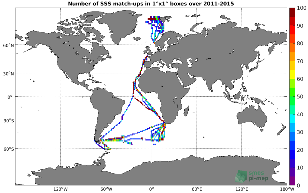
Figure 4: Number of SSS match-ups between TSG (Polarstern) SSS and the Aquarius SSS L4 OI v5 - Monthly (IPRC) SSS product for the Global Ocean Pi-MEP region over 1^\circ \times 1^\circ boxes and for the full satellite product period.
