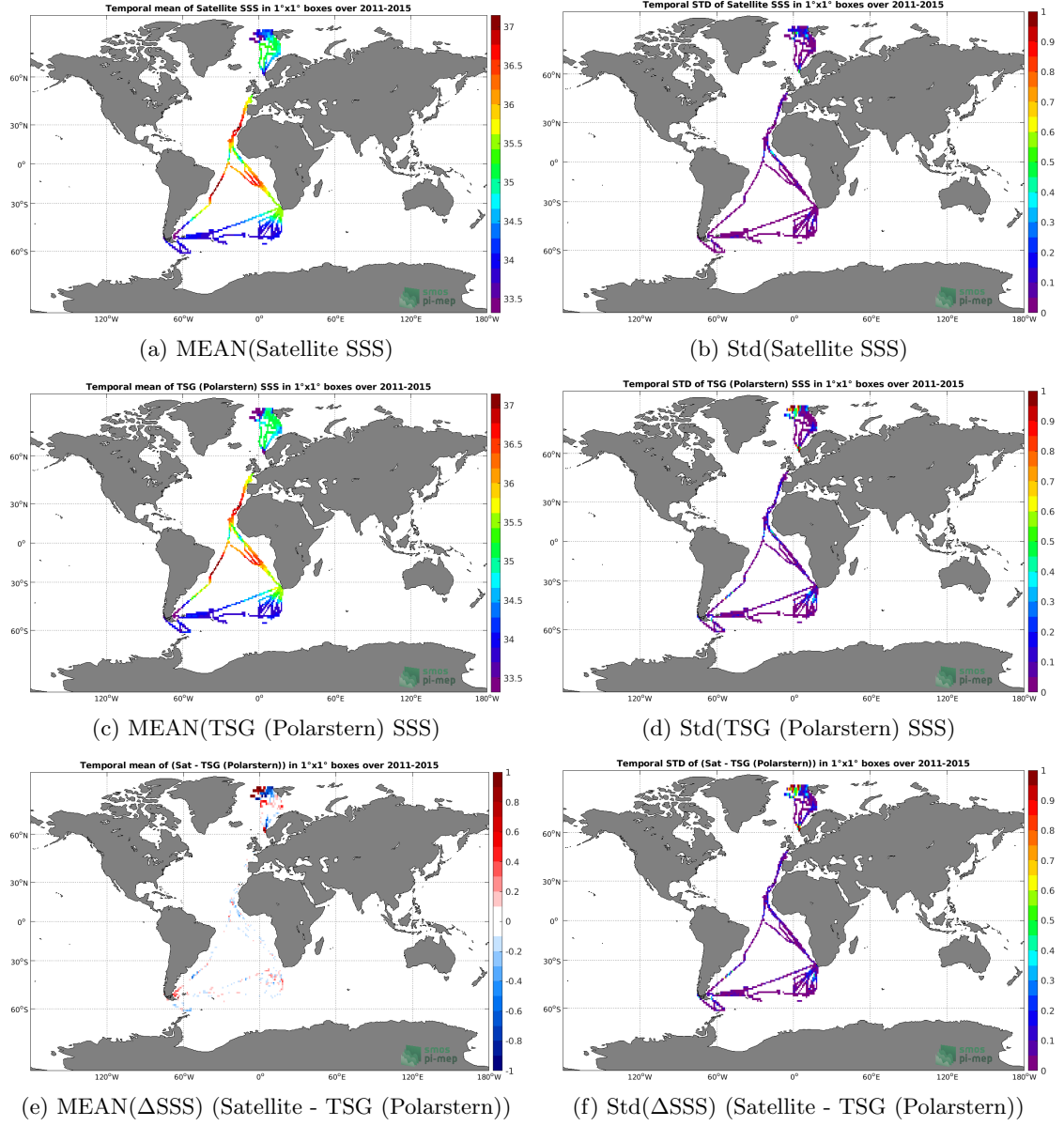
Figure 6: Temporal mean (left) and Std (right) of SSS from Aquarius SSS L4 OI v5 - Monthly (IPRC) (top), TSG (Polarstern) (middle), and of \Delta SSS (Satellite - TSG (Polarstern)). Only match-up pairs are used to generate these maps.
