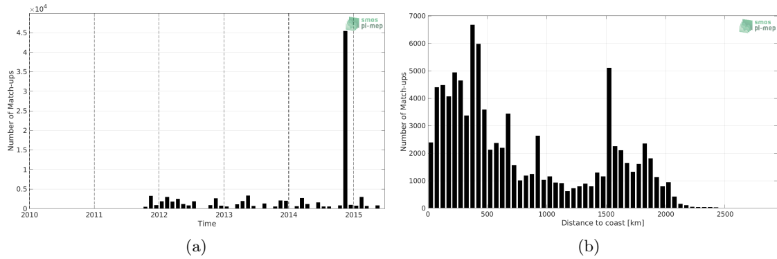
Figure 1: Number of match-ups between TSG (Polarstern) and Aquarius SSS L4 OI v5 - Monthly (IPRC) SSS as a function of time (a) and as function of the distance to coast (b) over the Global Ocean Pi-MEP region and for the full satellite product period.
