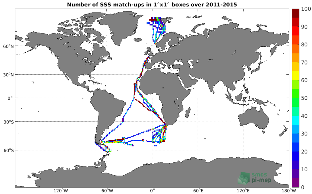
Figure 4: Number of SSS match-ups between TSG (Polarstern) SSS and the Aquarius SSS L4 OI v5 - Monthly (IPRC) SSS product for the Global Ocean Pi-MEP region over 1^\circ \times 1^\circ boxes and for the full satellite product period.
