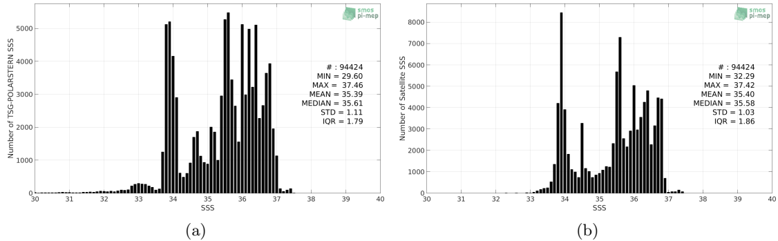
Figure 2: Histograms of SSS from TSG-POLARSTERN (a) and Aquarius-L4-IPRC-V5-MONTHLY (b) considering all match-up pairs per bins of 0.1 over the Global Ocean Pi-MEP region and for the full satellite product period.
