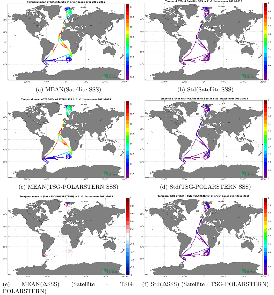
Figure 6: Temporal mean (left) and Std (right) of SSS from Aquarius-L4-IPRC-V5-MONTHLY (top), TSG-POLARSTERN (middle), and of \Delta SSS (Satellite - TSG-POLARSTERN). Only match-up pairs are used to generate these maps.
