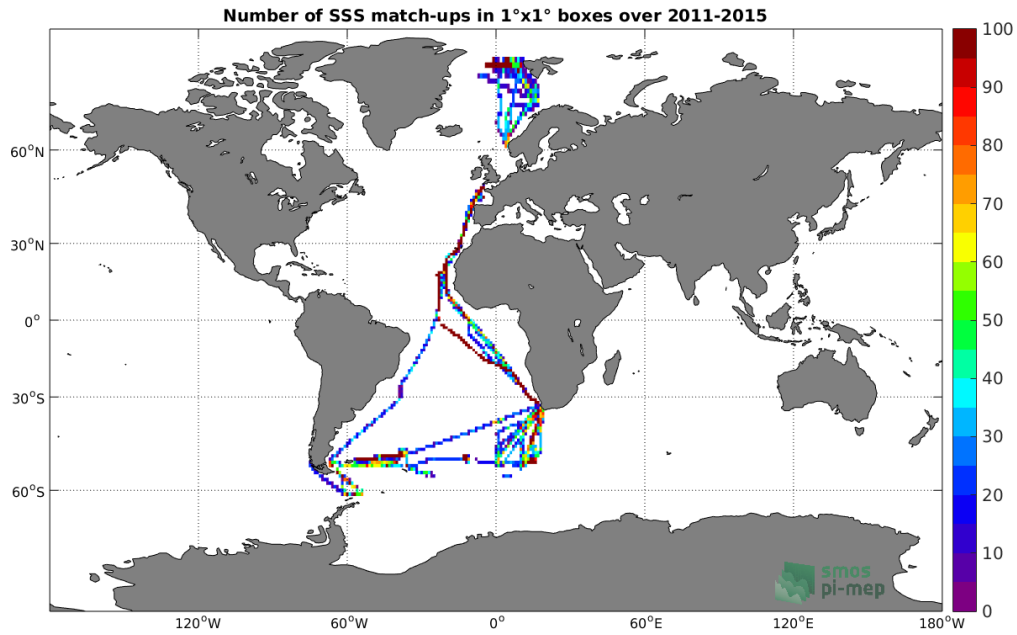
Figure 4: Number of SSS match-ups between TSG-POLARSTERN SSS and the Aquarius-L4-IPRC-V5-MONTHLY SSS product for the Global Ocean Pi-MEP region over 1^\circ \times 1^\circ boxes and for the full satellite product period.
