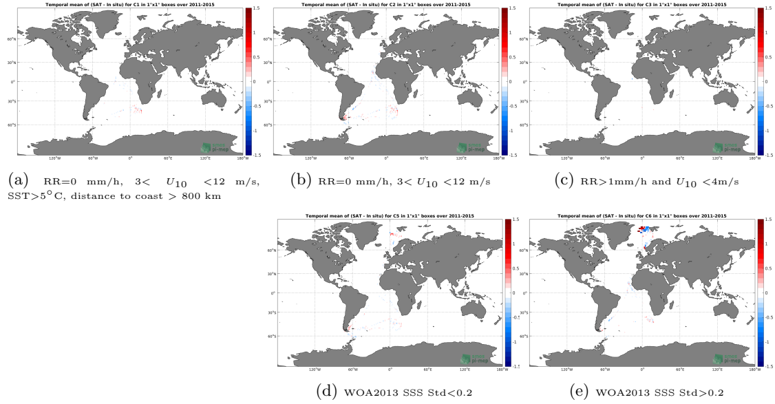
Figure 12: Temporal mean gridded over spatial boxes of size 1^\circ \times 1^\circ of \Delta SSS (Aquarius-L4-IPRC-V5-MONTHLY - TSG-POLARSTERN) for 5 different subdatasets corresponding to: RR=0 mm/h, 3 < U_{10} < 12 m/s, SST >5^\circ C, distance to coast > 800 km (a), RR=0 mm/h, 3 < U_{10} < 12 m/s (b), RR >1 mm/h and U_{10} < 4 m/s (c), WOA2013 SSS Std <0.2 (d), WOA2013 SSS Std >0.2 (e).
