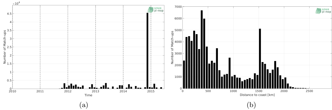
Figure 1: Number of match-ups between TSG-POLARSTERN and Aquarius-L4-IPRC-V5-MONTHLY SSS as a function of time (a) and as function of the distance to coast (b) over the Global Ocean Pi-MEP region and for the full satellite product period.
