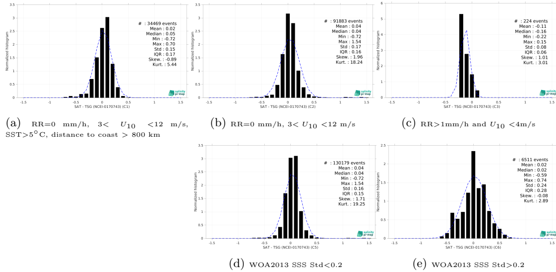
Figure 15: Normalized histogram of \Delta SSS (Aquarius SSS L4 OI v5 - Monthly (IPRC) - TSG (NCEI-0170743)) for 5 different subdatasets corresponding to: RR=0 mm/h, 3 < U_{10} < 12 m/s, SST>5°C, distance to coast > 800 km (a), RR=0 mm/h, 3 < U_{10} < 12 m/s (b), RR>1mm/h and U_{10} < 4 m/s (c), WOA2013 SSS Std<0.2 (d), WOA2013 SSS Std>0.2 (e).
