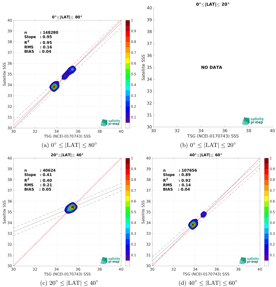
Figure 10: Contour maps of the concentration of Aquarius SSS L4 OI v5 - Monthly (IPRC) SSS (y-axis) versus TSG (NCEI-0170743) SSS (x-axis) at match-up pairs for different latitude bands. For each plot, the red line shows x=y . The black thin and dashed lines indicate a linear fit through the data cloud and the \pm 95\% confidence levels, respectively. The number match-up pairs n , the slope and R^2 coefficient of the linear fit, the root mean square (RMS) and the mean bias between satellite and in situ data are indicated for each latitude band in each plots.
