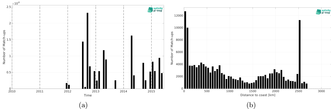
Figure 2: Number of match-ups between TSG (NCEI-0170743) and Aquarius SSS L4 OI v5 - Monthly (IPRC) SSS as a function of time (a) and as function of the distance to coast (b) over the Global Ocean Pi-MEP region and for the full satellite product period.
