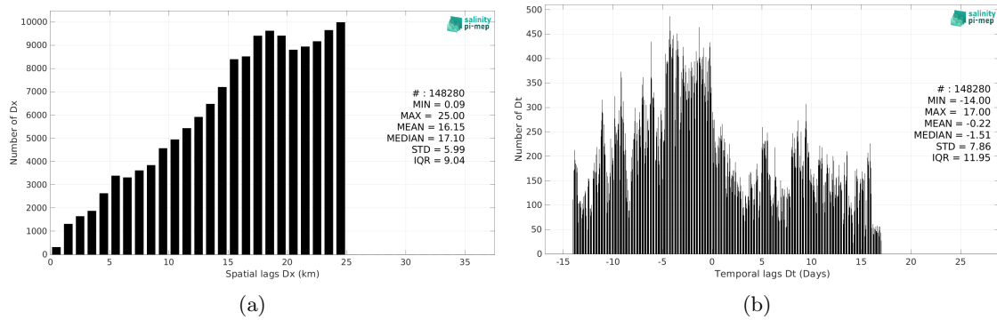
Figure 6: Histograms of the spatial (a) and temporal (b) lags between the location/time of the TSG (NCEI-0170743) measurement and the date of the corresponding Aquarius SSS L4 OI v5 - Monthly (IPRC) SSS pixel.
