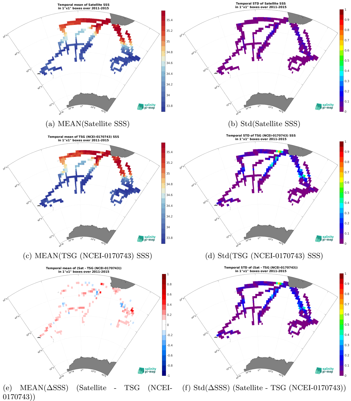
Figure 7: Temporal mean (left) and Std (right) of SSS from Aquarius SSS L4 OI v5 - Monthly (IPRC) (top), TSG (NCEI-0170743) (middle), and of \Delta SSS (Satellite - TSG (NCEI-0170743)). Only match-up pairs are used to generate these maps.
