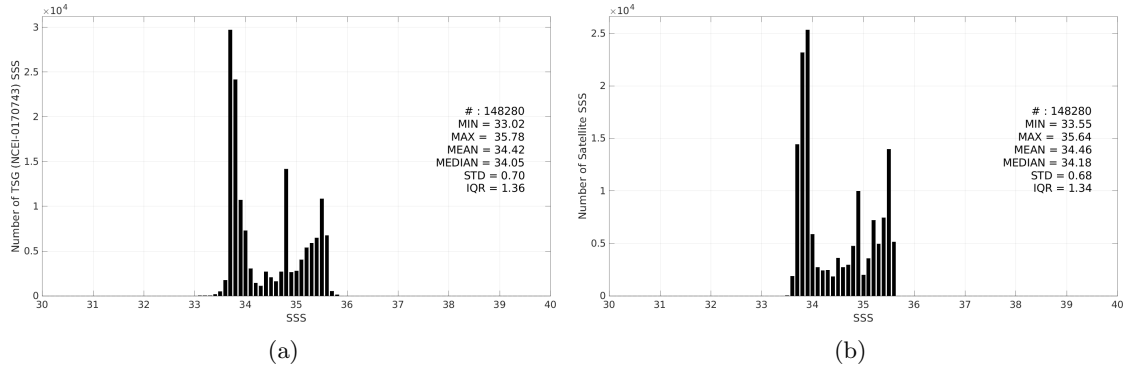
Figure 3: Histograms of SSS from TSG (NCEI-0170743) (a) and Aquarius SSS L4 OI v5 - Monthly (IPRC) (b) considering all match-up pairs per bins of 0.1 over the Global Ocean Pi-MEP region and for the full satellite product period.
