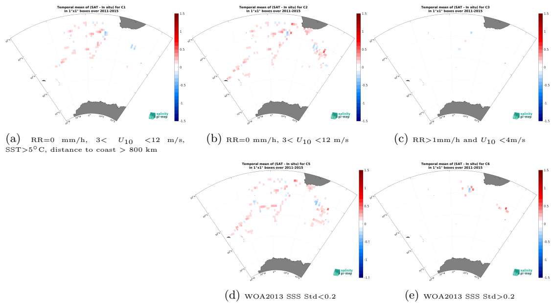
Figure 14: Temporal mean gridded over spatial boxes of size 1^\circ \times 1^\circ of \Delta SSS (Aquarius SSS L4 OI v5 - Monthly (IPRC) - TSG (NCEI-0170743)) for 5 different subdatasets corresponding to: RR=0 mm/h, 3 < U_{10} < 12 m/s, SST > 5^\circ\text{C} , distance to coast > 800 km (a), RR=0 mm/h, 3 < U_{10} < 12 m/s (b), RR > 1 mm/h and U_{10} < 4 m/s (c), WOA2013 SSS Std < 0.2 (d), WOA2013 SSS Std > 0.2 (e).
