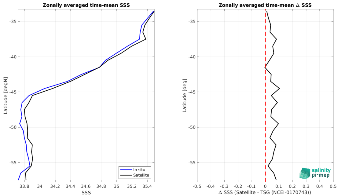
Figure 9: Left panel: Zonal mean SSS from Aquarius SSS L4 OI v5 - Monthly (IPRC) satellite product (black) and from TSG (NCEI-0170743) (blue). Right panel: Zonal mean of \Delta SSS (Satellite - TSG (NCEI-0170743)) for all the collected Pi-MEP match-up pairs estimated over the full satellite product period.
