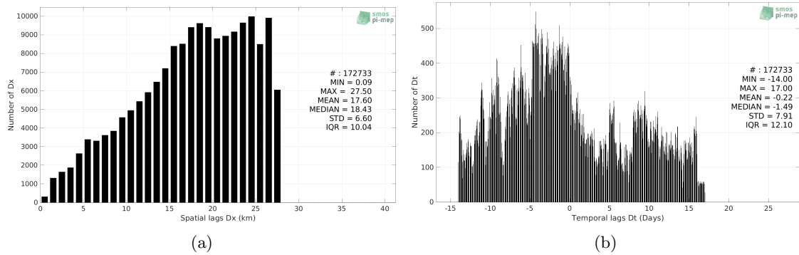
Figure 5: Histograms of the spatial (a) and temporal (b) lags between the location/time of the TSG (NCEI-0170743) measurement and the date of the corresponding Aquarius SSS L4 OI v5 - Monthly (IPRC) SSS pixel.
