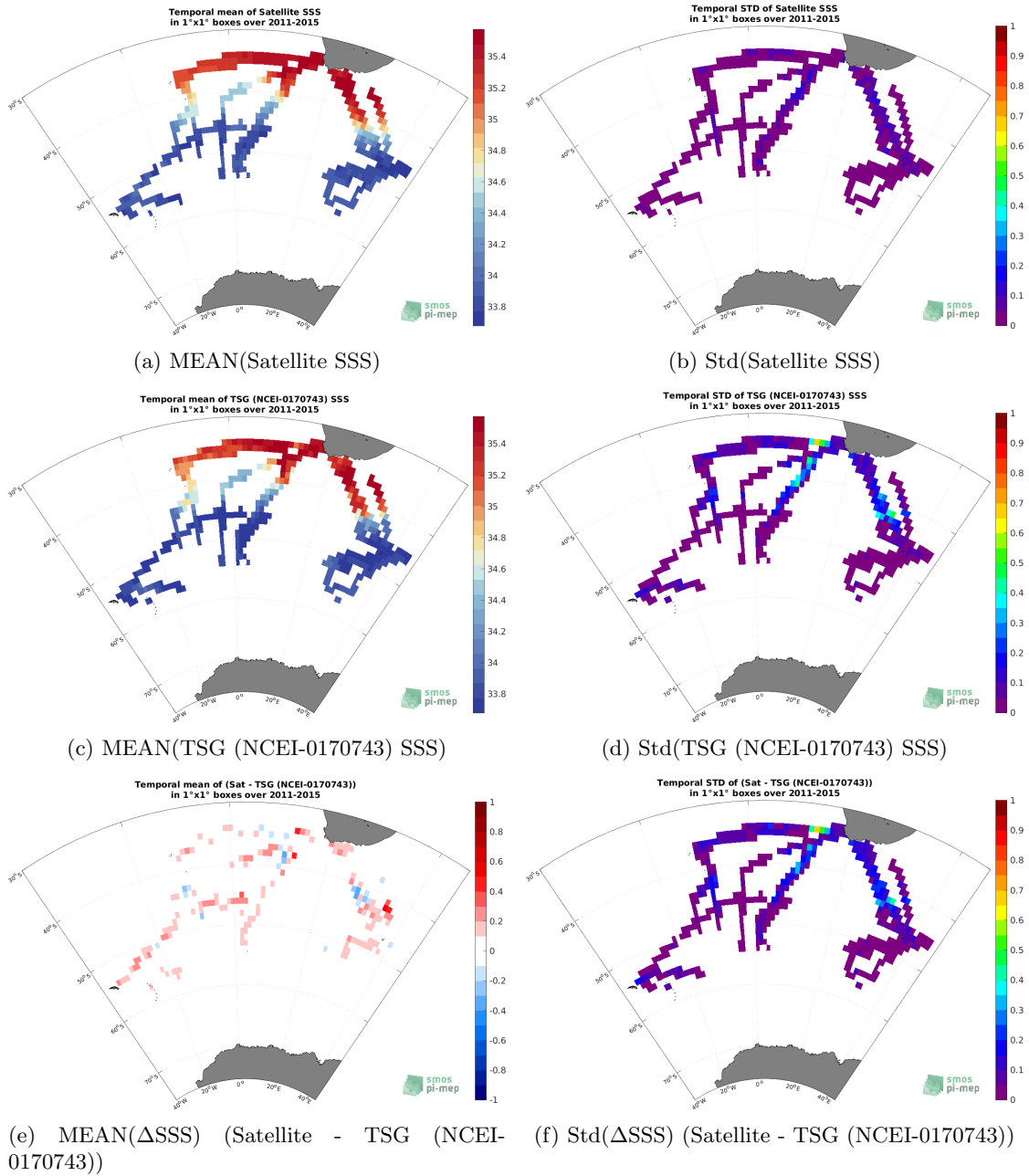
Figure 6: Temporal mean (left) and Std (right) of SSS from Aquarius SSS L4 OI v5 - Monthly (IPRC) (top), TSG (NCEI-0170743) (middle), and of \Delta SSS (Satellite - TSG (NCEI-0170743)). Only match-up pairs are used to generate these maps.
