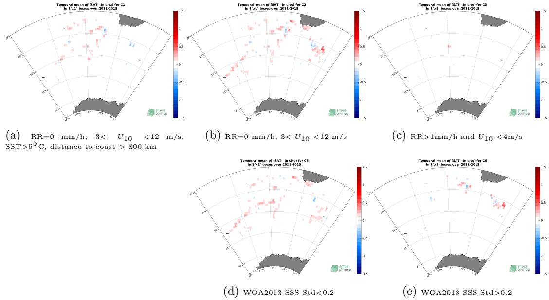
Figure 12: Temporal mean gridded over spatial boxes of size 1^\circ \times 1^\circ of \Delta SSS (Aquarius-L4-IPRC-V5-MONTHLY - TSG-NCEI-0170743) for 5 different subdatasets corresponding to: RR=0 mm/h, 3 < U_{10} < 12 m/s, SST > 5^\circ\text{C} , distance to coast > 800 km (a), RR=0 mm/h, 3 < U_{10} < 12 m/s (b), RR > 1\text{mm/h} and U_{10} < 4\text{m/s} (c), WOA2013 SSS Std < 0.2 (d), WOA2013 SSS Std > 0.2 (e).
