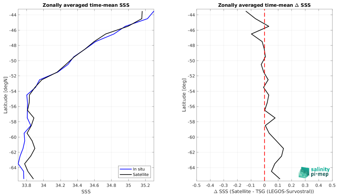
Figure 9: Left panel: Zonal mean SSS from Aquarius SSS L4 OI v5 - Monthly (IPRC) satellite product (black) and from TSG (LEGOS-Survostral) (blue). Right panel: Zonal mean of \Delta SSS (Satellite - TSG (LEGOS-Survostral)) for all the collected Pi-MEP match-up pairs estimated over the full satellite product period.
