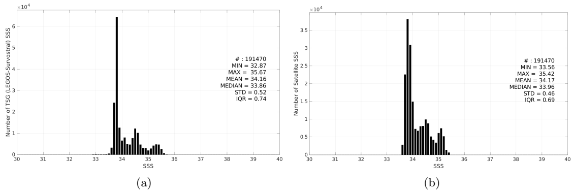
Figure 3: Histograms of SSS from TSG (LEGOS-Survostral) (a) and Aquarius SSS L4 OI v5 - Monthly (IPRC) (b) considering all match-up pairs per bins of 0.1 over the Global Ocean Pi-MEP region and for the full satellite product period.
