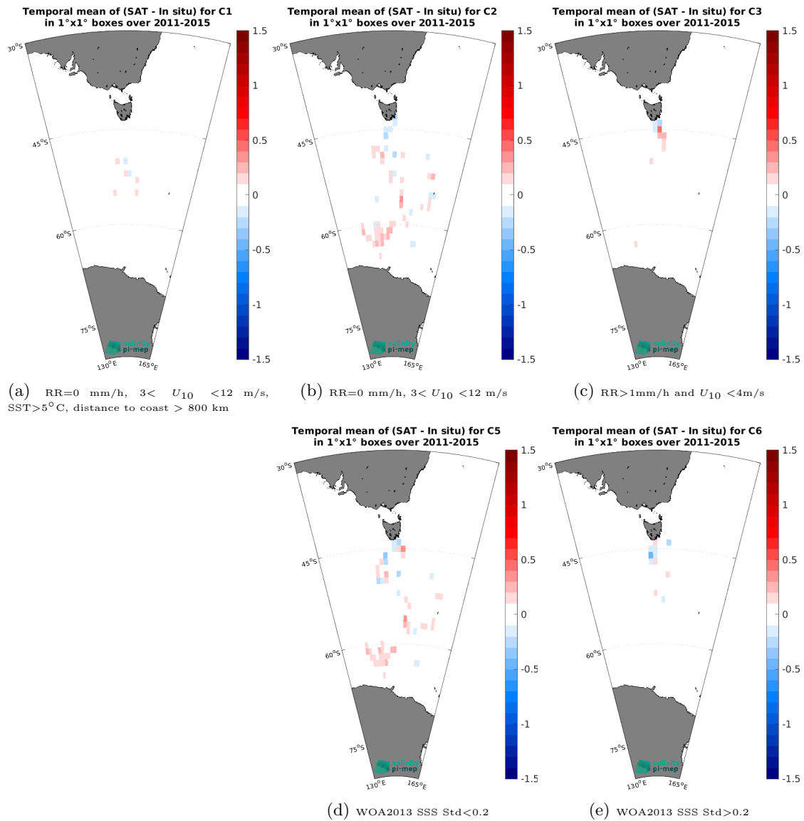
Figure 14: Temporal mean gridded over spatial boxes of size 1^\circ \times 1^\circ of \Delta SSS (Aquarius SSS L4 OI v5 - Monthly (IPRC) - TSG (LEGOS-Survostral)) for 5 different subdatasets corresponding to: RR=0 mm/h, 3 < U_{10} < 12 m/s, SST>5°C, distance to coast > 800 km (a), RR=0 mm/h, 3 < U_{10} < 12 m/s (b), RR>1mm/h and U_{10} < 4 m/s (c), WOA2013 SSS Std<0.2 (d), WOA2013 SSS Std>0.2 (e).
