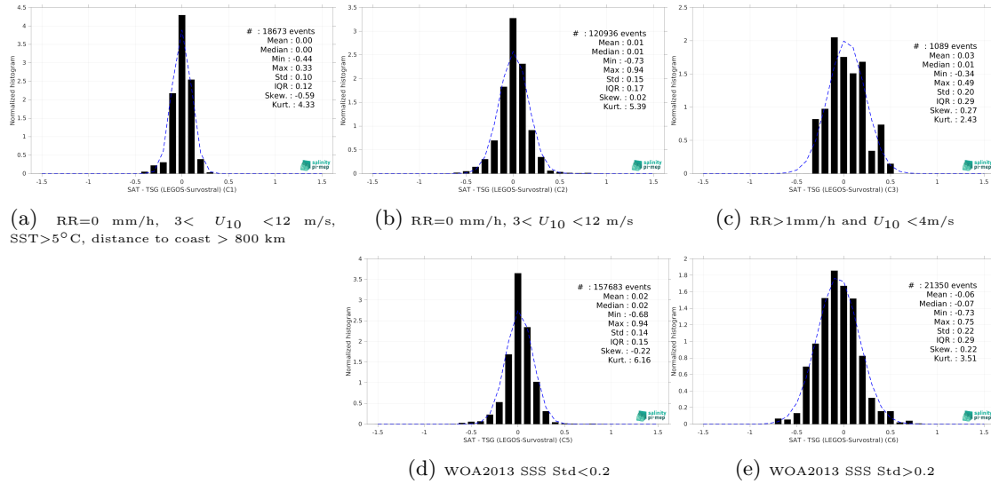
Figure 15: Normalized histogram of \Delta SSS (Aquarius SSS L4 OI v5 - Monthly (IPRC) - TSG (LEGOS-Survostral)) for 5 different subdatasets corresponding to: RR=0 mm/h, 3 < U_{10} < 12 m/s, SST>5°C, distance to coast > 800 km (a), RR=0 mm/h, 3 < U_{10} < 12 m/s (b), RR>1mm/h and U_{10} < 4 m/s (c), WOA2013 SSS Std<0.2 (d), WOA2013 SSS Std>0.2 (e).
