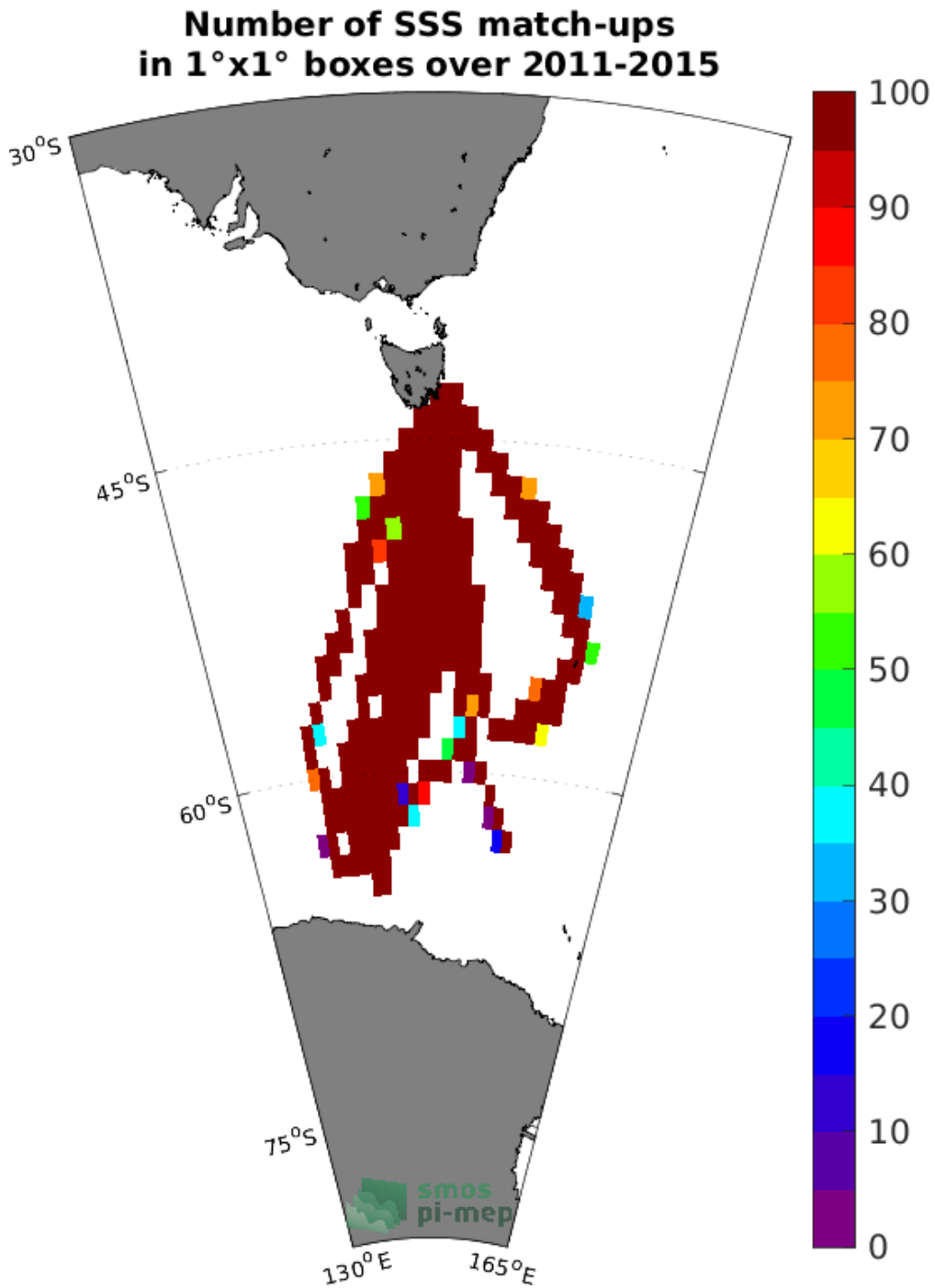
Figure 4: Number of SSS match-ups between TSG (LEGOS-Survostral) SSS and the Aquarius SSS L4 OI v5 - Monthly (IPRC) SSS product for the Global Ocean Pi-MEP region over 1°x1° boxes and for the full satellite product period.
