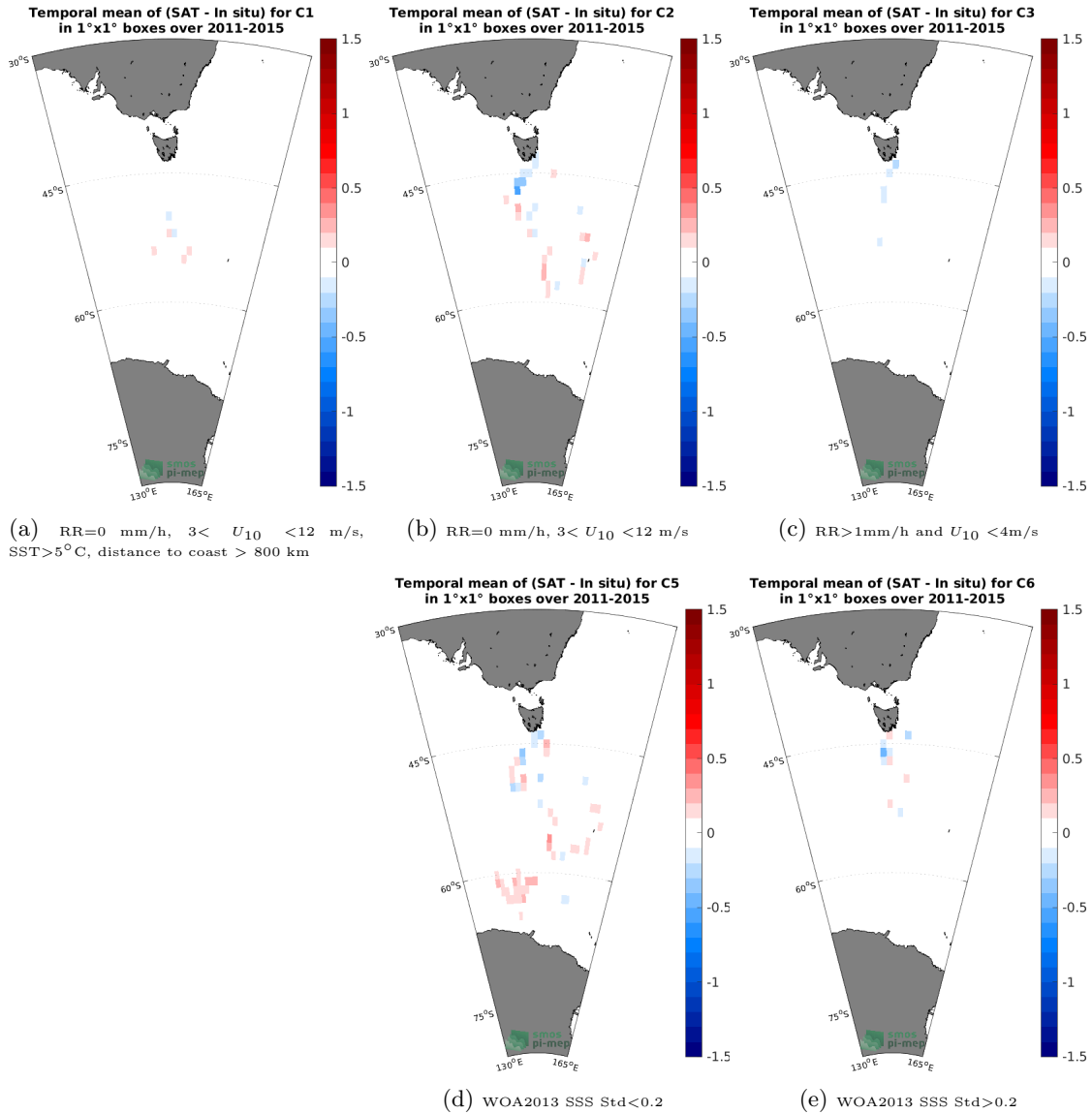
Figure 12: Temporal mean gridded over spatial boxes of size 1^\circ \times 1^\circ of \Delta SSS (Aquarius SSS L4 OI v5 - Monthly (IPRC) - TSG (LEGOS-Survostral)) for 5 different subdatasets corresponding to: RR=0 mm/h, 3 < U_{10} < 12 m/s, SST>5°C, distance to coast > 800 km (a), RR=0 mm/h, 3 < U_{10} < 12 m/s (b), RR>1mm/h and U_{10} < 4 m/s (c), WOA2013 SSS Std<0.2 (d), WOA2013 SSS Std>0.2 (e).
