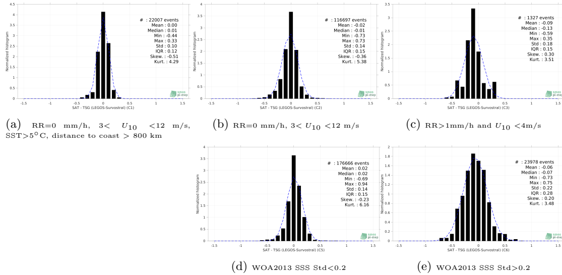
Figure 13: Normalized histogram of \Delta SSS (Aquarius SSS L4 OI v5 - Monthly (IPRC) - TSG (LEGOS-Survostral)) for 5 different subdatasets corresponding to: RR=0 mm/h, 3 < U_{10} < 12 m/s, SST > 5°C, distance to coast > 800 km (a), RR=0 mm/h, 3 < U_{10} < 12 m/s (b), RR > 1mm/h and U_{10} < 4 m/s (c), WOA2013 SSS Std < 0.2 (d), WOA2013 SSS Std > 0.2 (e).
