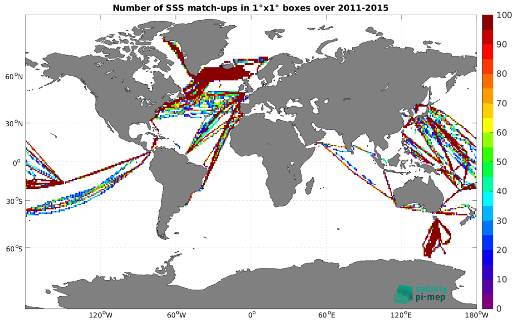
Figure 5: Number of SSS match-ups between TSG (LEGOS-DM) SSS and the Aquarius SSS L4 OI v5 - Monthly (IPRC) SSS product for the Global Ocean Pi-MEP region over 1^\circ \times 1^\circ boxes and for the full satellite product period.
