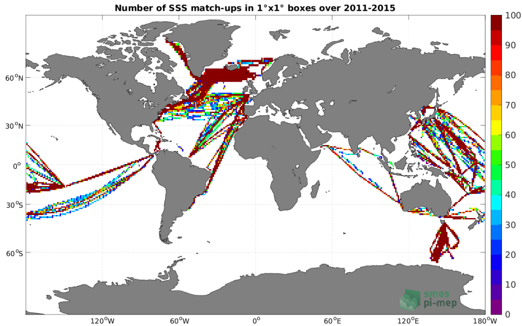
Figure 4: Number of SSS match-ups between TSG (LEGOS-DM) SSS and the Aquarius SSS L4 OI v5 - Monthly (IPRC) SSS product for the Global Ocean Pi-MEP region over 1^\circ \times 1^\circ boxes and for the full satellite product period.
