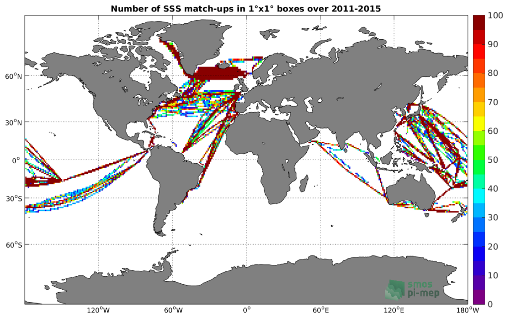
Figure 4: Number of SSS match-ups between TSG-LEGOS-DM SSS and the Aquarius-L4-IPRC-V5-MONTHLY SSS product for the Global Ocean Pi-MEP region over 1°x1° boxes and for the full satellite product period.
