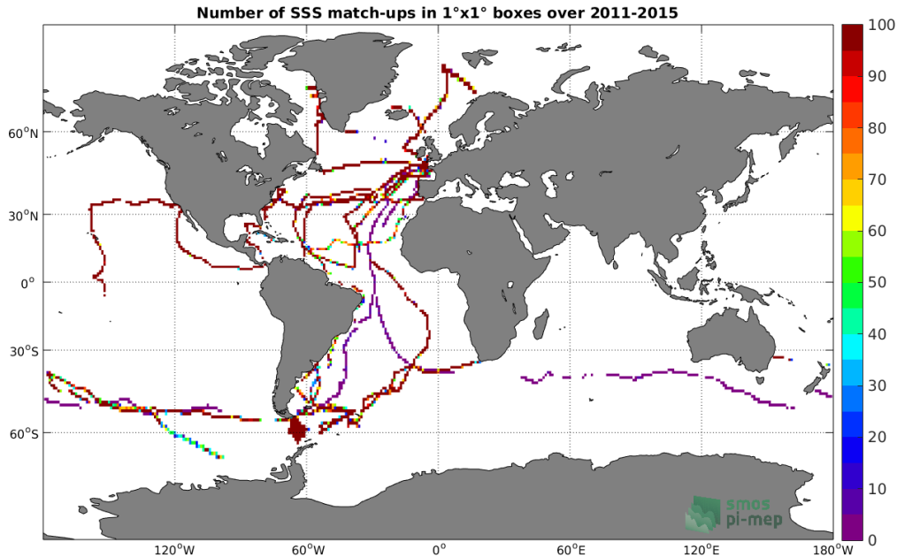
Figure 4: Number of SSS match-ups between TSG (GOSUD-Sailing-ship) SSS and the Aquarius SSS L4 OI v5 - Monthly (IPRC) SSS product for the Global Ocean Pi-MEP region over 1^\circ \times 1^\circ boxes and for the full satellite product period.
