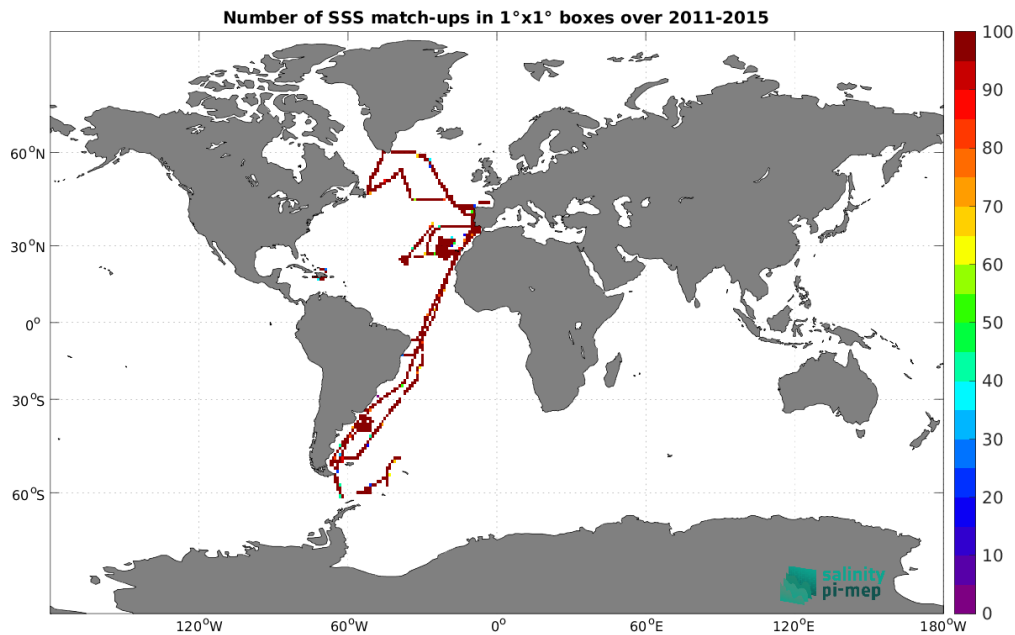
Figure 5: Number of SSS match-ups between TSG (CSIC-UTM) SSS and the Aquarius SSS L4 OI v5 - Monthly (IPRC) SSS product for the Global Ocean Pi-MEP region over 1^\circ \times 1^\circ boxes and for the full satellite product period.
