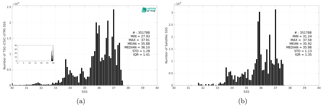
Figure 3: Histograms of SSS from TSG (CSIC-UTM) (a) and Aquarius SSS L4 OI v5 - Monthly (IPRC) (b) considering all match-up pairs per bins of 0.1 over the Global Ocean Pi-MEP region and for the full satellite product period.
