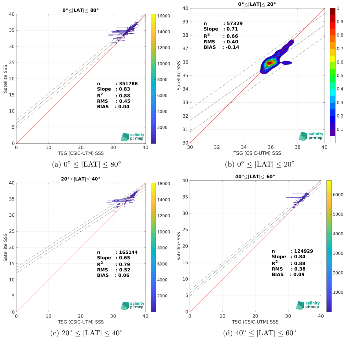
Figure 10: Contour maps of the concentration of Aquarius SSS L4 OI v5 - Monthly (IPRC) SSS (y-axis) versus TSG (CSIC-UTM) SSS (x-axis) at match-up pairs for different latitude bands. For each plot, the red line shows x=y . The black thin and dashed lines indicate a linear fit through the data cloud and the \pm 95\% confidence levels, respectively. The number match-up pairs n , the slope and R^2 coefficient of the linear fit, the root mean square (RMS) and the mean bias between satellite and in situ data are indicated for each latitude band in each plots.
