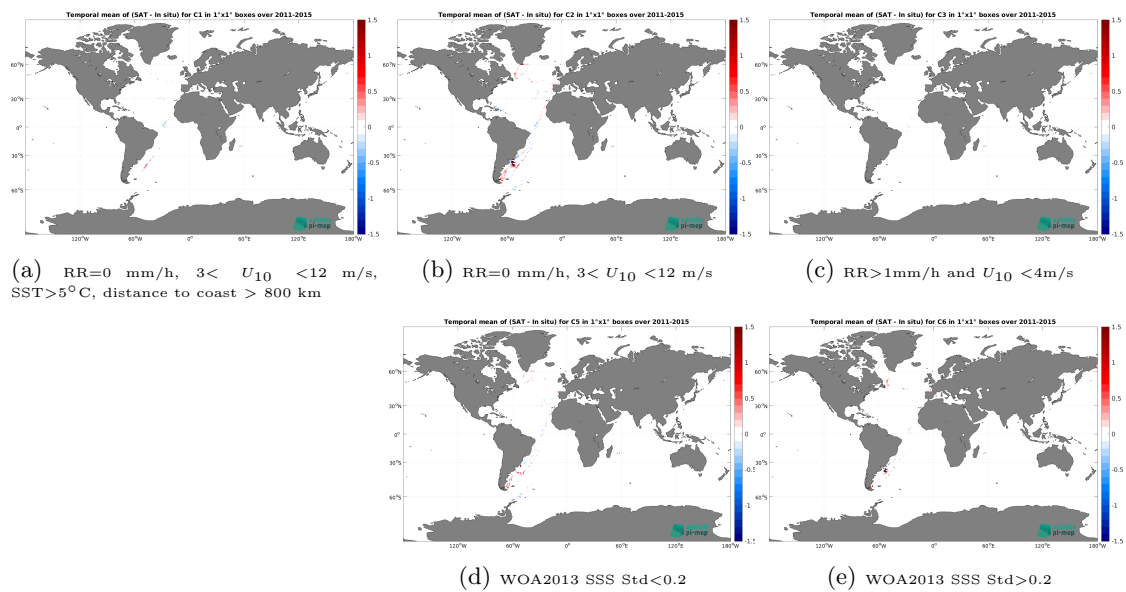
Figure 14: Temporal mean gridded over spatial boxes of size 1^\circ \times 1^\circ of \Delta SSS (Aquarius SSS L4 OI v5 - Monthly (IPRC) - TSG (CSIC-UTM)) for 5 different subdatasets corresponding to:RR=0 mm/h, 3 < U_{10} < 12 m/s, SST > 5^\circ\text{C} , distance to coast > 800 km (a), RR=0 mm/h, 3 < U_{10} < 12 m/s (b), RR > 1 mm/h and U_{10} < 4 m/s (c), WOA2013 SSS Std < 0.2 (d), WOA2013 SSS Std > 0.2 (e).
