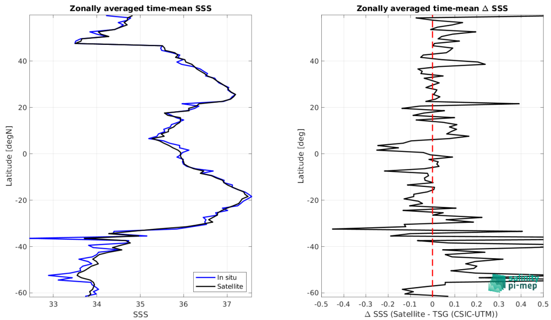
Figure 9: Left panel: Zonal mean SSS from Aquarius SSS L4 OI v5 - Monthly (IPRC) satellite product (black) and from TSG (CSIC-UTM) (blue). Right panel: Zonal mean of \Delta SSS (Satellite - TSG (CSIC-UTM)) for all the collected Pi-MEP match-up pairs estimated over the full satellite product period.
