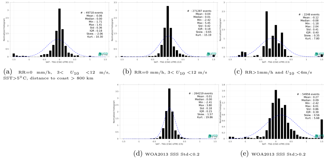
Figure 15: Normalized histogram of \Delta SSS (Aquarius SSS L4 OI v5 - Monthly (IPRC) - TSG (CSIC-UTM)) for 5 different subdatasets corresponding to: RR=0 mm/h, 3 < U_{10} < 12 m/s, SST>5°C, distance to coast > 800 km (a), RR=0 mm/h, 3 < U_{10} < 12 m/s (b), RR>1mm/h and U_{10} < 4 m/s (c), WOA2013 SSS Std<0.2 (d), WOA2013 SSS Std>0.2 (e).
