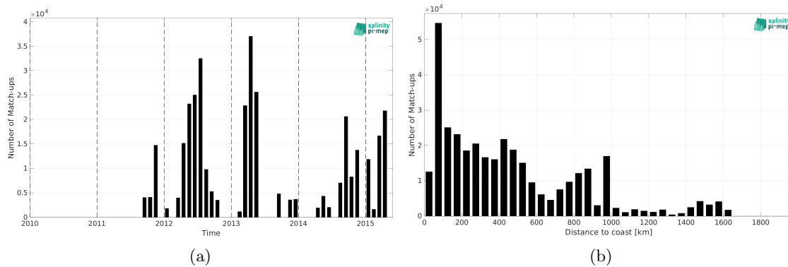
Figure 2: Number of match-ups between TSG (CSIC-UTM) and Aquarius SSS L4 OI v5 - Monthly (IPRC) SSS as a function of time (a) and as function of the distance to coast (b) over the Global Ocean Pi-MEP region and for the full satellite product period.
