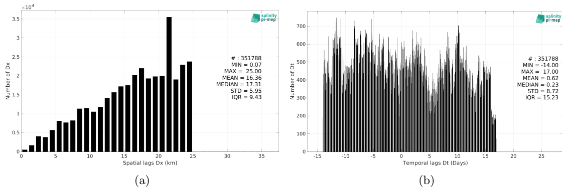
Figure 6: Histograms of the spatial (a) and temporal (b) lags between the location/time of the TSG (CSIC-UTM) measurement and the date of the corresponding Aquarius SSS L4 OI v5 - Monthly (IPRC) SSS pixel.
