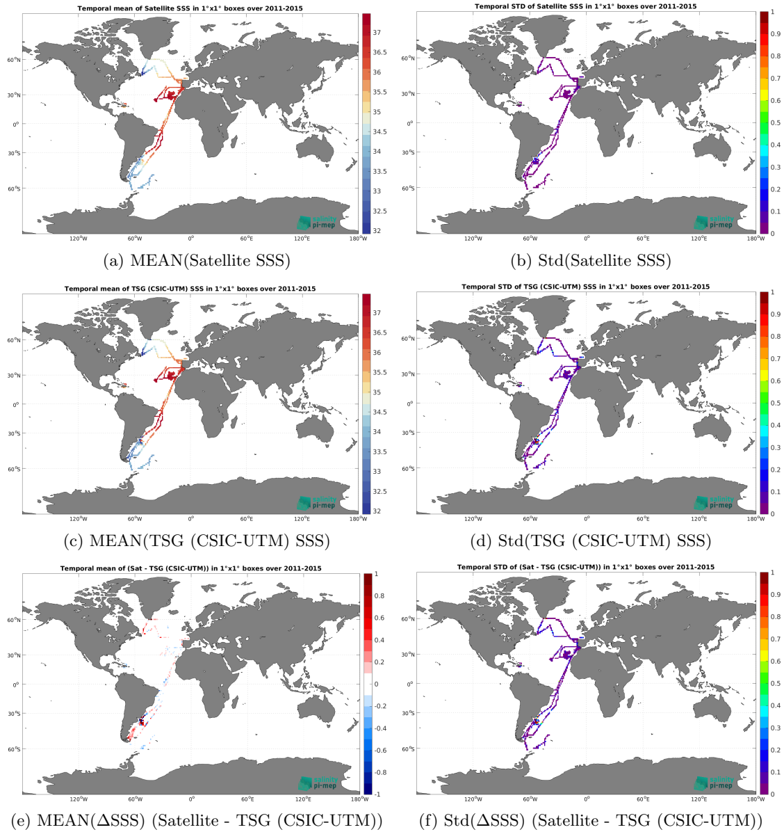
Figure 7: Temporal mean (left) and Std (right) of SSS from Aquarius SSS L4 OI v5 - Monthly (IPRC) (top), TSG (CSIC-UTM) (middle), and of \Delta SSS (Satellite - TSG (CSIC-UTM)). Only match-up pairs are used to generate these maps.
