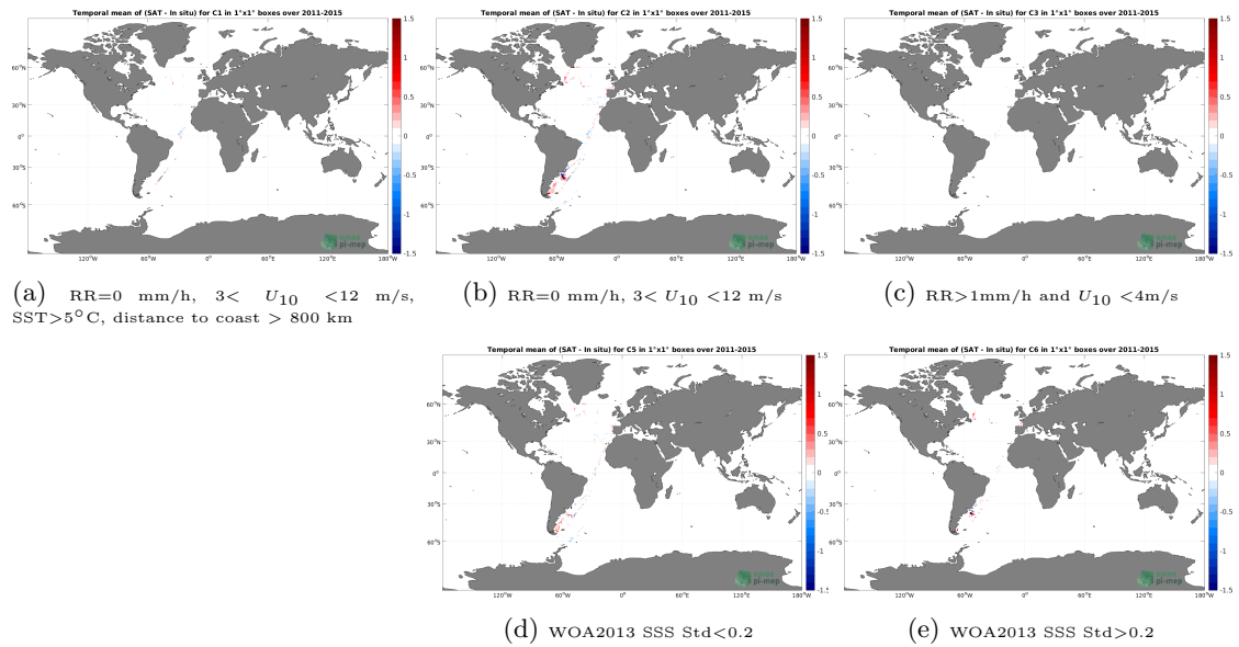
Figure 12: Temporal mean gridded over spatial boxes of size 1^\circ \times 1^\circ of \Delta SSS (Aquarius SSS L4 OI v5 - Monthly (IPRC) - TSG (CSIC-UTM)) for 5 different subdatasets corresponding to:RR=0 mm/h, 3 < U_{10} < 12 m/s, SST > 5^\circ\text{C} , distance to coast > 800 km (a), RR=0 mm/h, 3 < U_{10} < 12 m/s (b), RR > 1 mm/h and U_{10} < 4 m/s (c), WOA2013 SSS Std < 0.2 (d), WOA2013 SSS Std > 0.2 (e).
