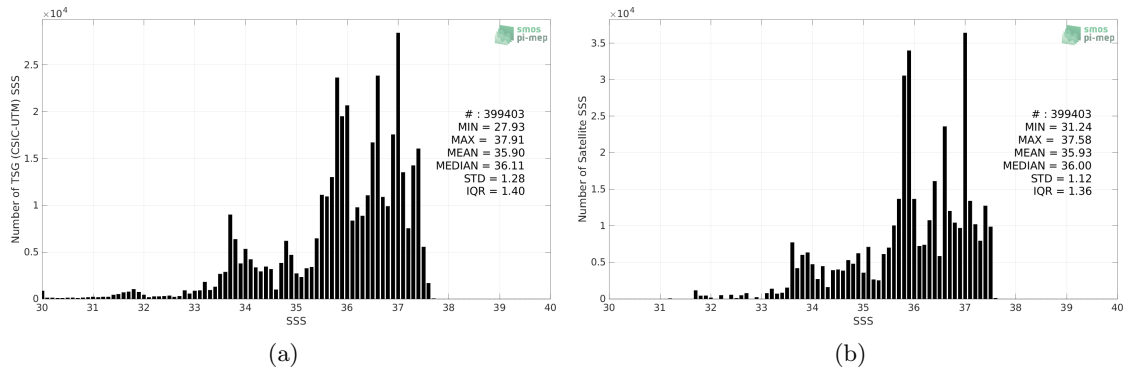
Figure 2: Histograms of SSS from TSG (CSIC-UTM) (a) and Aquarius SSS L4 OI v5 - Monthly (IPRC) (b) considering all match-up pairs per bins of 0.1 over the Global Ocean Pi-MEP region and for the full satellite product period.
