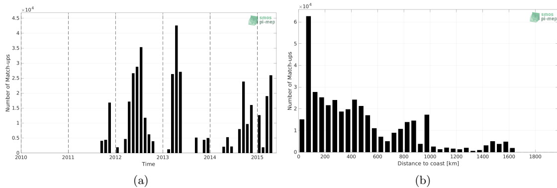
Figure 1: Number of match-ups between TSG (CSIC-UTM) and Aquarius SSS L4 OI v5 - Monthly (IPRC) SSS as a function of time (a) and as function of the distance to coast (b) over the Global Ocean Pi-MEP region and for the full satellite product period.
