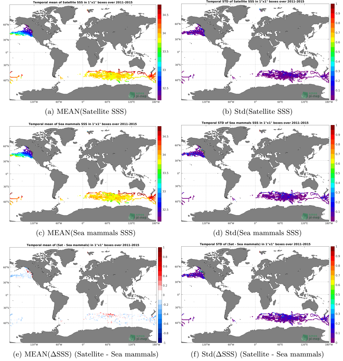
Figure 6: Temporal mean (left) and Std (right) of SSS from Aquarius SSS L4 OI v5 - Monthly (IPRC) (top), Sea mammals (middle), and of \Delta SSS (Satellite - Sea mammals). Only match-up pairs are used to generate these maps.
