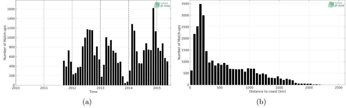
Figure 1: Number of match-ups between Sea mammals and Aquarius SSS L4 OI v5 - Monthly (IPRC) SSS as a function of time (a) and as function of the distance to coast (b) over the Global Ocean Pi-MEP region and for the full satellite product period.
