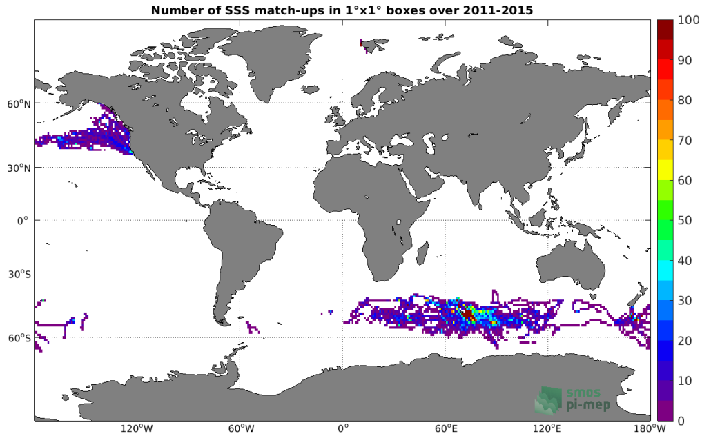
Figure 4: Number of SSS match-ups between Sea mammals SSS and the Aquarius SSS L4 OI v5 - Monthly (IPRC) SSS product for the Global Ocean Pi-MEP region over 1°x1° boxes and for the full satellite product period.
