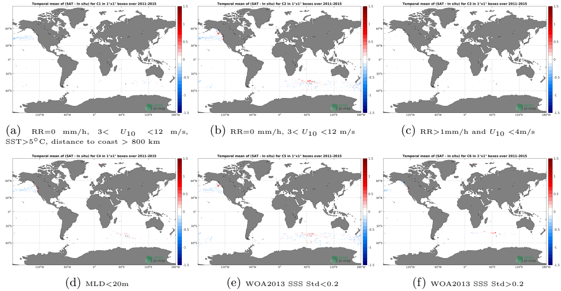
Figure 12: Temporal mean gridded over spatial boxes of size 1^\circ \times 1^\circ of \Delta SSS (Aquarius SSS L4 OI v5 - Monthly (IPRC) - Sea mammals) for 6 different subdatasets corresponding to: RR=0 mm/h, 3 < U_{10} < 12 m/s, SST > 5^\circ C , distance to coast > 800 km (a), RR=0 mm/h, 3 < U_{10} < 12 m/s (b), RR > 1 mm/h and U_{10} < 4 m/s (c), MLD < 20 m (d), WOA2013 SSS Std < 0.2 (e), WOA2013 SSS Std > 0.2 (f).
