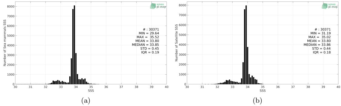
Figure 2: Histograms of SSS from Sea mammals (a) and Aquarius SSS L4 OI v5 - Monthly (IPRC) (b) considering all match-up pairs per bins of 0.1 over the Global Ocean Pi-MEP region and for the full satellite product period.
