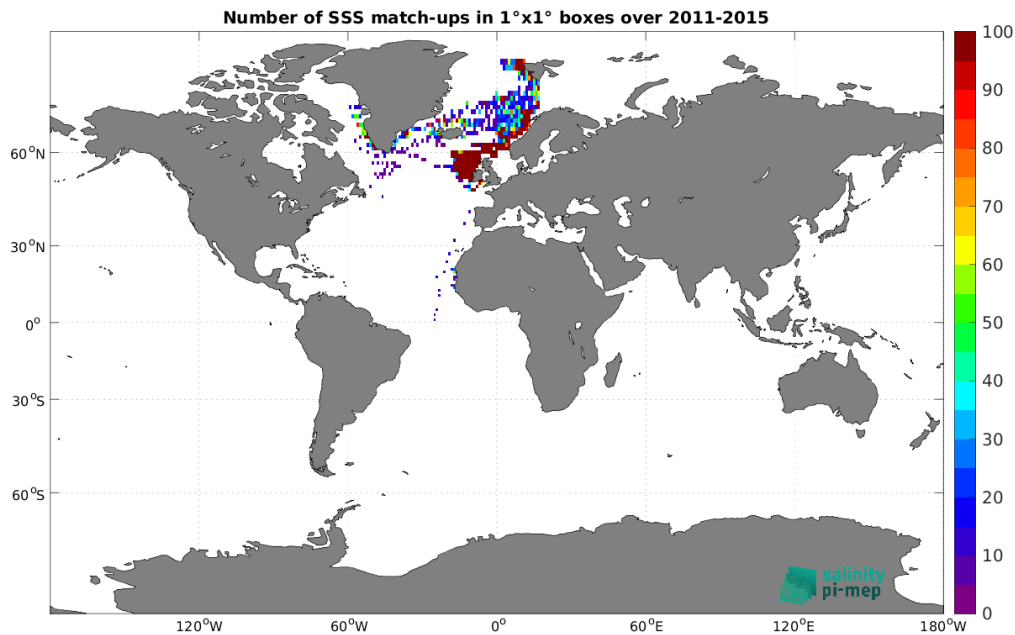
Figure 5: Number of SSS match-ups between ICES SSS and the Aquarius SSS L4 OI v5 - Monthly (IPRC) SSS product for the Global Ocean Pi-MEP region over 1^\circ \times 1^\circ boxes and for the full satellite product period.
