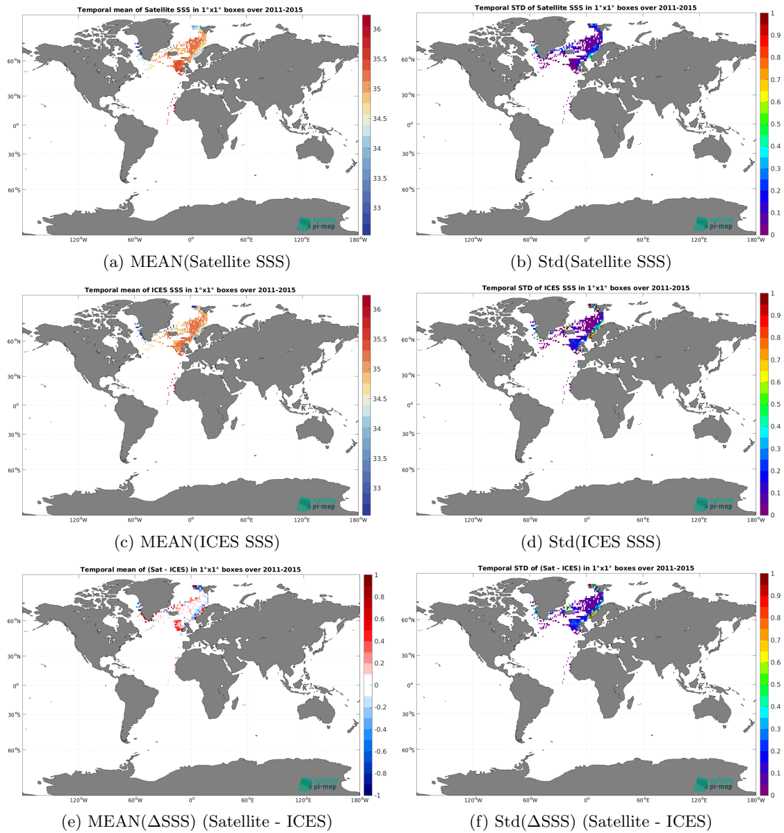
Figure 7: Temporal mean (left) and Std (right) of SSS from Aquarius SSS L4 OI v5 - Monthly (IPRC) (top), ICES (middle), and of \Delta SSS (Satellite - ICES). Only match-up pairs are used to generate these maps.
