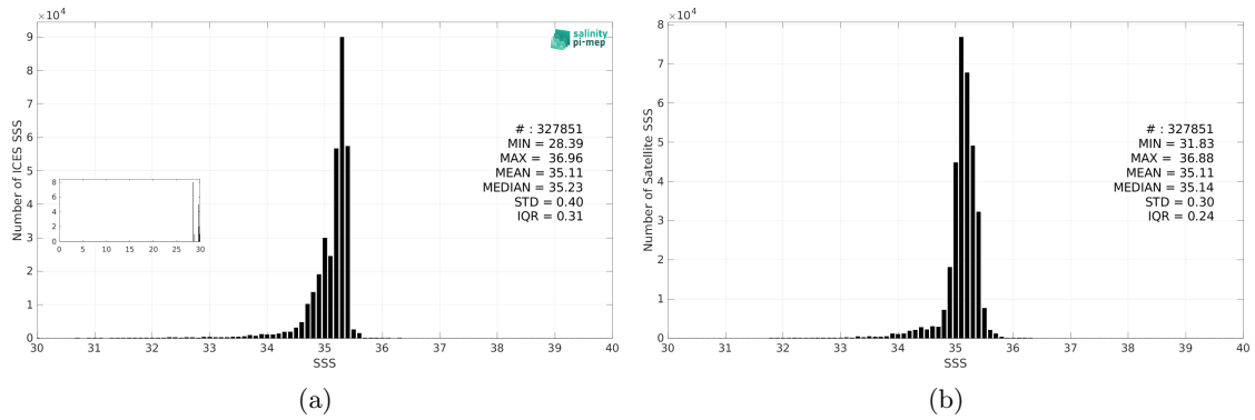
Figure 3: Histograms of SSS from ICES (a) and Aquarius SSS L4 OI v5 - Monthly (IPRC) (b) considering all match-up pairs per bins of 0.1 over the Global Ocean Pi-MEP region and for the full satellite product period.
