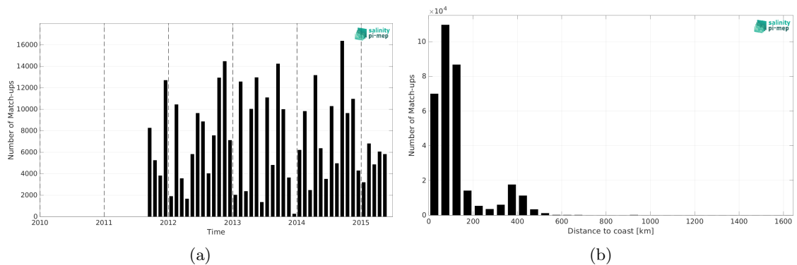
Figure 2: Number of match-ups between ICES and Aquarius SSS L4 OI v5 - Monthly (IPRC) SSS as a function of time (a) and as function of the distance to coast (b) over the Global Ocean Pi-MEP region and for the full satellite product period.
