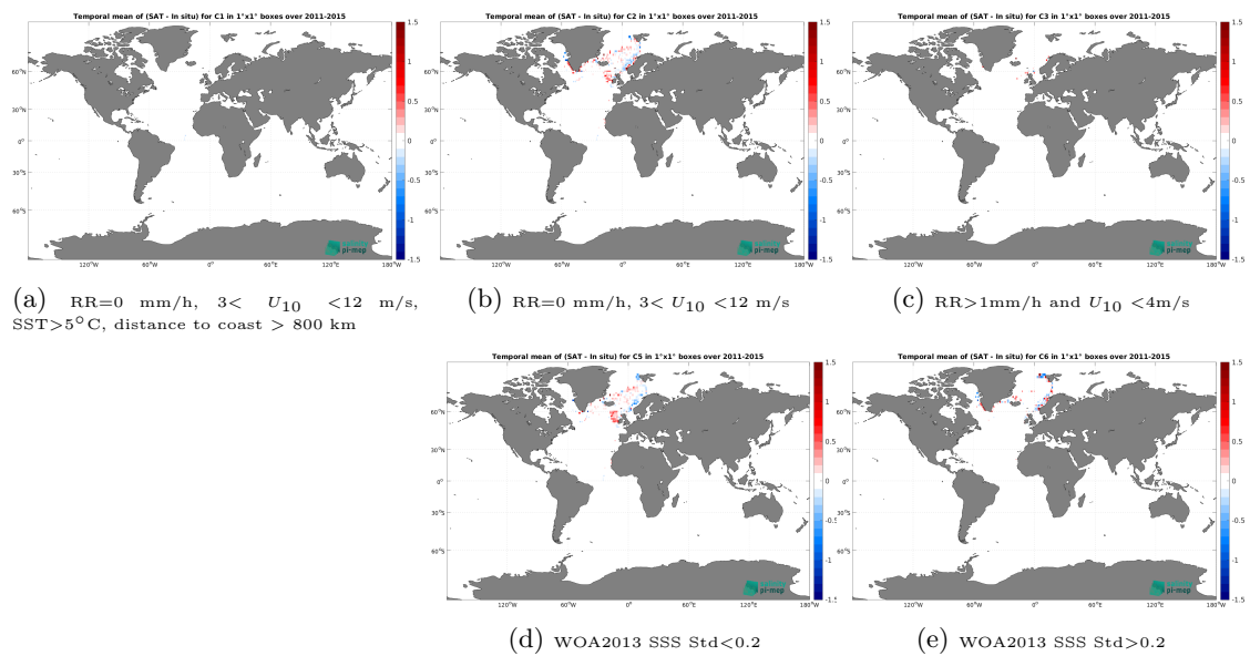
Figure 14: Temporal mean gridded over spatial boxes of size 1^\circ \times 1^\circ of \Delta SSS (Aquarius SSS L4 OI v5 - Monthly (IPRC) - ICES) for 5 different subdatasets corresponding to:RR=0 mm/h, 3 < U_{10} < 12 m/s, SST > 5^\circ\text{C} , distance to coast > 800 km (a), RR=0 mm/h, 3 < U_{10} < 12 m/s (b), RR > 1 mm/h and U_{10} < 4 m/s (c), WOA2013 SSS Std < 0.2 (d), WOA2013 SSS Std > 0.2 (e).
