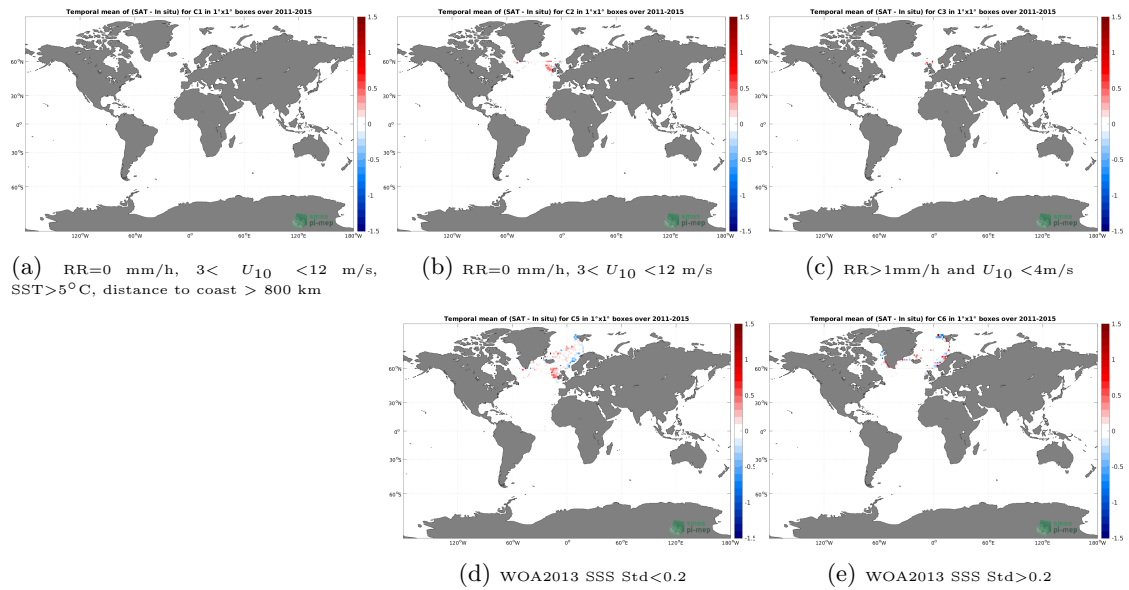
Figure 12: Temporal mean gridded over spatial boxes of size 1^\circ \times 1^\circ of \Delta SSS (Aquarius SSS L4 OI v5 - Monthly (IPRC) - ICES) for 5 different subdatasets corresponding to:RR=0 mm/h, 3 < U_{10} < 12 m/s, SST >5^\circ C, distance to coast > 800 km (a), RR=0 mm/h, 3 < U_{10} < 12 m/s (b), RR >1 mm/h and U_{10} < 4 m/s (c), WOA2013 SSS Std <0.2 (d), WOA2013 SSS Std >0.2 (e).
