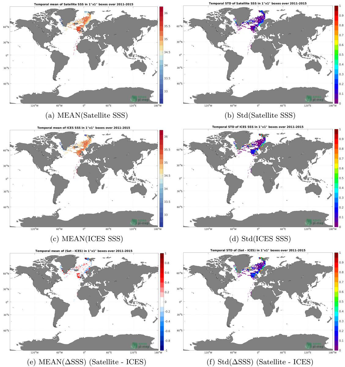
Figure 6: Temporal mean (left) and Std (right) of SSS from Aquarius SSS L4 OI v5 - Monthly (IPRC) (top), ICES (middle), and of \Delta SSS (Satellite - ICES). Only match-up pairs are used to generate these maps.
