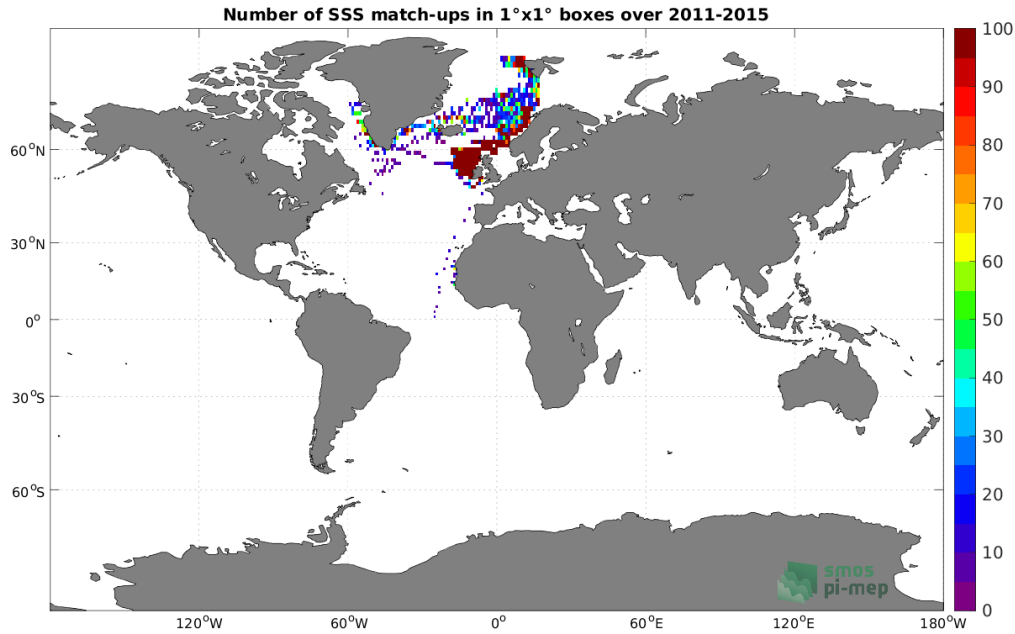
Figure 4: Number of SSS match-ups between ICES SSS and the Aquarius SSS L4 OI v5 - Monthly (IPRC) SSS product for the Global Ocean Pi-MEP region over 1^\circ \times 1^\circ boxes and for the full satellite product period.
