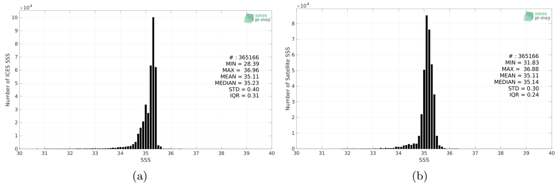
Figure 2: Histograms of SSS from ICES (a) and Aquarius SSS L4 OI v5 - Monthly (IPRC) (b) considering all match-up pairs per bins of 0.1 over the Global Ocean Pi-MEP region and for the full satellite product period.
