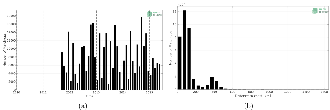
Figure 1: Number of match-ups between ICES and Aquarius SSS L4 OI v5 - Monthly (IPRC) SSS as a function of time (a) and as function of the distance to coast (b) over the Global Ocean Pi-MEP region and for the full satellite product period.
