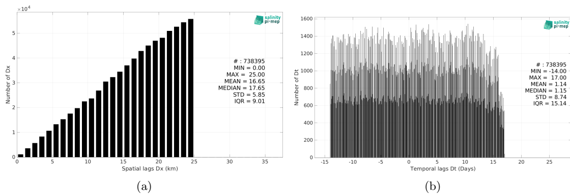
Figure 5: Histograms of the spatial (a) and temporal (b) lags between the location/time of the Surface drifters measurement and the date of the corresponding Aquarius SSS L4 OI v5 - Monthly (IPRC) SSS pixel.
