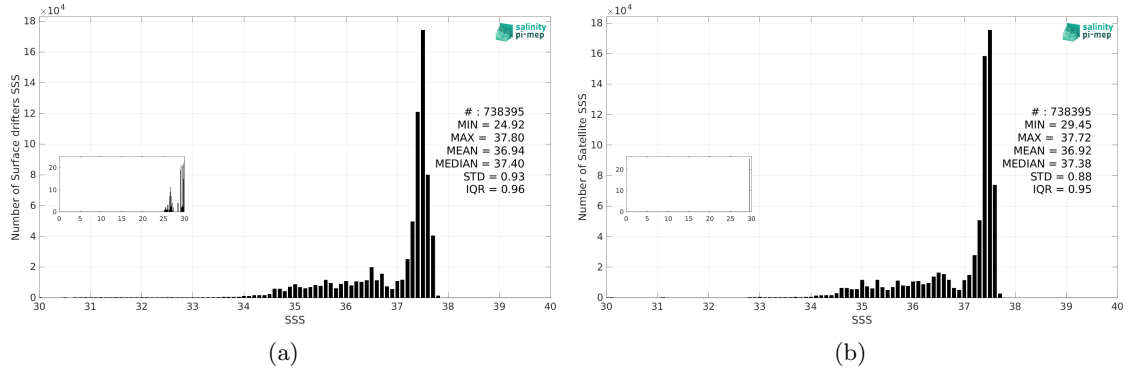
Figure 3: Histograms of SSS from Surface drifters (a) and Aquarius SSS L4 OI v5 - Monthly (IPRC) (b) considering all match-up pairs per bins of 0.1 over the Global Ocean Pi-MEP region and for the full satellite product period.
