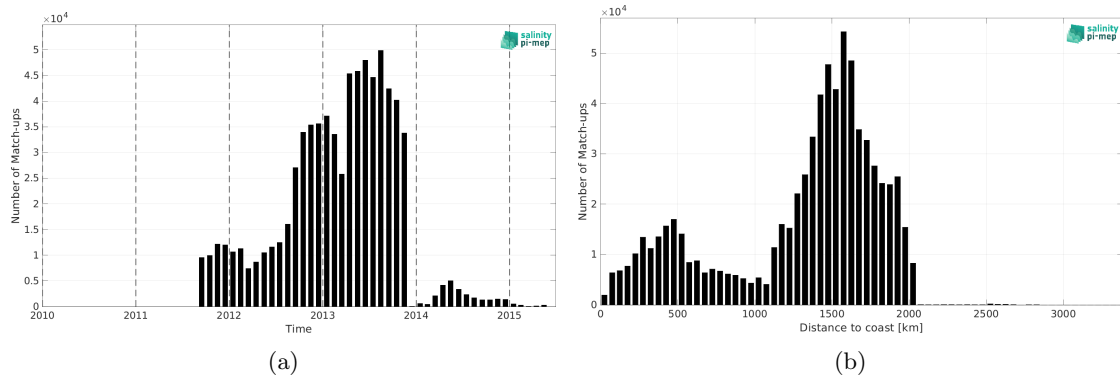
Figure 2: Number of match-ups between Surface drifters and Aquarius SSS L4 OI v5 - Monthly (IPRC) SSS as a function of time (a) and as function of the distance to coast (b) over the Global Ocean Pi-MEP region and for the full satellite product period.
