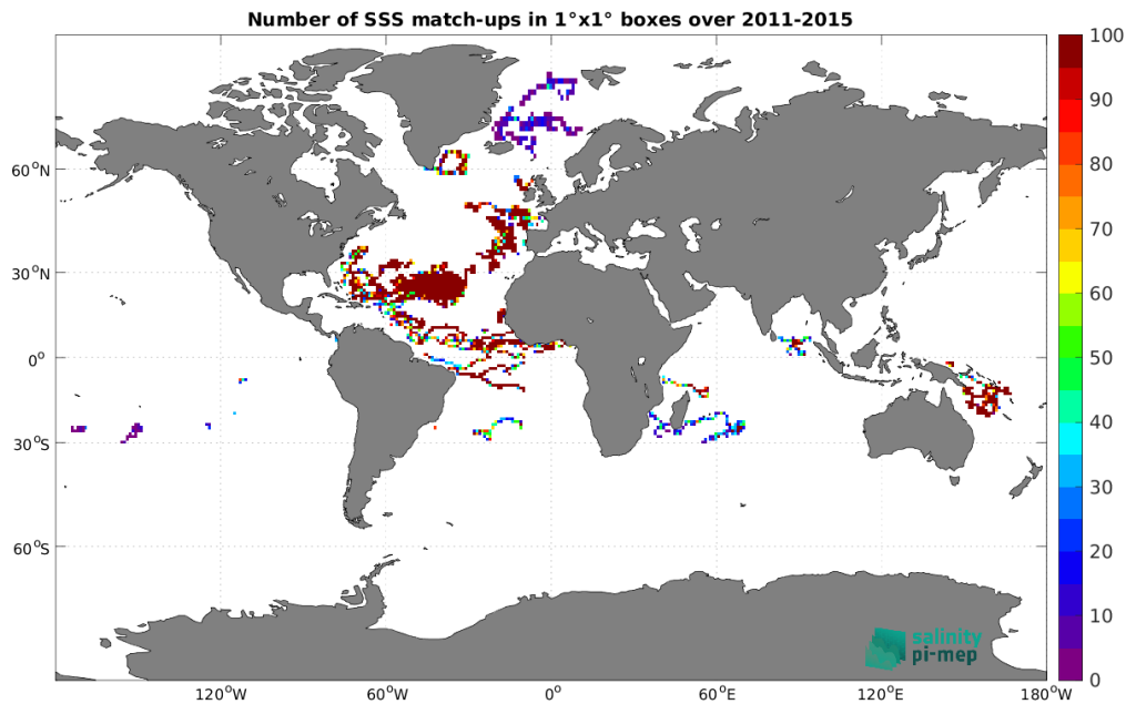
Figure 4: Number of SSS match-ups between Surface drifters SSS and the Aquarius SSS L4 OI v5 - Monthly (IPRC) SSS product for the Global Ocean Pi-MEP region over 1°×1° boxes and for the full satellite product period.
