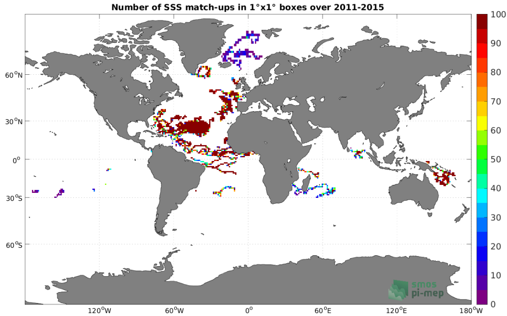
Figure 3: Number of SSS match-ups between Surface drifters SSS and the Aquarius SSS L4 OI v5 - Monthly (IPRC) SSS product for the Global Ocean Pi-MEP region over 1^\circ \times 1^\circ boxes and for the full satellite product period.
