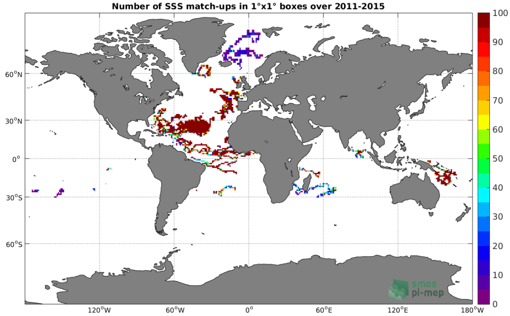
Figure 3: Number of SSS match-ups between Surface drifters SSS and the Aquarius-L4-IPRC-V5-MONTHLY SSS product for the Global Ocean Pi-MEP region over 1^\circ \times 1^\circ boxes and for the full satellite product period.
