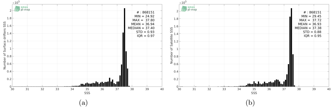
Figure 2: Histograms of SSS from Surface drifters (a) and Aquarius-L4-IPRC-V5-MONTHLY (b) considering all match-up pairs per bins of 0.1 over the Global Ocean Pi-MEP region and for the full satellite product period.
