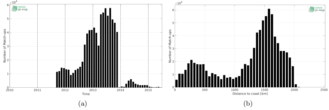
Figure 1: Number of match-ups between Surface drifters and Aquarius-L4-IPRC-V5-MONTHLY SSS as a function of time (a) and as function of the distance to coast (b) over the Global Ocean Pi-MEP region and for the full satellite product period.
