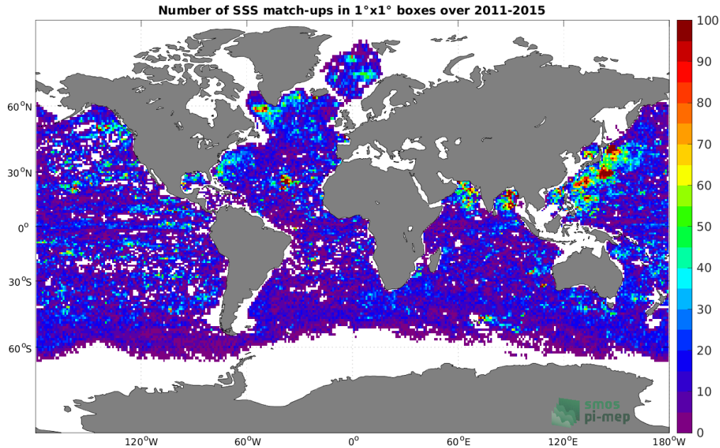
Figure 4: Number of SSS match-ups between Argo SSS and the Aquarius SSS L4 OI v5 - Monthly (IPRC) SSS product for the Global Ocean Pi-MEP region over 1^\circ \times 1^\circ boxes and for the full satellite product period.
