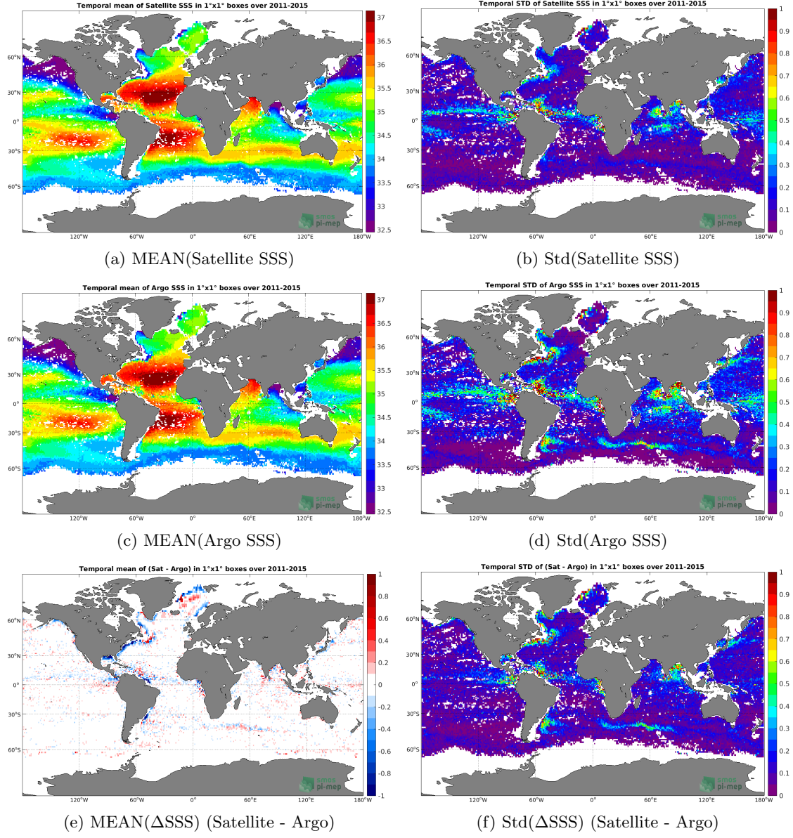
Figure 6: Temporal mean (left) and Std (right) of SSS from Aquarius SSS L4 OI v5 - Monthly (IPRC) (top), Argo (middle), and of \Delta SSS (Satellite - Argo). Only match-up pairs are used to generate these maps.
