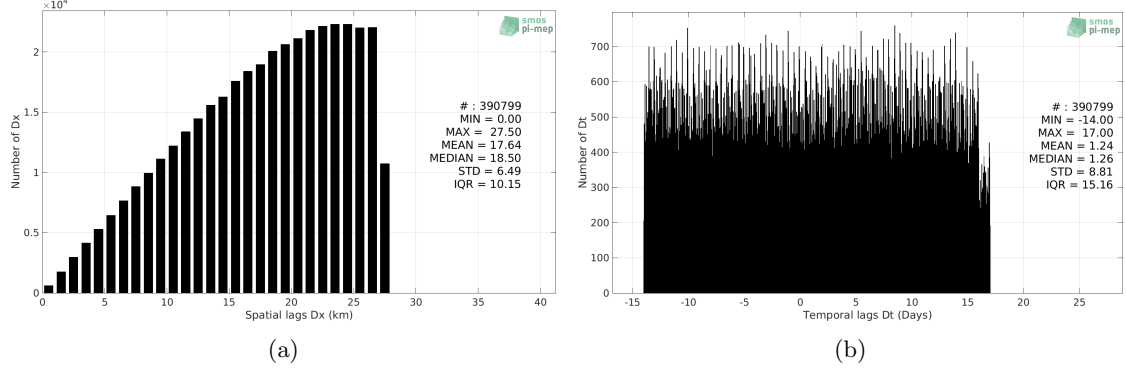
Figure 5: Histograms of the spatial (a) and temporal (b) lags between the time of the Argo measurements and the date of the corresponding Aquarius SSS L4 OI v5 - Monthly (IPRC) SSS product.
