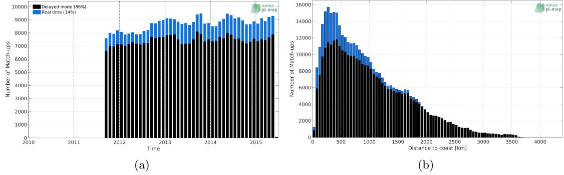
Figure 1: Number of match-ups between Argo and Aquarius SSS L4 OI v5 - Monthly (IPRC) SSS as a function of time (a) and as function of the distance to coast (b) over the Global Ocean Pi-MEP region and for the full satellite product period.
