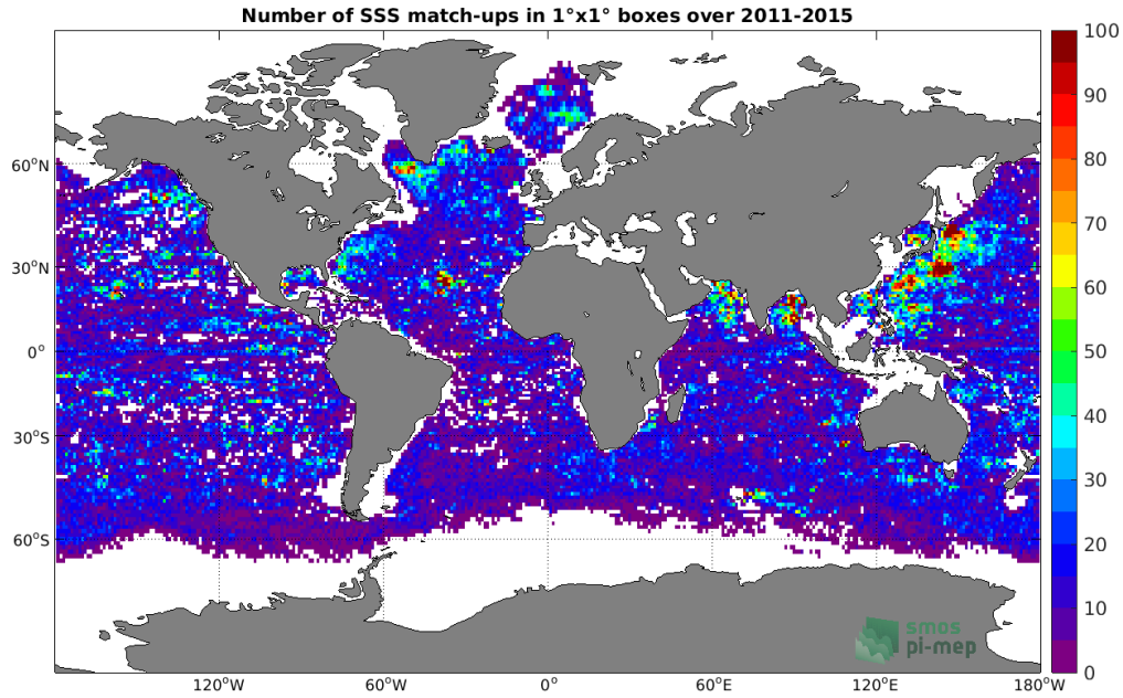
Figure 4: Number of SSS match-ups between Argos SSS and the Aquarius SSS L4 OI v5 - Monthly (IPRC) SSS product for the Global Ocean Pi-MEP region over 1^\circ \times 1^\circ boxes and for the full satellite product period.
