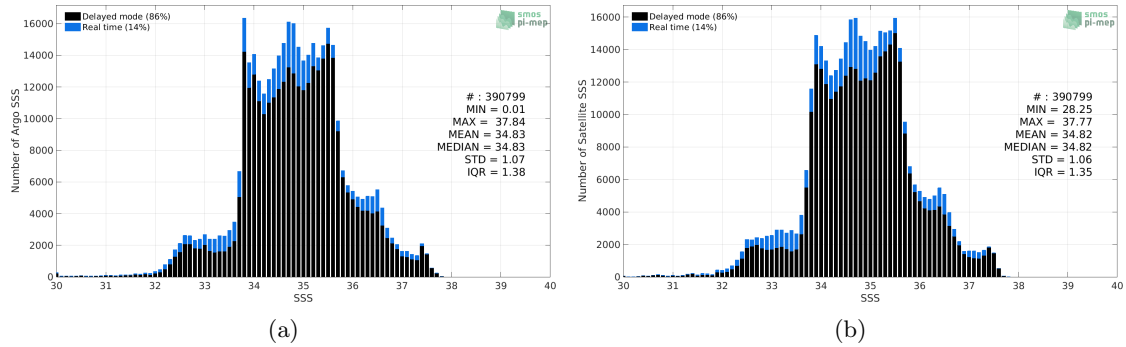
Figure 2: Histograms of SSS from Argo (a) and Aquarius SSS L4 OI v5 - Monthly (IPRC) (b) considering all match-up pairs per bins of 0.1 over the Global Ocean Pi-MEP region and for the full satellite product period.
