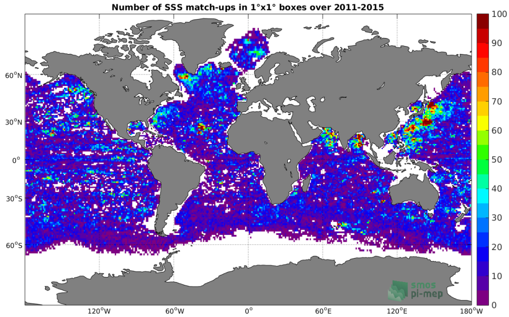
Figure 4: Number of SSS match-ups between Argo SSS and the Aquarius-L4-IPRC-V5-MONTHLY SSS product for the Global Ocean Pi-MEP region over 1^\circ \times 1^\circ boxes and for the full satellite product period.
