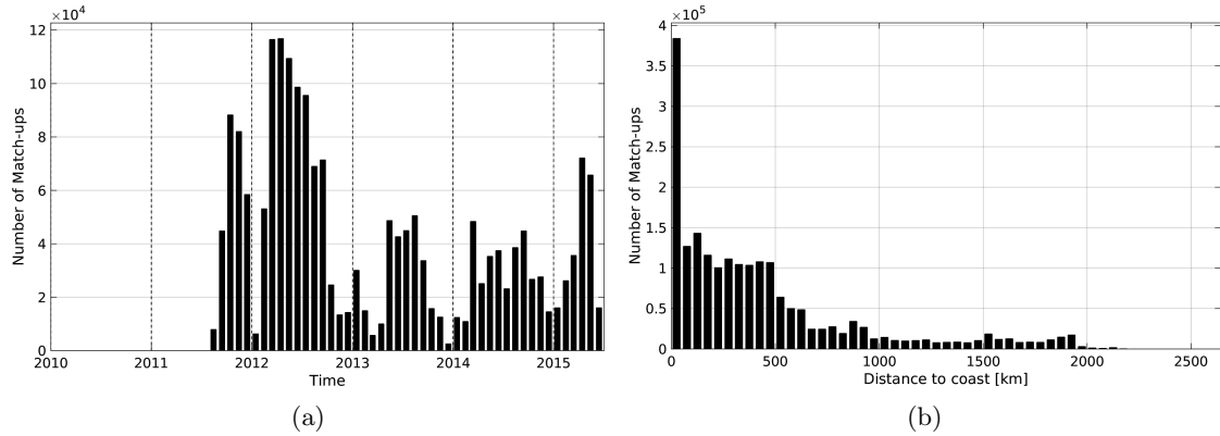
Figure 1: Number of match-ups between TSG-SAMOS and Aquarius-L4-IPRC-V4-WEEKLY SSS as a function of time (a) and as function of the distance to coast (b) over the Global Ocean Pi-MEP region and for the full satellite product period.
