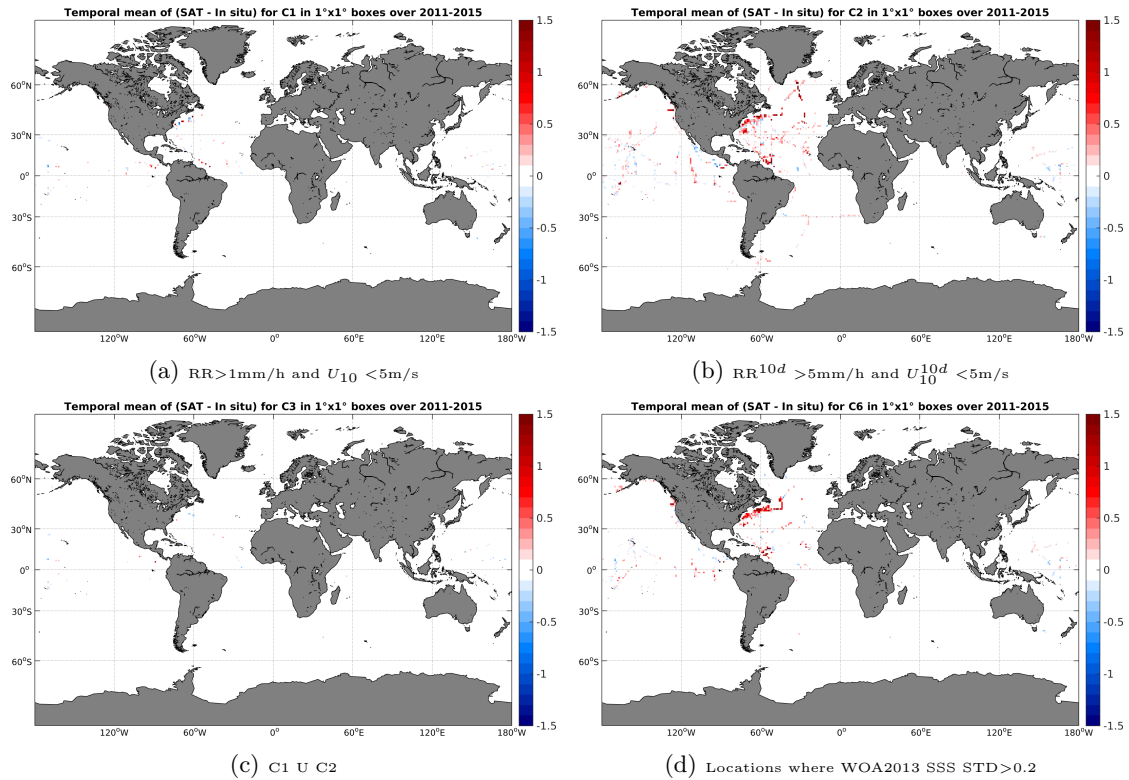
Figure 12: Temporal mean gridded over spatial boxes of size 1^\circ \times 1^\circ of \Delta SSS (Aquarius-L4-IPRC-V4-WEEKLY - TSG-SAMOS) for 4 different subdatasets corresponding to: RR > 1\text{mm/h} and U_{10} < 5\text{m/s} (a), RR^{10d} > 5\text{mm/h} and U_{10}^{10d} < 5\text{m/s} (b), C1 U C2 (c), Locations where WOA2013 SSS STD > 0.2 (d).
