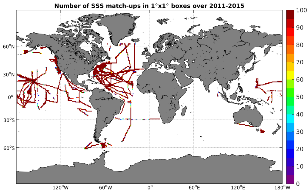
Figure 4: Number of SSS match-ups between TSG-SAMOS SSS and the Aquarius-L4-IPRC-V4-WEEKLY SSS product for the Global Ocean Pi-MEP region over 1^\circ \times 1^\circ boxes and for the full satellite product period.
