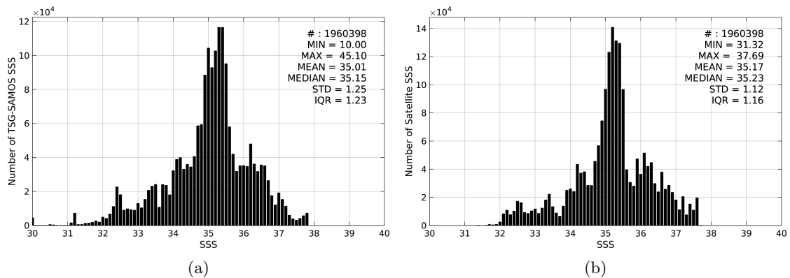
Figure 2: Histograms of SSS from TSG-SAMOS (a) and Aquarius-L4-IPRC-V4-WEEKLY (b) considering all match-up pairs per bins of 0.1 over the Global Ocean Pi-MEP region and for the full satellite product period.
