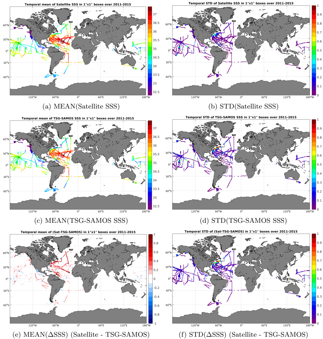
Figure 6: Temporal mean (left) and STD (right) of SSS from Aquarius-L4-IPRC-V4-WEEKLY (top), TSG-SAMOS (middle), and of \Delta SSS (Satellite - TSG-SAMOS). Only match-up pairs are used to generate these maps.
