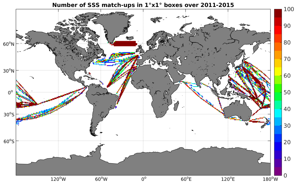
Figure 4: Number of SSS match-ups between TSG-LEGOS-DM SSS and the Aquarius-L4-IPRC-V4-WEEKLY SSS product for the Global Ocean Pi-MEP region over 1^\circ \times 1^\circ boxes and for the full satellite product period.
