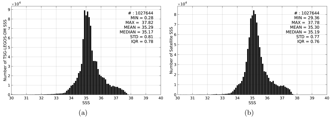
Figure 2: Histograms of SSS from TSG-LEGOS-DM (a) and Aquarius-L4-IPRC-V4-WEEKLY (b) considering all match-up pairs per bins of 0.1 over the Global Ocean Pi-MEP region and for the full satellite product period.
