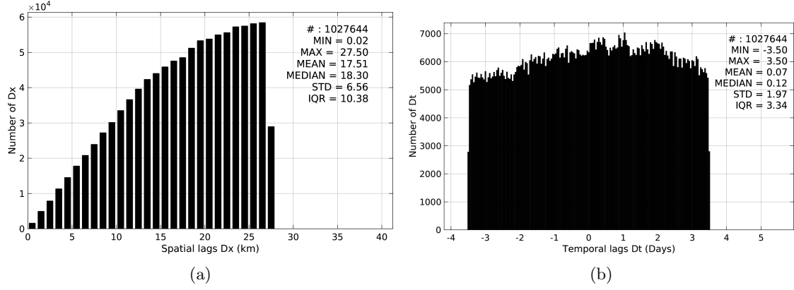
Figure 5: Histograms of the spatial (a) and temporal (b) lags between the time of the TSG-LEGOS-DM measurements and the date of the corresponding Aquarius-L4-IPRC-V4-WEEKLY SSS product.
