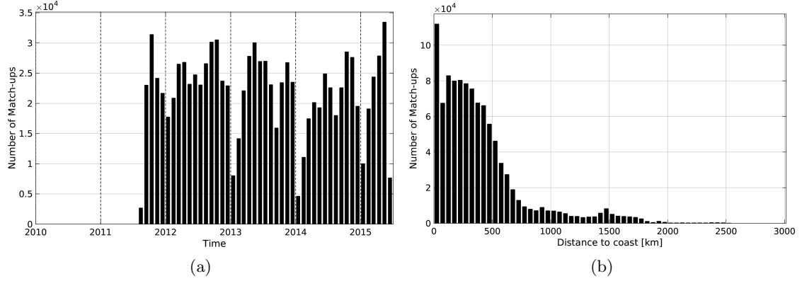
Figure 1: Number of match-ups between TSG-LEGOS-DM and Aquarius-L4-IPRC-V4-WEEKLY SSS as a function of time (a) and as function of the distance to coast (b) over the Global Ocean Pi-MEP region and for the full satellite product period.
