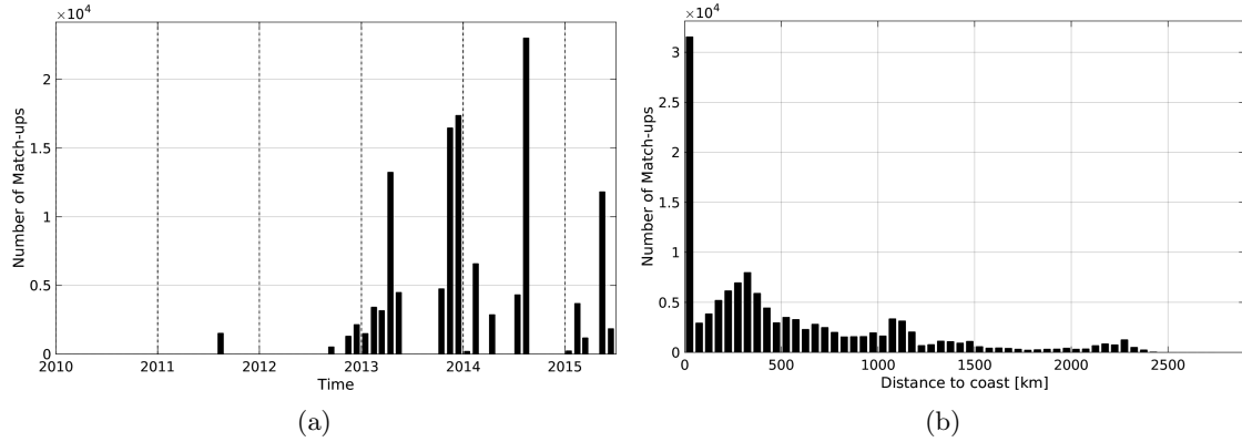
Figure 1: Number of match-ups between TSG-GOSUD-Sailing-ship and Aquarius-L4-IPRC-V4-WEEKLY SSS as a function of time (a) and as function of the distance to coast (b) over the Global Ocean Pi-MEP region and for the full satellite product period.
