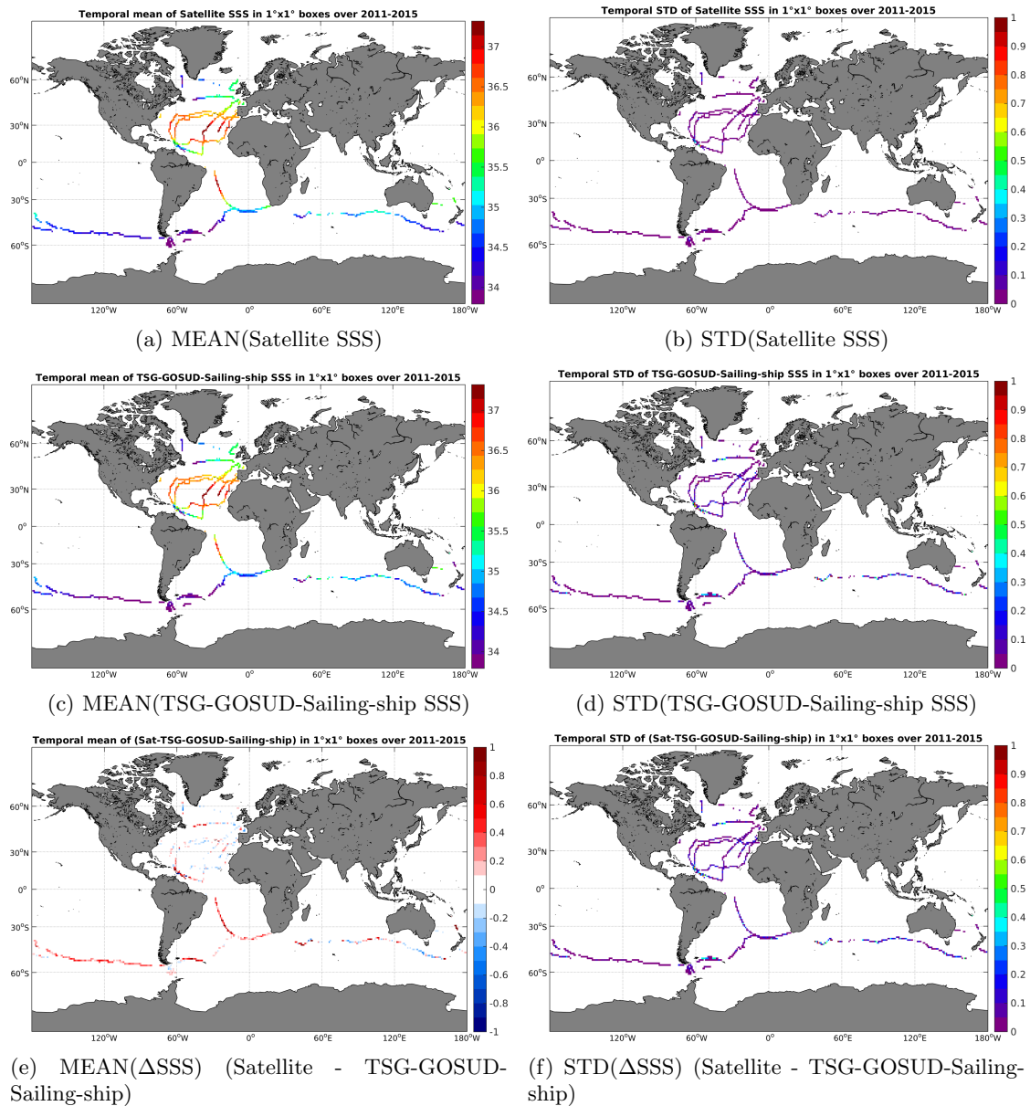
Figure 6: Temporal mean (left) and STD (right) of SSS from Aquarius-L4-IPRC-V4-WEEKLY (top), TSG-GOSUD-Sailing-ship (middle), and of \Delta SSS (Satellite - TSG-GOSUD-Sailing-ship). Only match-up pairs are used to generate these maps.
