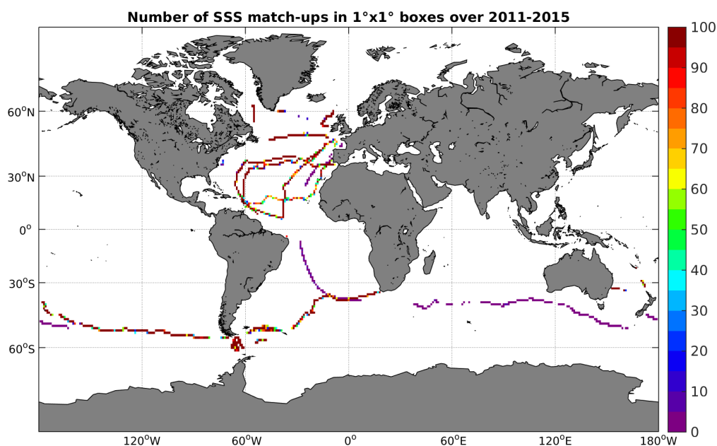
Figure 4: Number of SSS match-ups between TSG-GOSUD-Sailing-ship SSS and the Aquarius-L4-IPRC-V4-WEEKLY SSS product for the Global Ocean Pi-MEP region over 1°x1° boxes and for the full satellite product period.
