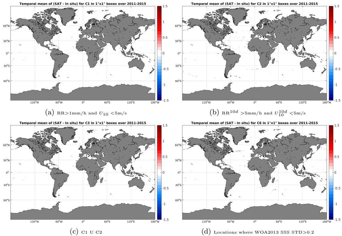
Figure 12: Temporal mean gridded over spatial boxes of size 1^\circ \times 1^\circ of \Delta SSS (Aquarius-L4-IPRC-V4-WEEKLY - TSG-GOSUD-Sailing-ship) for 4 different subdatasets corresponding to: RR > 1mm/h and U_{10} < 5\text{m/s} (a), RR^{10d} > 5\text{mm/h} and U_{10}^{10d} < 5\text{m/s} (b), C1 U C2 (c), Locations where WOA2013 SSS STD > 0.2 (d).
