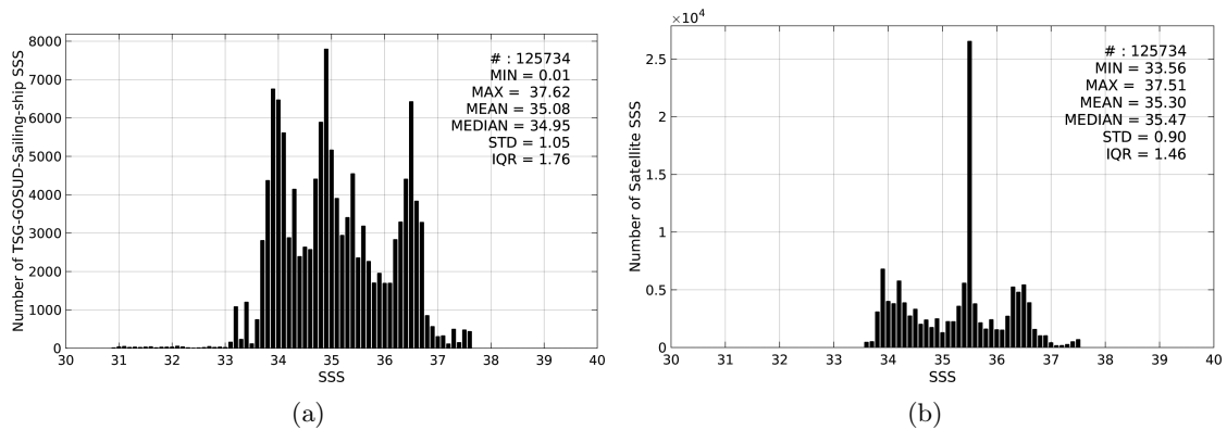
Figure 2: Histograms of SSS from TSG-GOSUD-Sailing-ship (a) and Aquarius-L4-IPRC-V4-WEEKLY (b) considering all match-up pairs per bins of 0.1 over the Global Ocean Pi-MEP region and for the full satellite product period.
