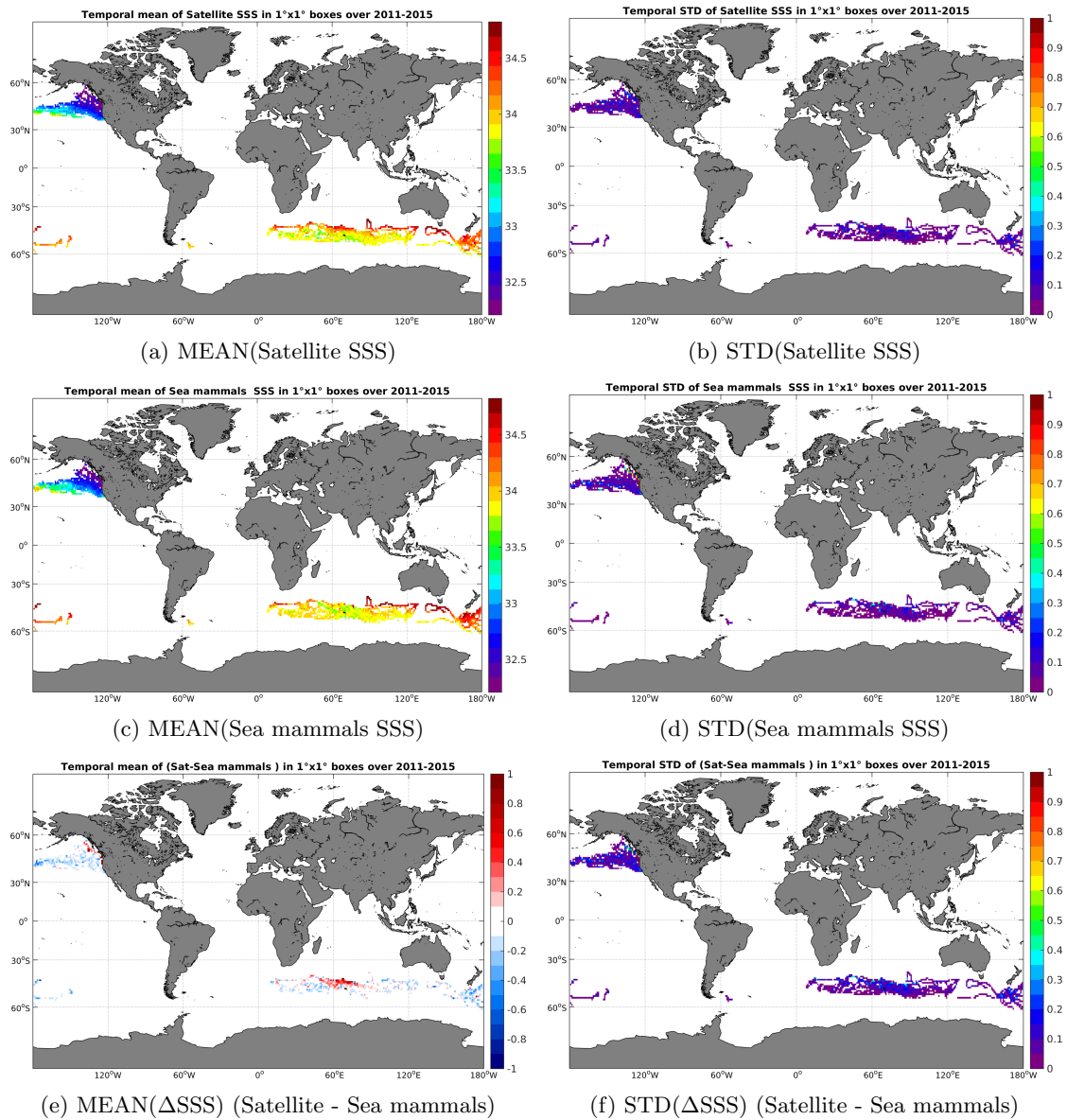
Figure 6: Temporal mean (left) and STD (right) of SSS from Aquarius-L4-IPRC-V4-WEEKLY (top), Sea mammals (middle), and of \Delta SSS (Satellite - Sea mammals). Only match-up pairs are used to generate these maps.
