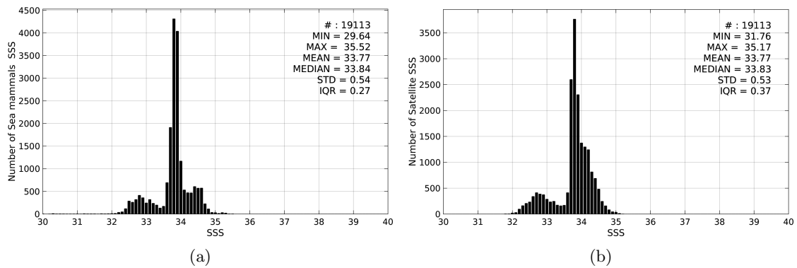
Figure 2: Histograms of SSS from Sea mammals (a) and Aquarius-L4-IPRC-V4-WEEKLY (b) considering all match-up pairs per bins of 0.1 over the Global Ocean Pi-MEP region and for the full satellite product period.
