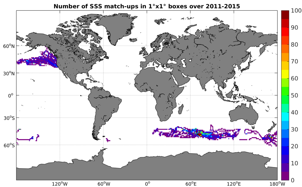
Figure 4: Number of SSS match-ups between Sea mammals SSS and the Aquarius-L4-IPRC-V4-WEEKLY SSS product for the Global Ocean Pi-MEP region over 1^\circ \times 1^\circ boxes and for the full satellite product period.
