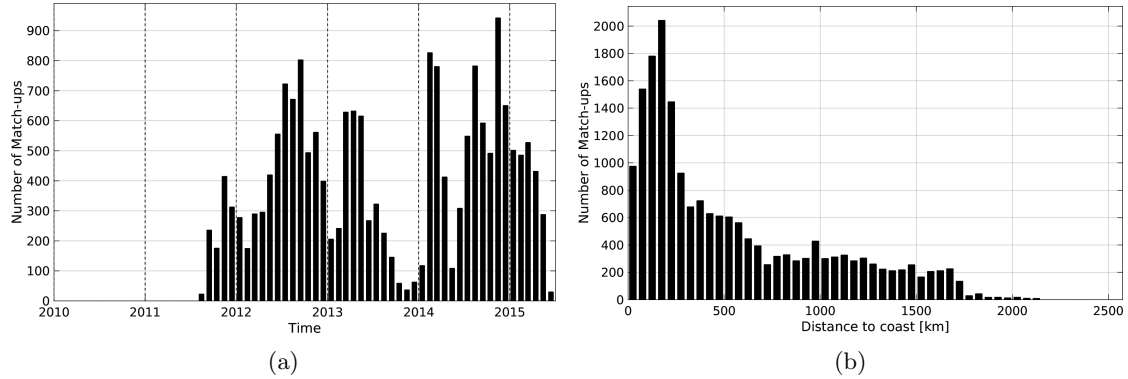
Figure 1: Number of match-ups between Sea mammals and Aquarius-L4-IPRC-V4-WEEKLY SSS as a function of time (a) and as function of the distance to coast (b) over the Global Ocean Pi-MEP region and for the full satellite product period.
