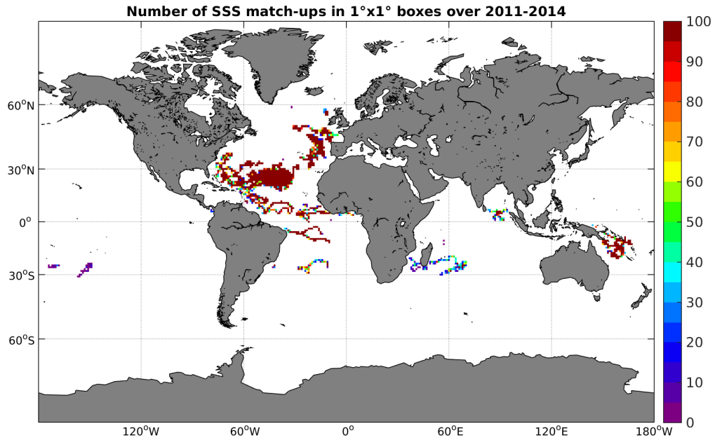
Figure 3: Number of SSS match-ups between Surface drifters SSS and the Aquarius-L4-IPRC-V4-WEEKLY SSS product for the Global Ocean Pi-MEP region over 1^\circ \times 1^\circ boxes and for the full satellite product period.
