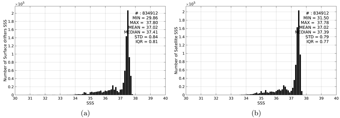
Figure 2: Histograms of SSS from Surface drifters (a) and Aquarius-L4-IPRC-V4-WEEKLY (b) considering all match-up pairs per bins of 0.1 over the Global Ocean Pi-MEP region and for the full satellite product period.
