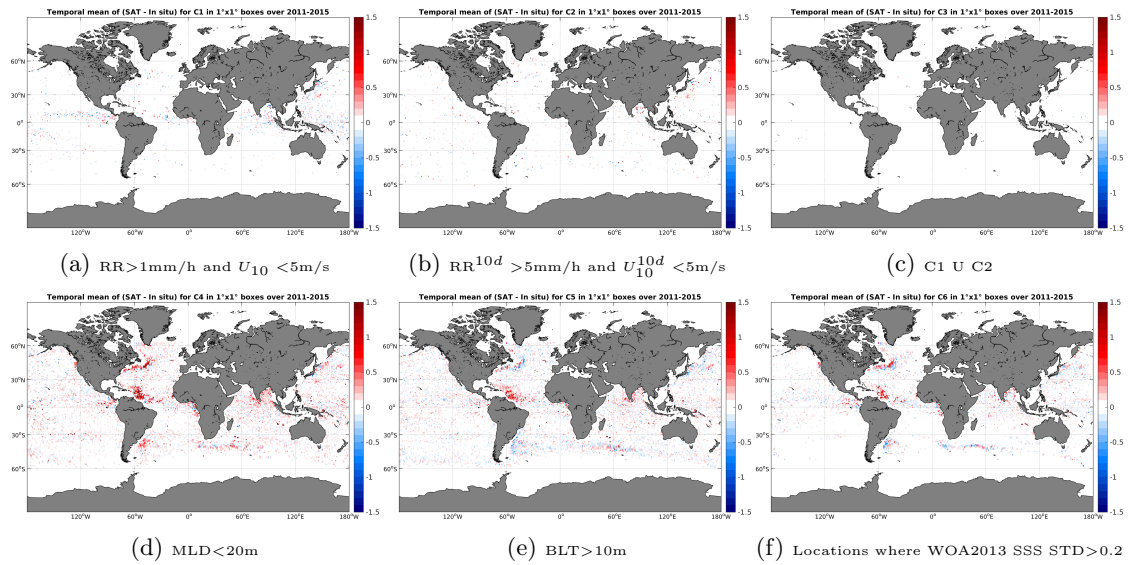
Figure 12: Temporal mean gridded over spatial boxes of size 1^\circ \times 1^\circ of \Delta SSS (Aquarius-L4-IPRC-V4-WEEKLY - Argo) for 6 different subdatasets corresponding to: RR>1mm/h and U_{10} < 5\text{m/s} (a), RR^{10d} > 5\text{mm/h} and U_{10}^{10d} < 5\text{m/s} (b), C1 U C2 (c), MLD<20m (d), BLT>10m (e), Locations where WOA2013 SSS STD>0.2 (f).
