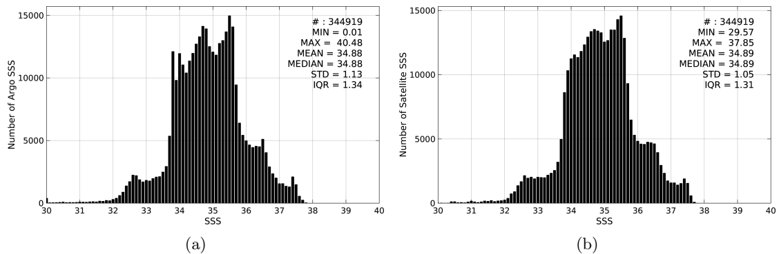
Figure 2: Histograms of SSS from Argo (a) and Aquarius-L4-IPRC-V4-WEEKLY (b) considering all match-up pairs per bins of 0.1 over the Global Ocean Pi-MEP region and for the full satellite product period.
