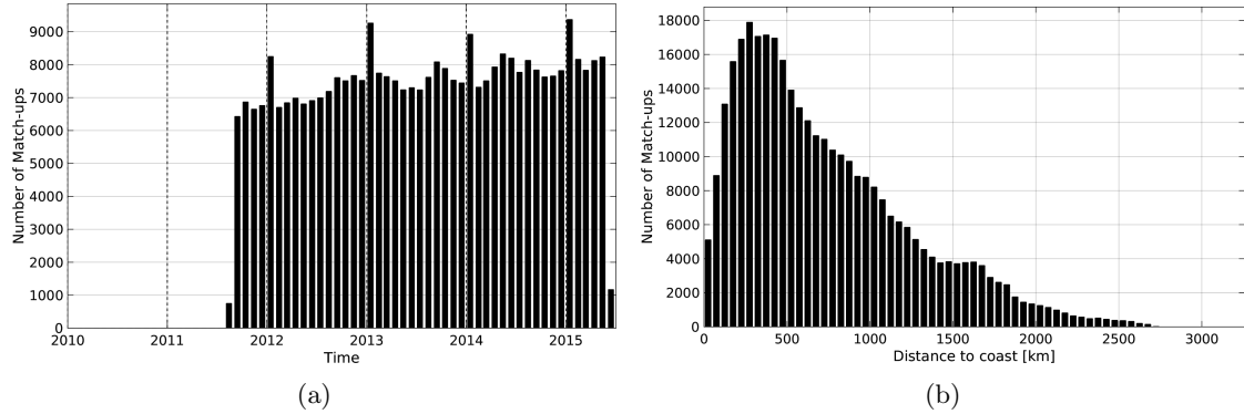
Figure 1: Number of match-ups between Argo and Aquarius-L4-IPRC-V4-WEEKLY SSS as a function of time (a) and as function of the distance to coast (b) over the Global Ocean Pi-MEP region and for the full satellite product period.
