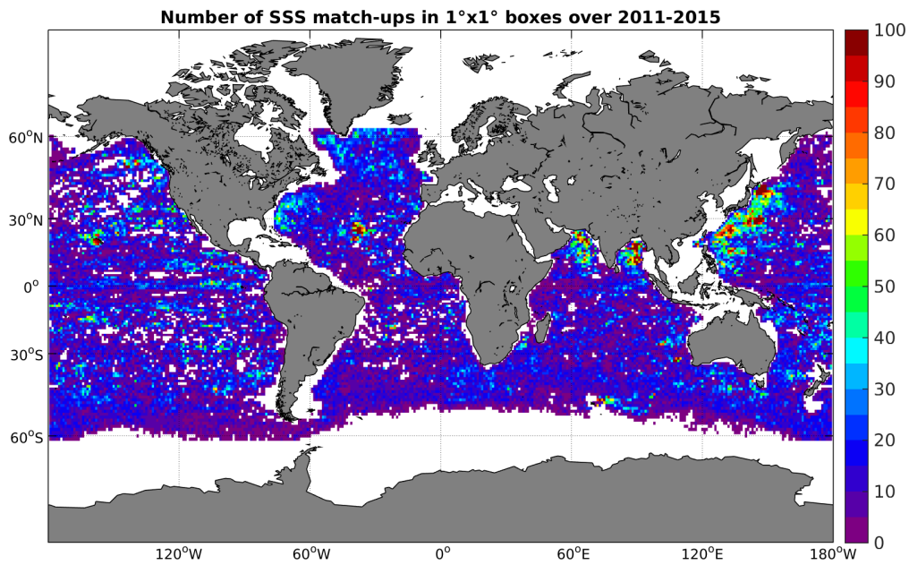
Figure 4: Number of SSS match-ups between Argo SSS and the Aquarius-L4-IPRC-V4-WEEKLY SSS product for the Global Ocean Pi-MEP region over 1^\circ \times 1^\circ boxes and for the full satellite product period.
