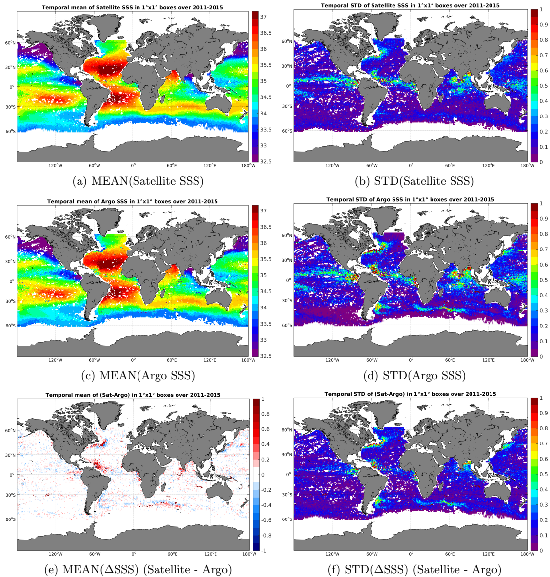
Figure 6: Temporal mean (left) and STD (right) of SSS from Aquarius-L4-IPRC-V4-WEEKLY (top), Argo (middle), and of \Delta SSS (Satellite - Argo). Only match-up pairs are used to generate these maps.
