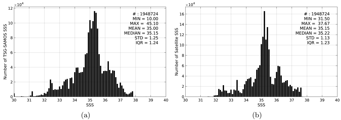
Figure 2: Histograms of SSS from TSG-SAMOS (a) and Aquarius-L4-IPRC-V4-MONTHLY (b) considering all match-up pairs per bins of 0.1 over the Global Ocean Pi-MEP region and for the full satellite product period.
