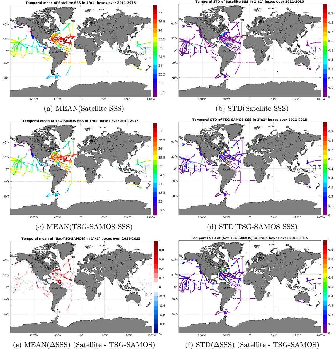
Figure 6: Temporal mean (left) and STD (right) of SSS from Aquarius-L4-IPRC-V4-MONTHLY (top), TSG-SAMOS (middle), and of \Delta SSS (Satellite - TSG-SAMOS). Only match-up pairs are used to generate these maps.
