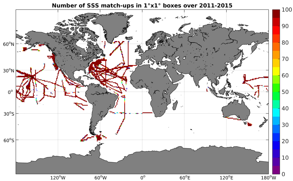
Figure 4: Number of SSS match-ups between TSG-SAMOS SSS and the Aquarius-L4-IPRC-V4-MONTHLY SSS product for the Global Ocean Pi-MEP region over 1^\circ \times 1^\circ boxes and for the full satellite product period.
