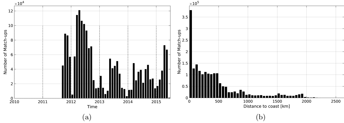
Figure 1: Number of match-ups between TSG-SAMOS and Aquarius-L4-IPRC-V4-MONTHLY SSS as a function of time (a) and as function of the distance to coast (b) over the Global Ocean Pi-MEP region and for the full satellite product period.
