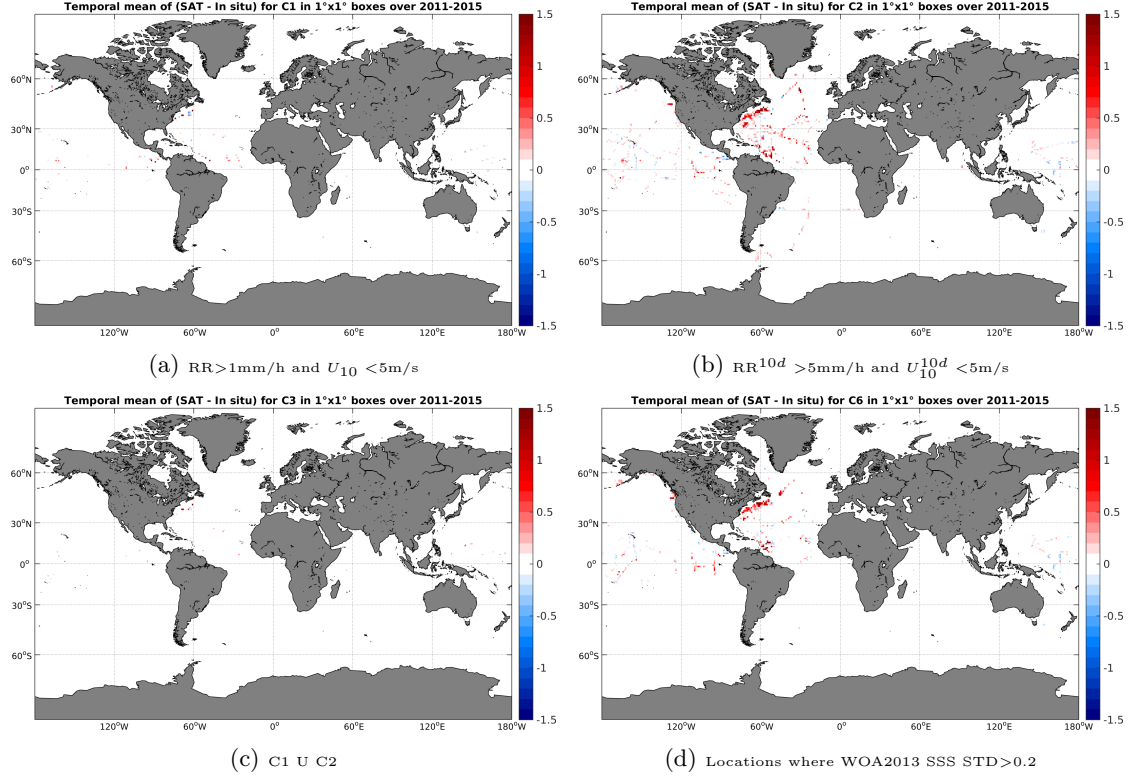
Figure 12: Temporal mean gridded over spatial boxes of size 1^\circ \times 1^\circ of \Delta SSS (Aquarius-L4-IPRC-V4-MONTHLY - TSG-SAMOS) for 4 different subdatasets corresponding to: RR > 1\text{mm/h} and U_{10} < 5\text{m/s} (a), RR^{10d} > 5\text{mm/h} and U_{10}^{10d} < 5\text{m/s} (b), C1 U C2 (c), Locations where WOA2013 SSS STD > 0.2 (d).
