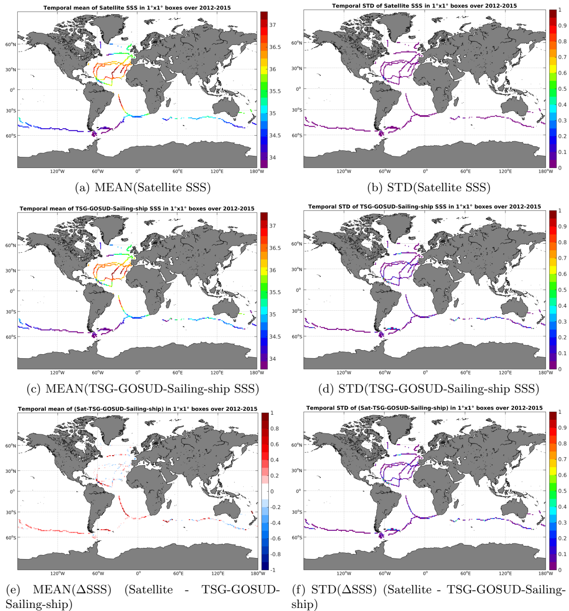
Figure 6: Temporal mean (left) and STD (right) of SSS from Aquarius-L4-IPRC-V4-MONTHLY (top), TSG-GOSUD-Sailing-ship (middle), and of \Delta SSS (Satellite - TSG-GOSUD-Sailing-ship). Only match-up pairs are used to generate these maps.
