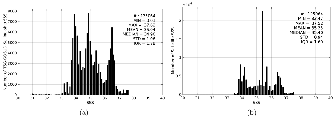
Figure 2: Histograms of SSS from TSG-GOSUD-Sailing-ship (a) and Aquarius-L4-IPRC-V4-MONTHLY (b) considering all match-up pairs per bins of 0.1 over the Global Ocean Pi-MEP region and for the full satellite product period.
