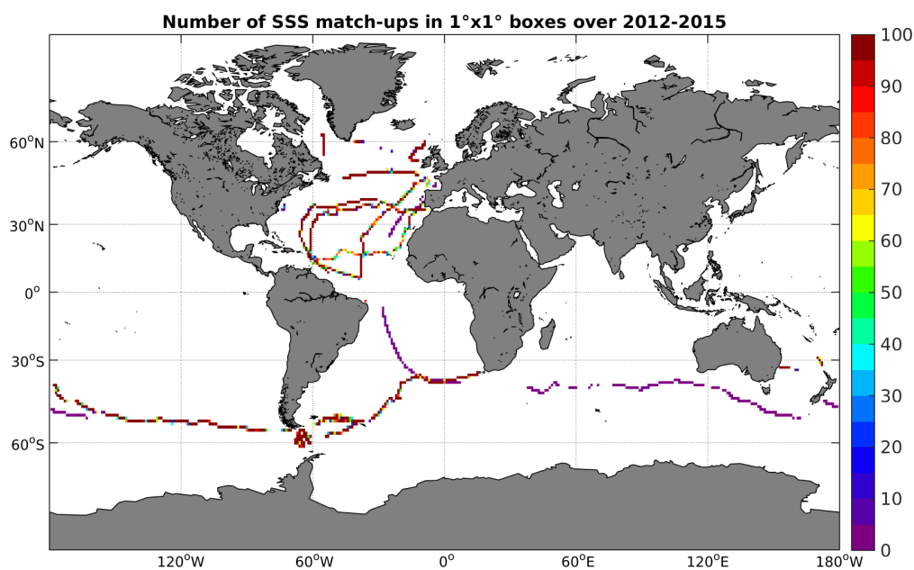
Figure 4: Number of SSS match-ups between TSG-GOSUD-Sailing-ship SSS and the Aquarius-L4-IPRC-V4-MONTHLY SSS product for the Global Ocean Pi-MEP region over 1°x1° boxes and for the full satellite product period.
