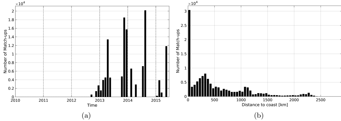
Figure 1: Number of match-ups between TSG-GOSUD-Sailing-ship and Aquarius-L4-IPRC-V4-MONTHLY SSS as a function of time (a) and as function of the distance to coast (b) over the Global Ocean Pi-MEP region and for the full satellite product period.
