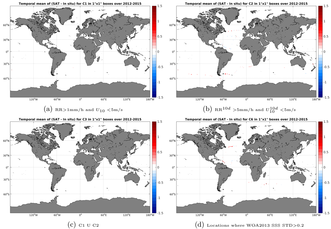
Figure 12: Temporal mean gridded over spatial boxes of size 1°x1° of \Delta SSS (Aquarius-L4-IPRC-V4-MONTHLY - TSG-GOSUD-Sailing-ship) for 4 different subdatasets corresponding to:RR>1mm/h and U_{10} < 5m/s (a), RR^{10d} > 5mm/h and U_{10}^{10d} < 5m/s (b), C1 U C2 (c),Locations where WOA2013 SSS STD>0.2 (d).
