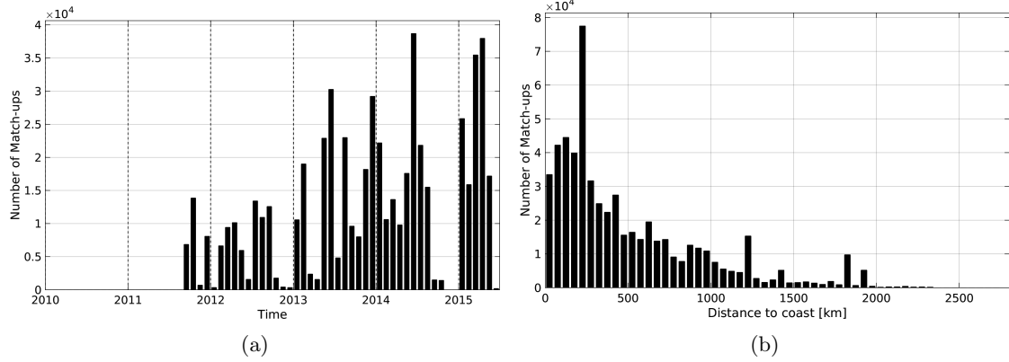
Figure 1: Number of match-ups between TSG-GOSUD-Research-vessel and Aquarius-L4-IPRC-V4-MONTHLY SSS as a function of time (a) and as function of the distance to coast (b) over the Global Ocean Pi-MEP region and for the full satellite product period.
