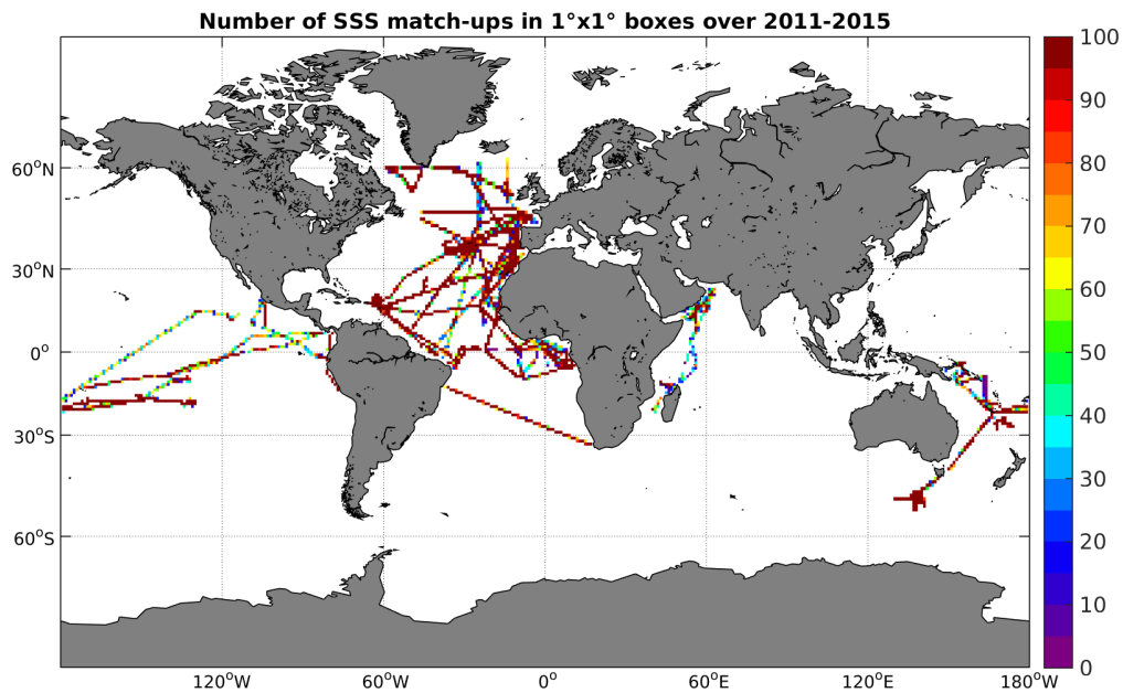
Figure 4: Number of SSS match-ups between TSG-GOSUD-Research-vessel SSS and the Aquarius-L4-IPRC-V4-MONTHLY SSS product for the Global Ocean Pi-MEP region over 1^\circ \times 1^\circ boxes and for the full satellite product period.
