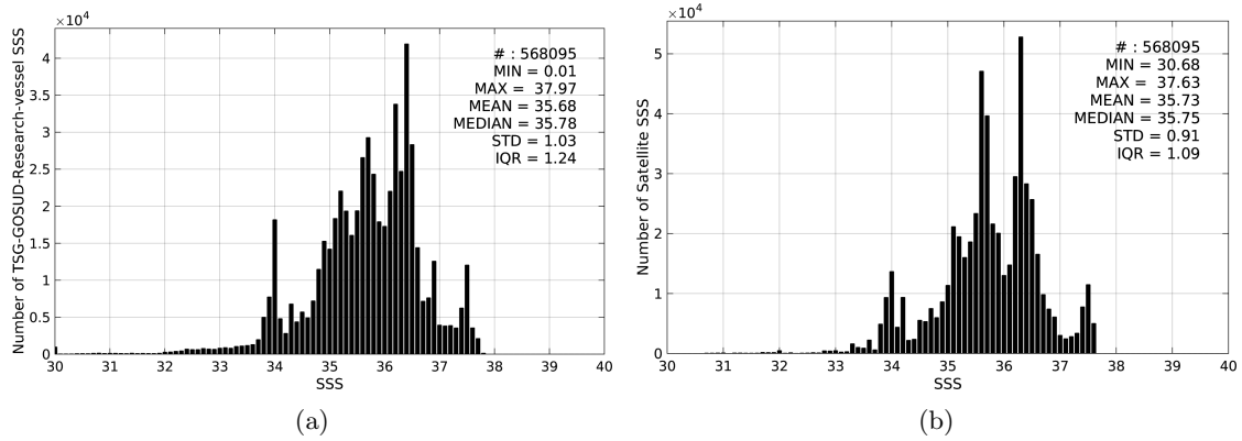
Figure 2: Histograms of SSS from TSG-GOSUD-Research-vessel (a) and Aquarius-L4-IPRC-V4-MONTHLY (b) considering all match-up pairs per bins of 0.1 over the Global Ocean Pi-MEP region and for the full satellite product period.
