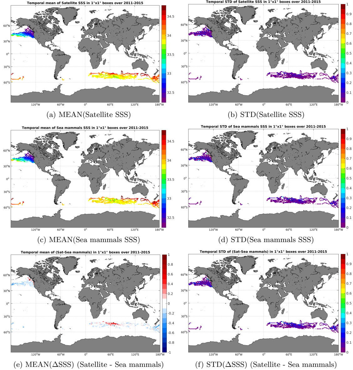
Figure 6: Temporal mean (left) and STD (right) of SSS from Aquarius-L4-IPRC-V4-MONTHLY (top), Sea mammals (middle), and of \Delta SSS (Satellite - Sea mammals). Only match-up pairs are used to generate these maps.
