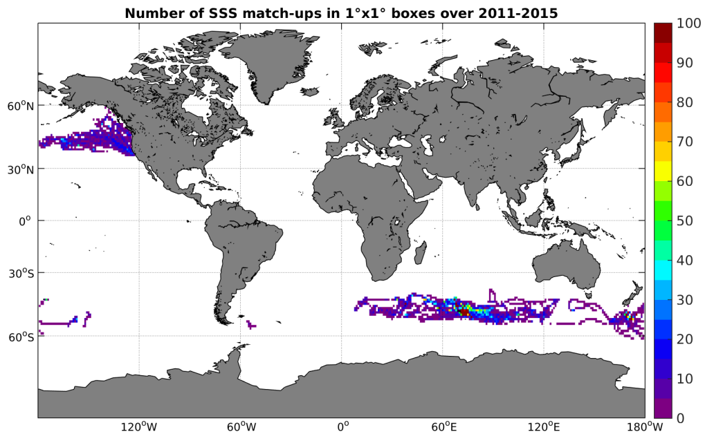
Figure 4: Number of SSS match-ups between Sea mammals SSS and the Aquarius-L4-IPRC-V4-MONTHLY SSS product for the Global Ocean Pi-MEP region over 1^\circ \times 1^\circ boxes and for the full satellite product period.
