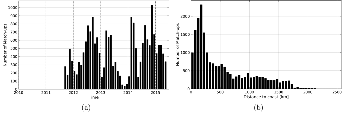
Figure 1: Number of match-ups between Sea mammals and Aquarius-L4-IPRC-V4-MONTHLY SSS as a function of time (a) and as function of the distance to coast (b) over the Global Ocean Pi-MEP region and for the full satellite product period.
