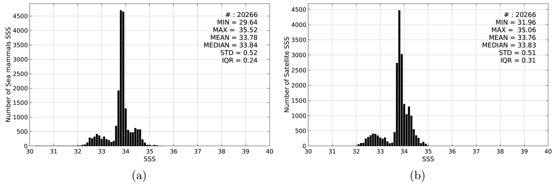
Figure 2: Histograms of SSS from Sea mammals (a) and Aquarius-L4-IPRC-V4-MONTHLY (b) considering all match-up pairs per bins of 0.1 over the Global Ocean Pi-MEP region and for the full satellite product period.
