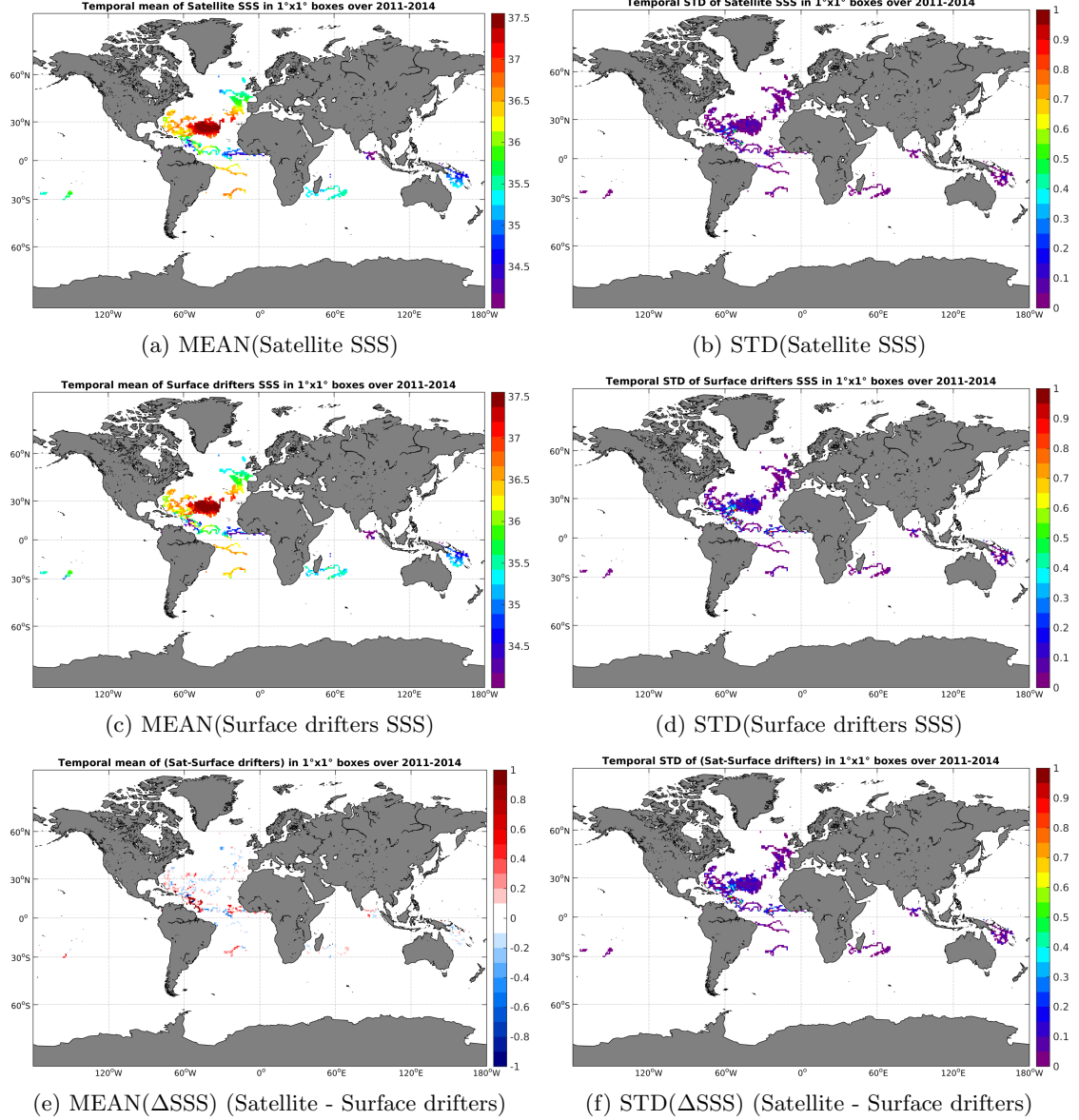
Figure 5: Temporal mean (left) and STD (right) of SSS from Aquarius-L4-IPRC-V4-MONTHLY (top), Surface drifters (middle), and of \Delta SSS (Satellite - Surface drifters). Only match-up pairs are used to generate these maps.
