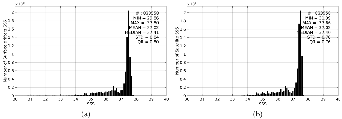
Figure 2: Histograms of SSS from Surface drifters (a) and Aquarius-L4-IPRC-V4-MONTHLY (b) considering all match-up pairs per bins of 0.1 over the Global Ocean Pi-MEP region and for the full satellite product period.
