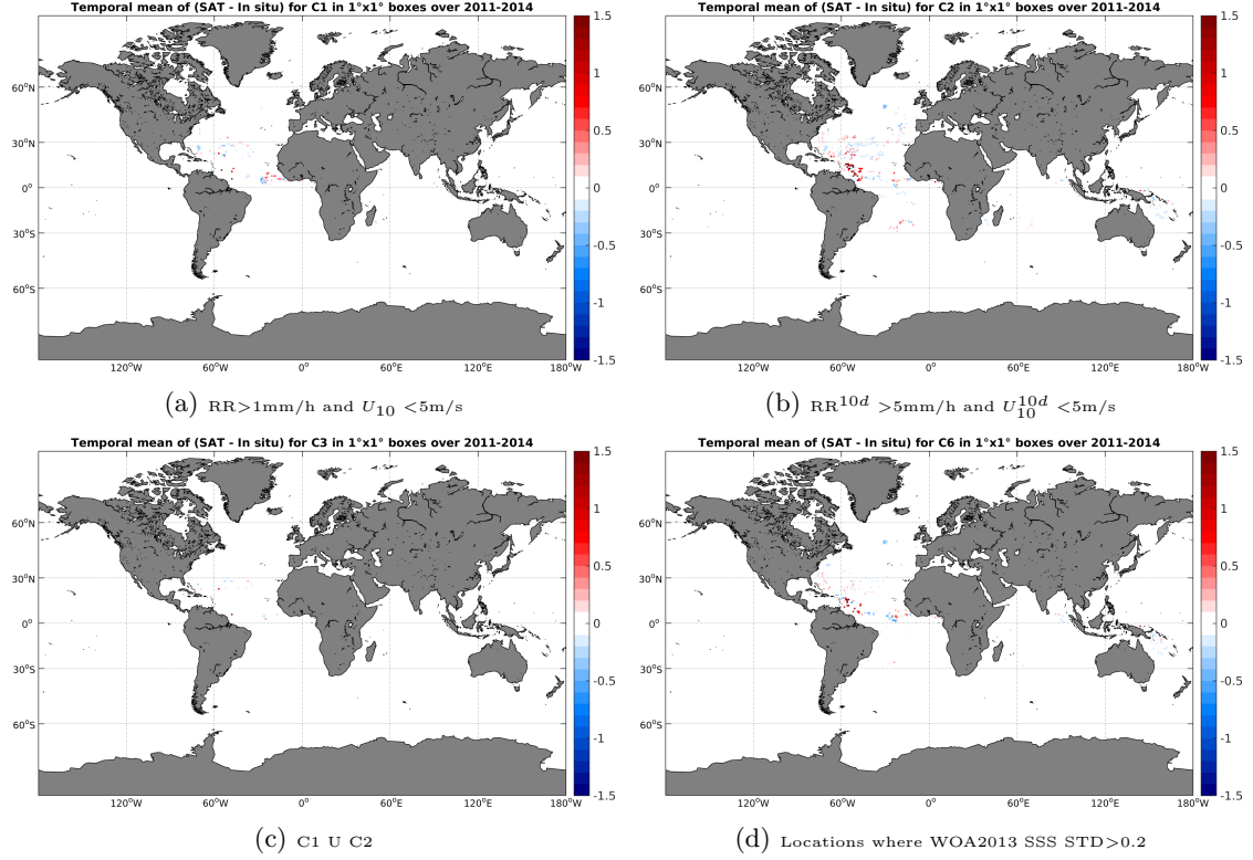
Figure 11: Temporal mean gridded over spatial boxes of size 1^\circ \times 1^\circ of \Delta SSS (Aquarius-L4-IPRC-V4-MONTHLY - Surface drifters) for 4 different subdatasets corresponding to: RR > 1\text{mm/h} and U_{10} < 5\text{m/s} (a), RR^{10d} > 5\text{mm/h} and U_{10}^{10d} < 5\text{m/s} (b), C1 U C2 (c), Locations where WOA2013 SSS STD > 0.2 (d).
