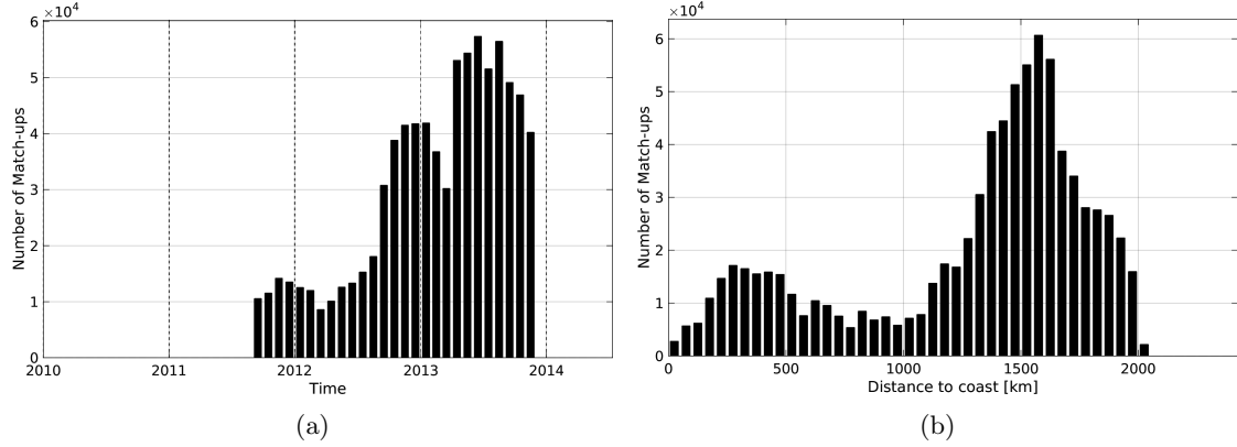
Figure 1: Number of match-ups between Surface drifters and Aquarius-L4-IPRC-V4-MONTHLY SSS as a function of time (a) and as function of the distance to coast (b) over the Global Ocean Pi-MEP region and for the full satellite product period.
