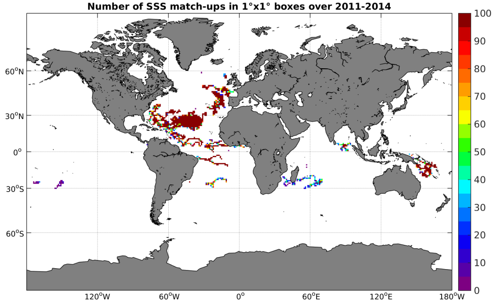
Figure 3: Number of SSS match-ups between Surface drifters SSS and the Aquarius-L4-IPRC-V4-MONTHLY SSS product for the Global Ocean Pi-MEP region over 1°x1° boxes and for the full satellite product period.
