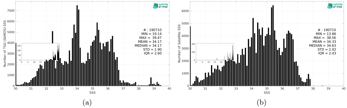
Figure 3: Histograms of SSS from TSG (SAMOS) (a) and Aquarius SSS L3 OR v5 - 7-Day running (NASA-GSFC) (b) considering all match-up pairs per bins of 0.1 over the Global Ocean Pi-MEP region and for the full satellite product period.
