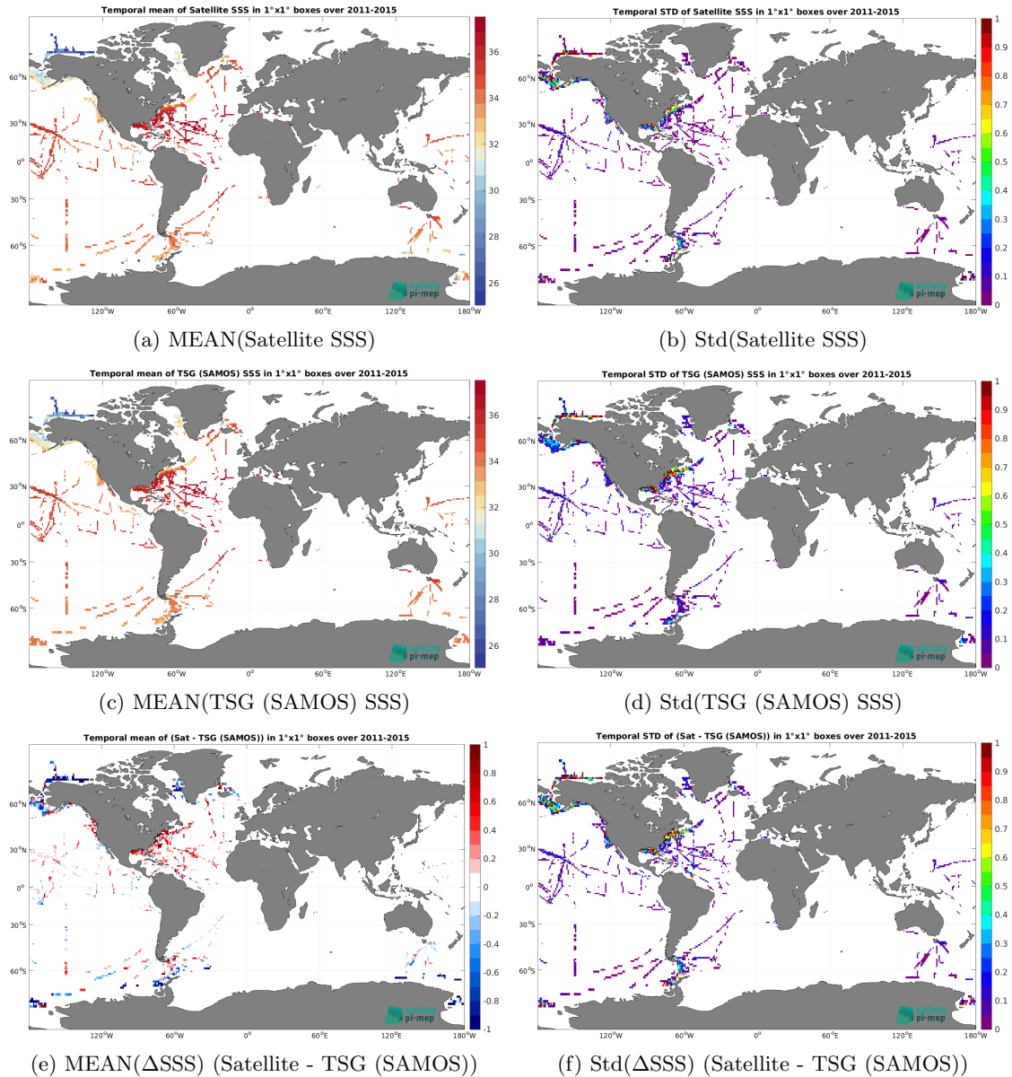
Figure 7: Temporal mean (left) and Std (right) of SSS from Aquarius SSS L3 OR v5 - 7-Day running (NASA-GSFC) (top), TSG (SAMOS) (middle), and of \Delta SSS (Satellite - TSG (SAMOS)). Only match-up pairs are used to generate these maps.
