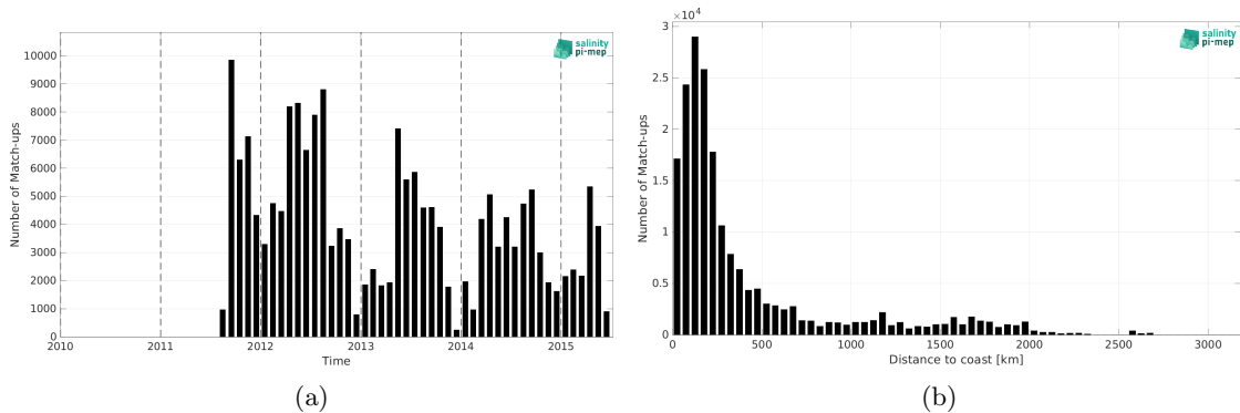
Figure 2: Number of match-ups between TSG (SAMOS) and Aquarius SSS L3 OR v5 - 7-Day running (NASA-GSFC) SSS as a function of time (a) and as function of the distance to coast (b) over the Global Ocean Pi-MEP region and for the full satellite product period.
