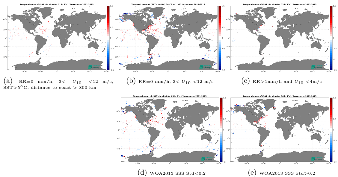
Figure 14: Temporal mean gridded over spatial boxes of size 1^\circ \times 1^\circ of \Delta SSS (Aquarius SSS L3 OR v5 - 7-Day running (NASA-GSFC) - TSG (SAMOS)) for 5 different subdatasets corresponding to:RR=0 mm/h, 3 < U_{10} < 12 m/s, SST > 5^\circ\text{C} , distance to coast > 800 km (a), RR=0 mm/h, 3 < U_{10} < 12 m/s (b), RR > 1 mm/h and U_{10} < 4 m/s (c), WOA2013 SSS Std < 0.2 (d), WOA2013 SSS Std > 0.2 (e).
