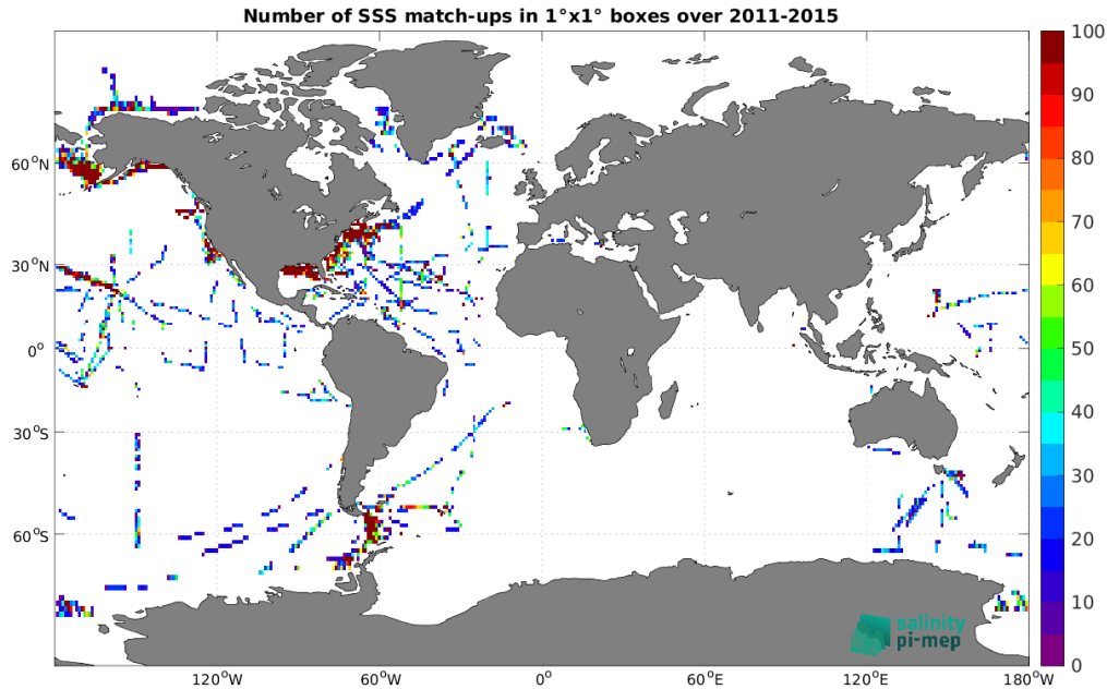
Figure 5: Number of SSS match-ups between TSG (SAMOS) SSS and the Aquarius SSS L3 OR v5 - 7-Day running (NASA-GSFC) SSS product for the Global Ocean Pi-MEP region over 1^\circ \times 1^\circ boxes and for the full satellite product period.
